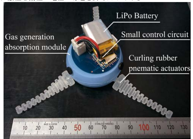
Fig.2 Appearance of the untethered pneumatic robot
