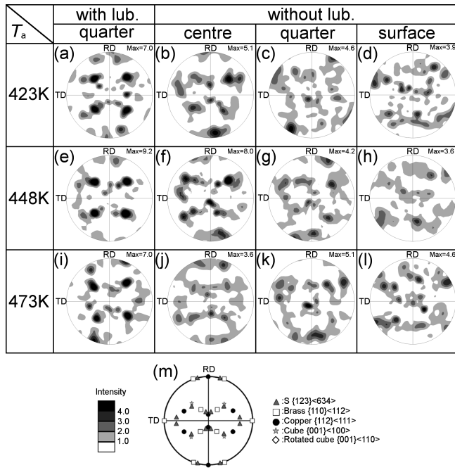
Fig. 10 {111} pole figures of ARB processed 4N-Cu: (a)–(d) are ARB 6c annealed at 423 K, (e)–(h) are ARB 6c annealed at 448 K and (i)–(l) are ARB 6c annealed at 473 K. The first column from the left is the results at quarter of ARB with lubrication. The second, third, and the fourth columns from the left are at centre, quarter, and surface of ARB without lubrication, respectively. (m) ideal orientations of the rolling texture along \beta fibre, Cube and rotated Cube orientations.
