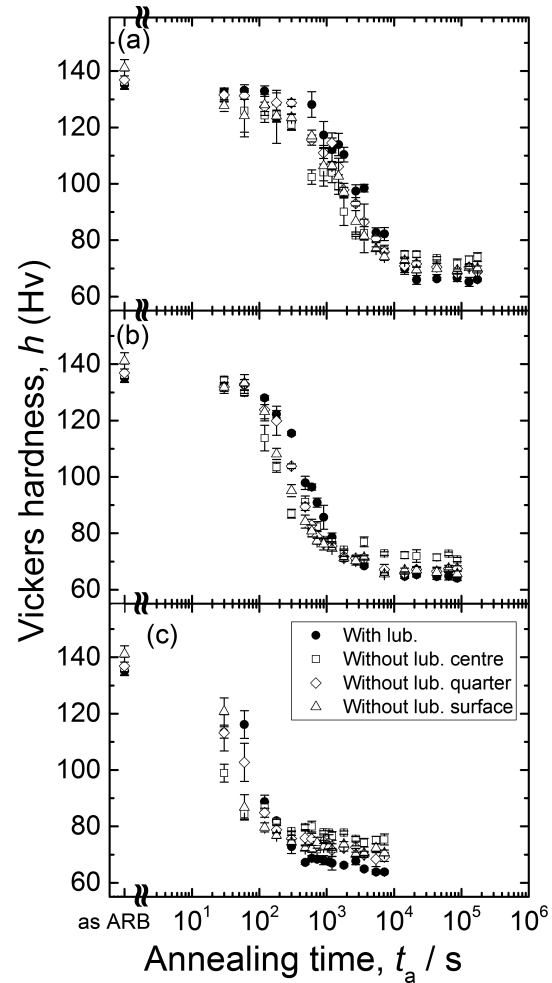
Fig. 9 Annealing time dependence on Vickers hardness of ARB 6c with and without lubrication of which annealing temperature at (a) 423 K, (b) 448 K and (c) 473 K.
