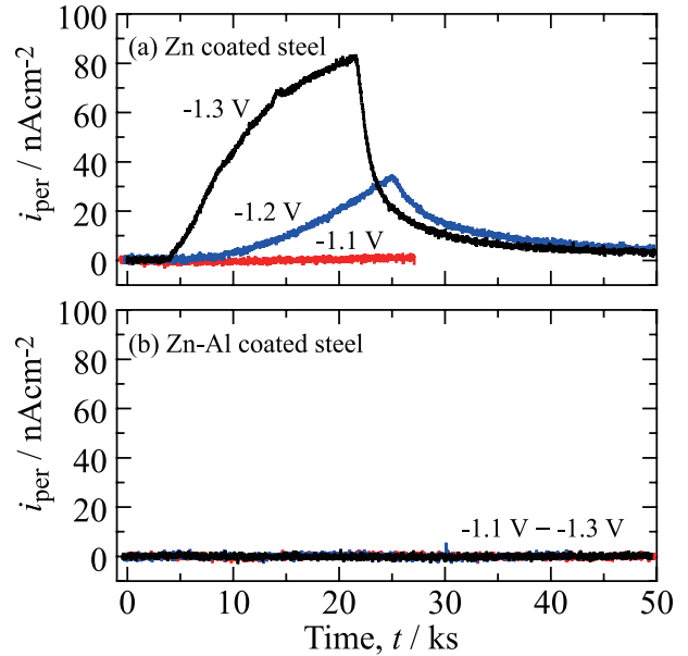
Fig. 7. Changes in hydrogen permeation currents for Zn coated steels and Zn-Al coated steels in NaCl solution at various polarization potentials. (Online version in color.)
