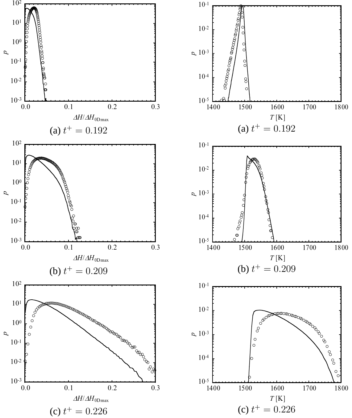
Figure 5.15: PDF of heat release rate (left) and temperature (right) at droplet position. Solid lines represent PDF of whole flow field.
