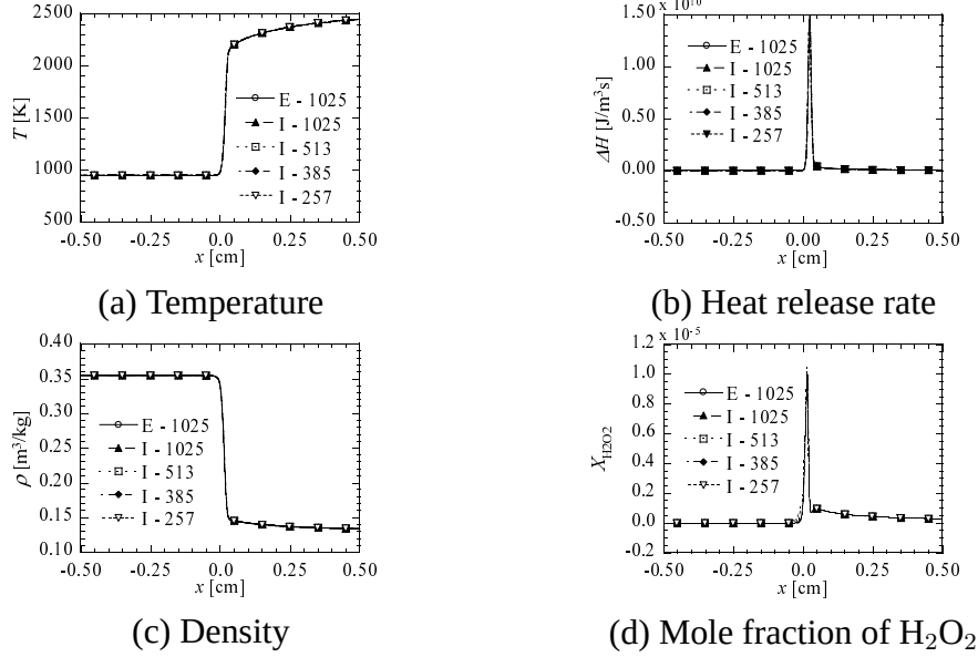
Figure B.3: Spatial distributions of temperature, heat release rate, density and mole fraction of H 2 O 2 of methane/air premixed flame for different grid point cases.
