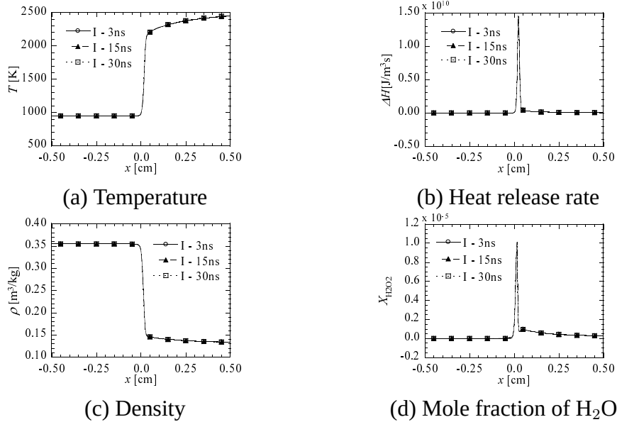
Figure B.4: Spatial distributions of temperature, heat release rate, density and mole fraction of H 2 O 2 of methane/air premixed flame for different time increment cases.
