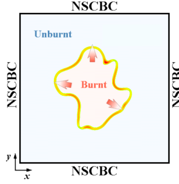
Figure 4.1: Geometry of the flow field.
