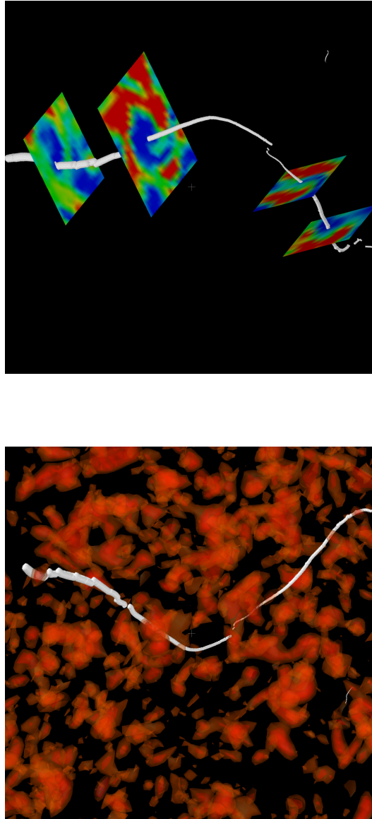
Figure 5.22: Distribution and isosurface of temperature around an axis of the coherent fine scale eddy
