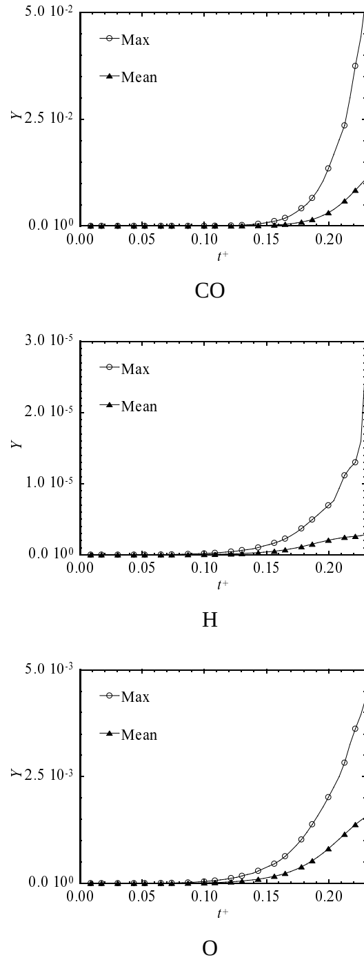
Figure 5.5: Temporal developments of mass fraction of major species.
