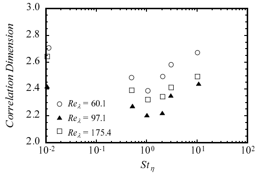
Figure 2.27: Nonuniformity of particle distribution based on correlation dimension.
