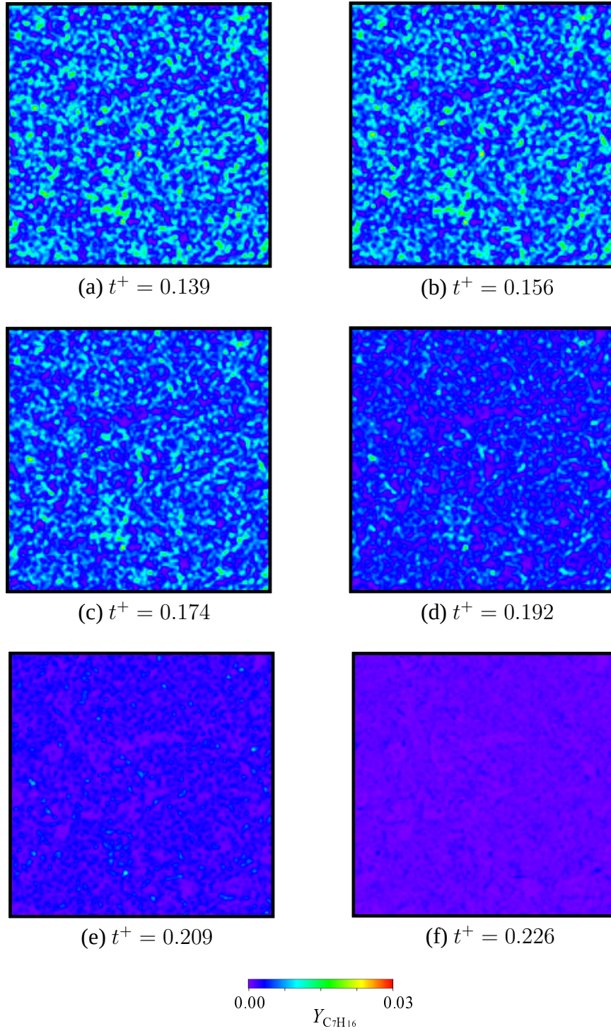
Figure 5.9: Temporal developments of distributions of mass fraction of C_7H_{16} .
