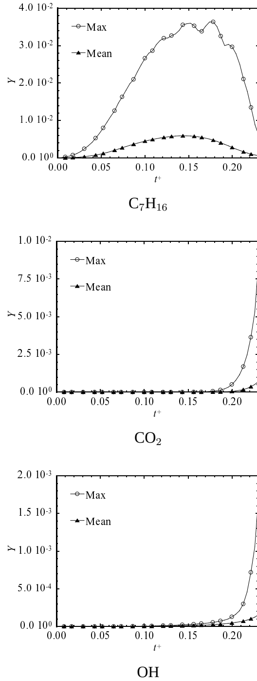
Figure 5.4: Temporal developments of mass fraction of major species.
