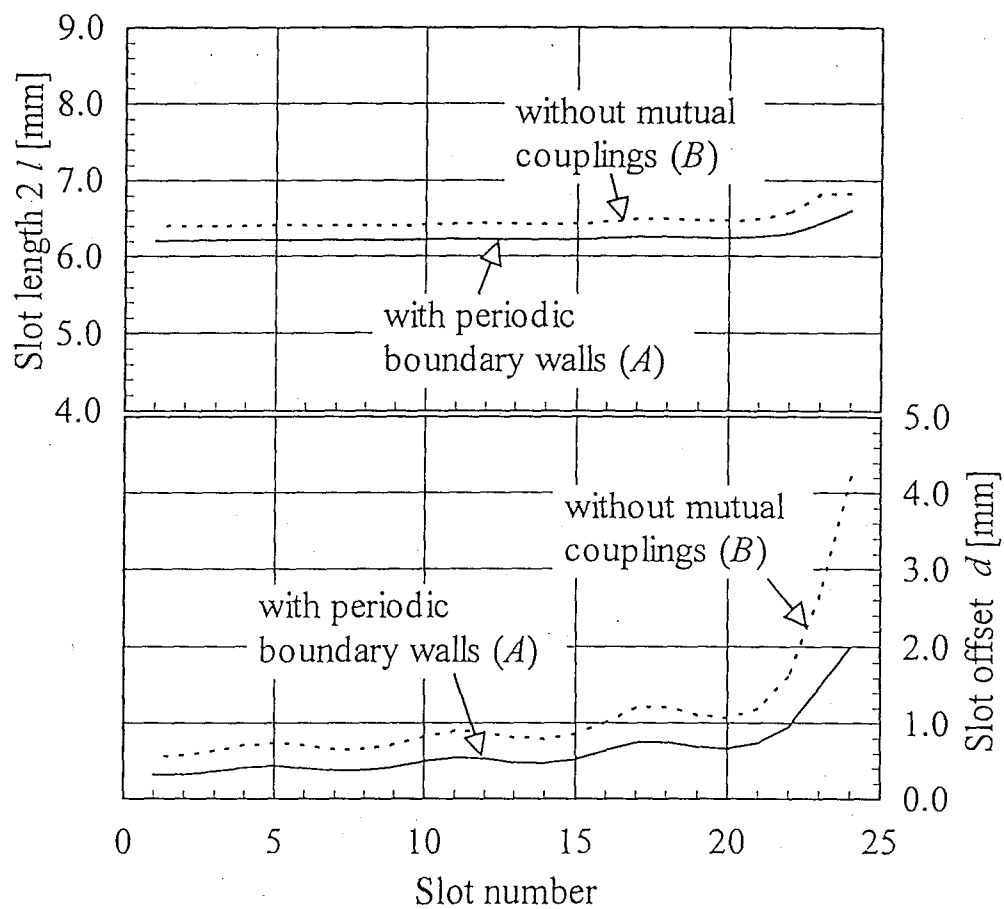
Fig.3.6 Slot parameters related to normalized conductance
