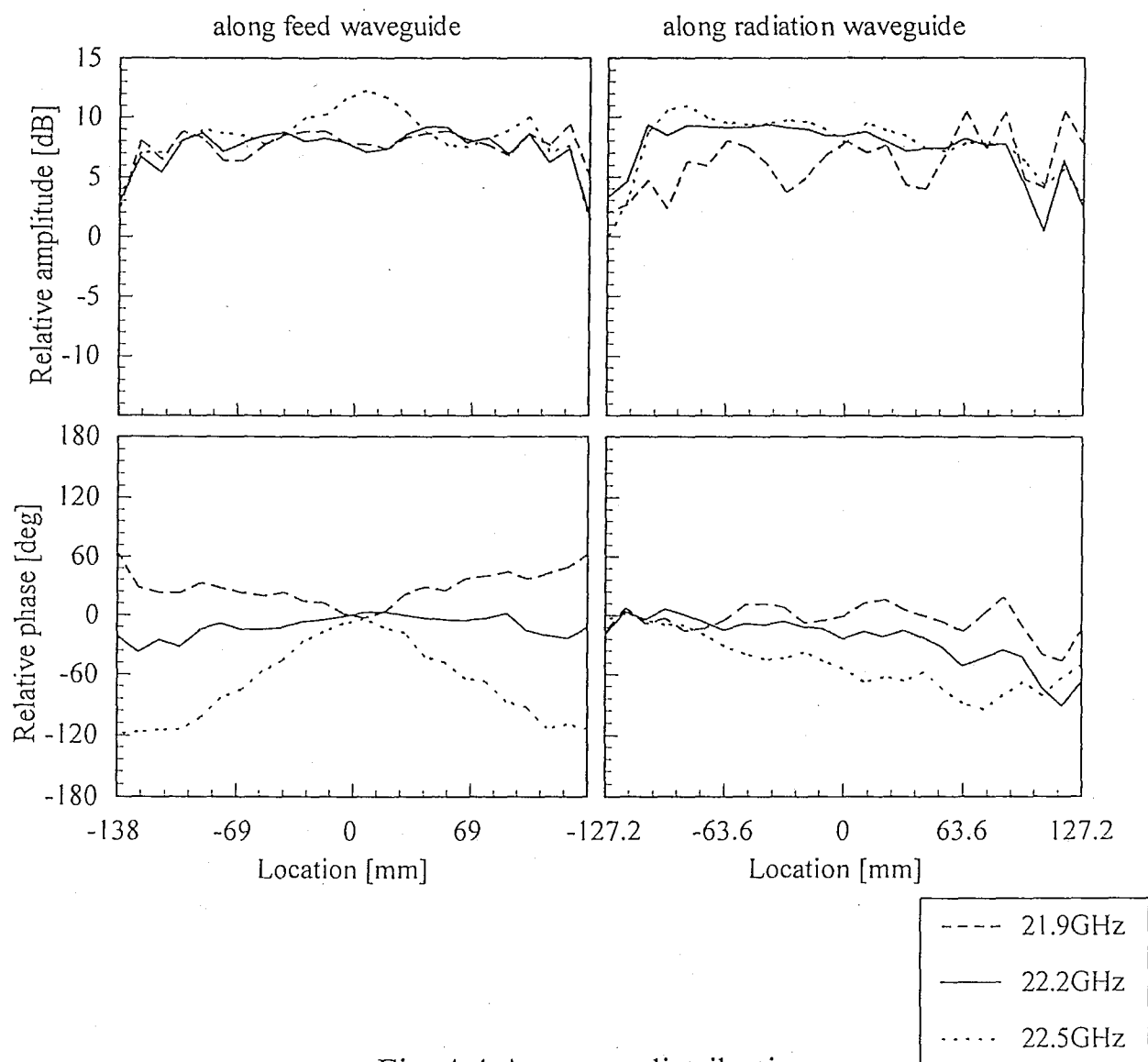
Fig. 4.4 Aperture distribution
