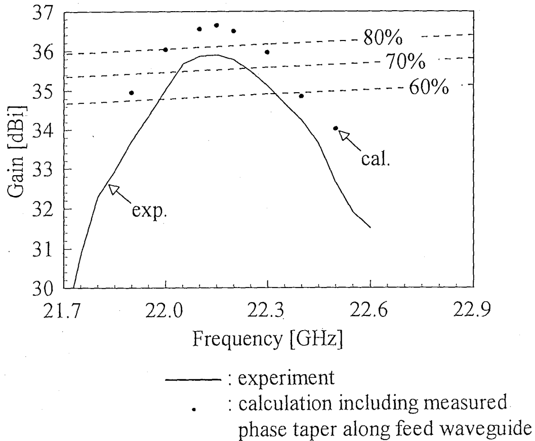
Fig. 4.2 Gain and antenna efficiency
