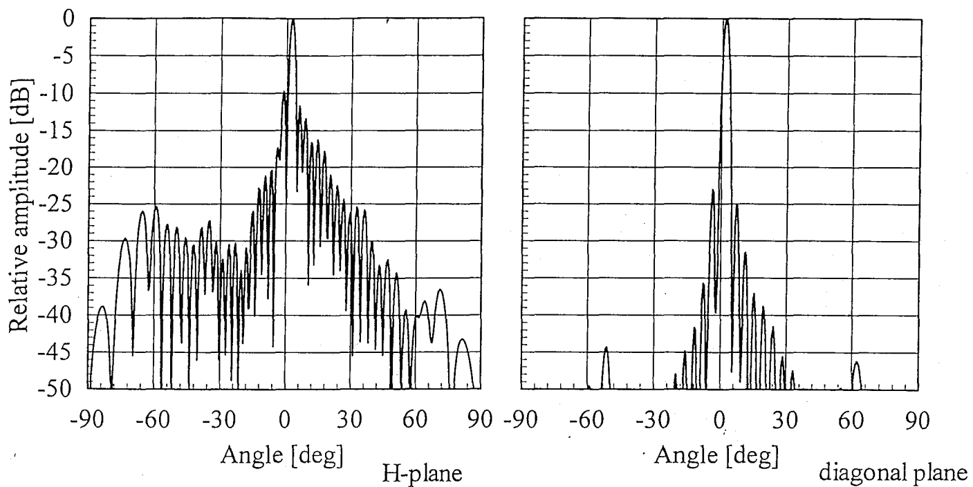
Fig. 4.8 Radiation pattern
