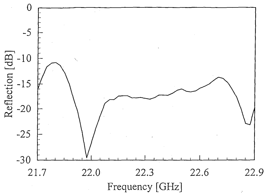
Fig.4.3 Reflection characteristics
