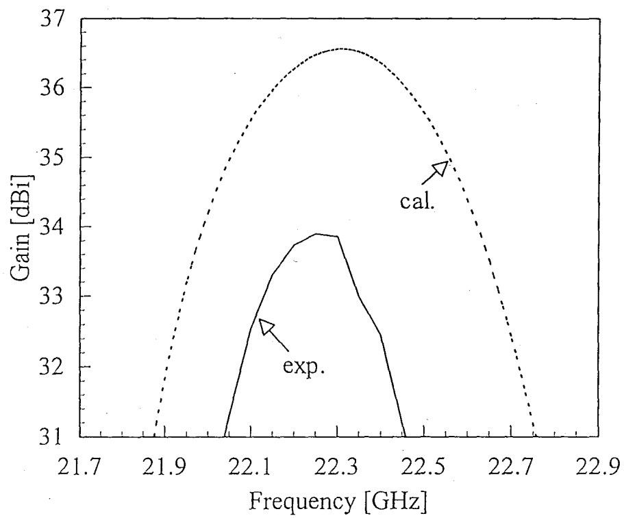
Fig. 2.18 Antenna gain
