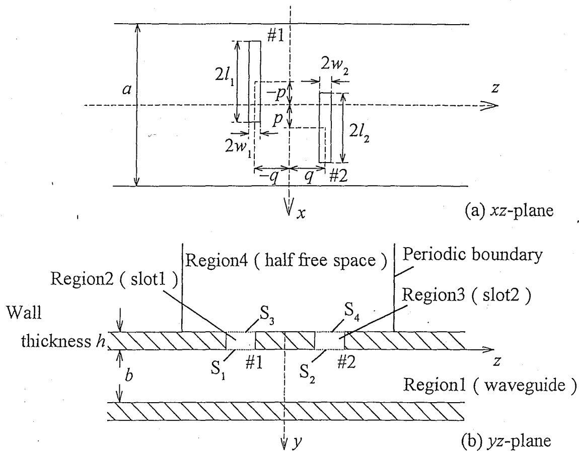
Fig. 6.3 Analysis model of reflection-cancelling slot pair
