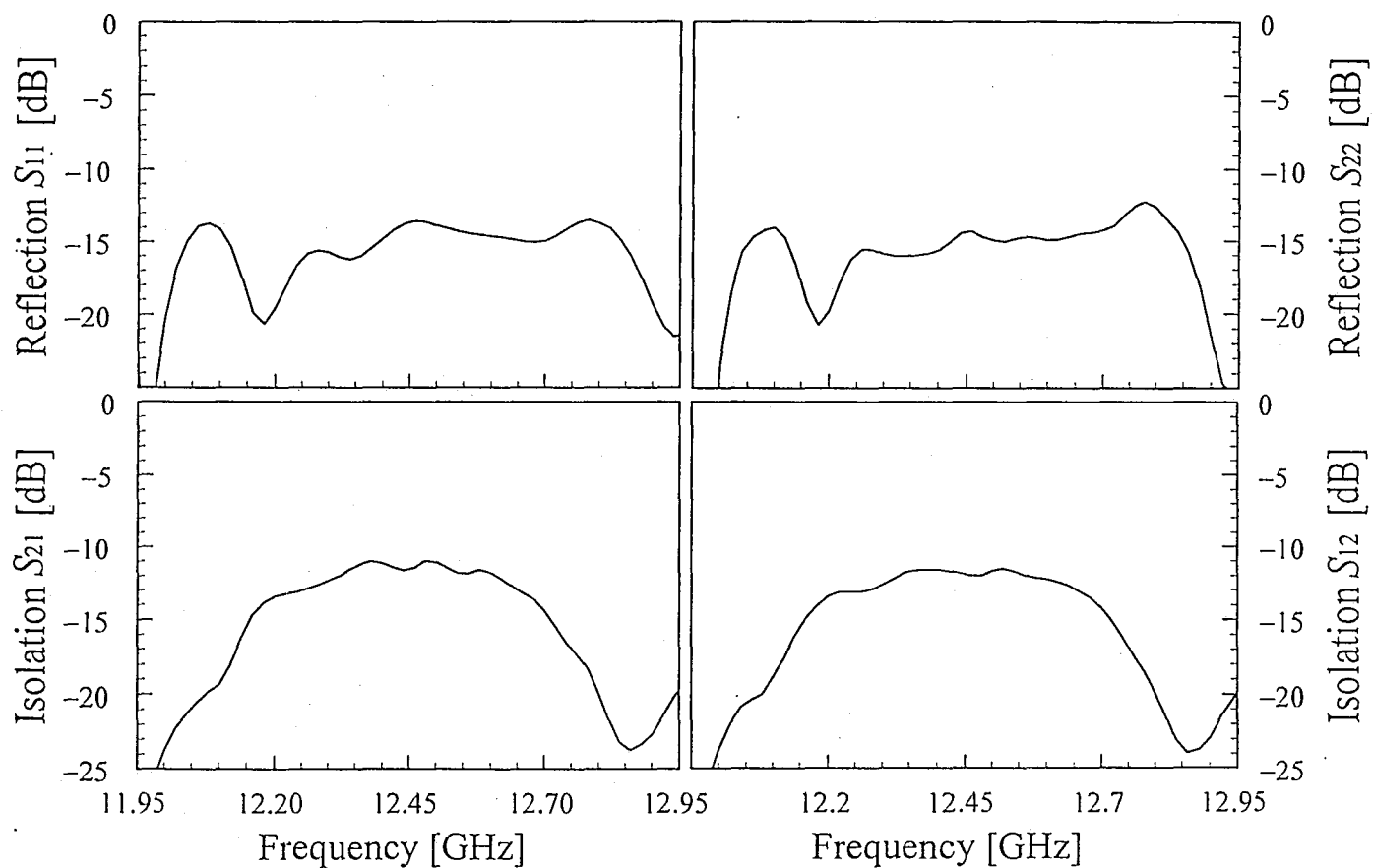
Fig. 5.6 Reflection and isolation characteristics of port #1 and #2
