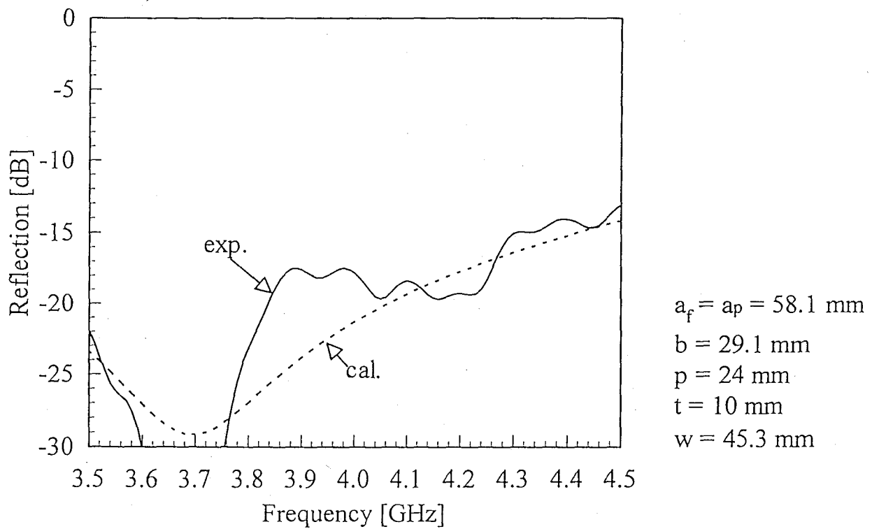
Fig. 2.5 Reflection characteristics of the model 2 with iris
