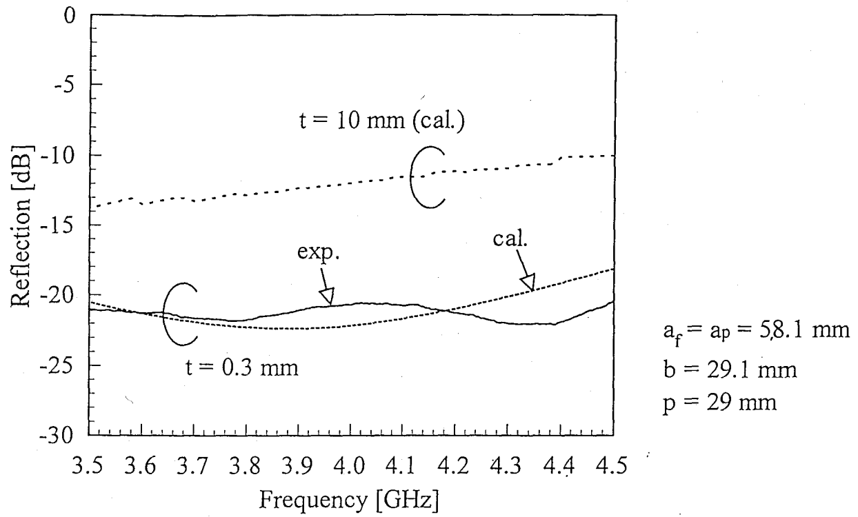
Fig. 2.4 Reflection characteristics of the model 1 without iris
