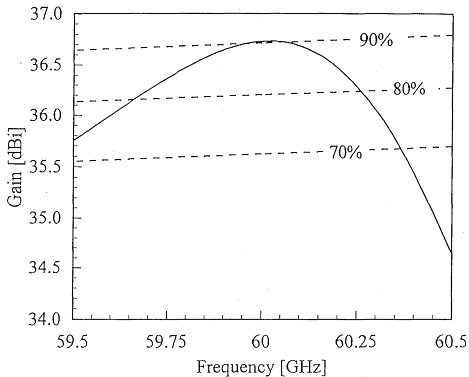
Fig. 4.9 Gain and antenna efficiency
