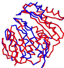
Figure 3-6-d-3. A superimposition of the Cα chains between the two subunits of the dimer in the St -Rtc+AMP crystal. The A-subunit and A'-subunit are indicated by wire models with blue and red colors, respectively.
