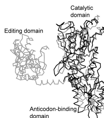
Figure 4. Superimposed Ca chains of Ap ThrRS-1 (black) onto Ec ThrRS (gray, PDB-ID=1QF6).
