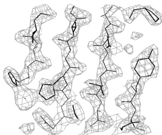
Figure 7-3-c-1. A part of the final 2|F_o| - |F_c| electron density map of the Ap ThrRS-1 crystal, contoured at 1.5 \sigma level (colored in gray).
