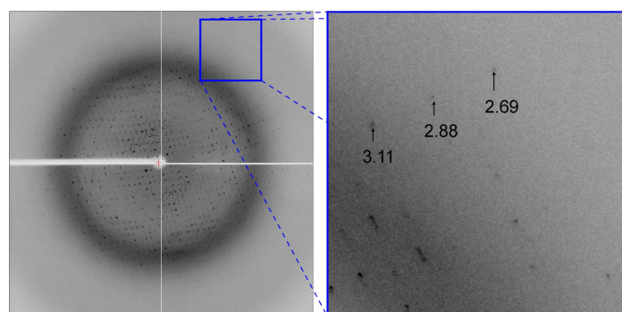
Figure 7-8-b-2 An X-ray diffraction image of S /ThrRS-2* crystal, taken with an oscillation angle of 1^\circ (left) and its zoomed up image in a box (right). Arrows indicate diffraction spots at the resolutions shown with values.
