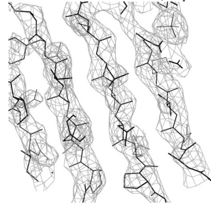
Figure 3-6-c-1. A part of the final 2|F_o| - |F_c| electron density map of the St -Rtc+AMP crystal, contoured at 1.5 \sigma level (colored in gray).
