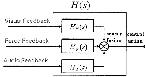
Figure 3-18: Multimodal sensory feedback scheme
