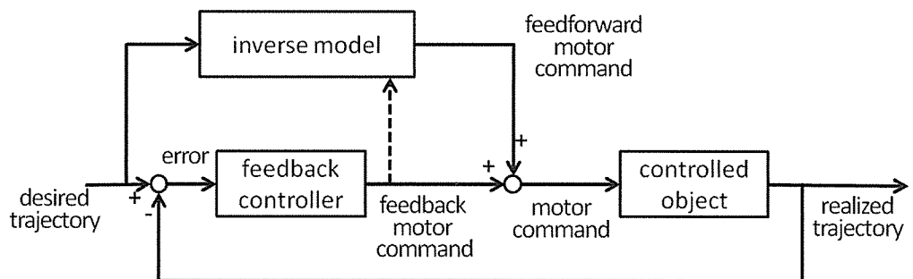
Figure 2-1: Three computational schemes for acquiring an inverse model through learning. Broken lines show information used for training. A Direct inverse modeling approach. B Forward and inverse modeling approach. C Feedback-error-learning approach. Modified from [19].
