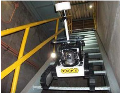
Figure 3: Survey Runner developed by TOPY Industries, Limited. ( http://www.topy.co.jp/release/201203/entry396.html )
