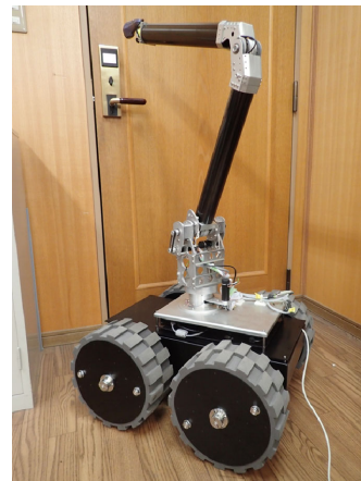
Figure 6: RhinoUS-I, a mobile manipulator with ultrasonic sensors
