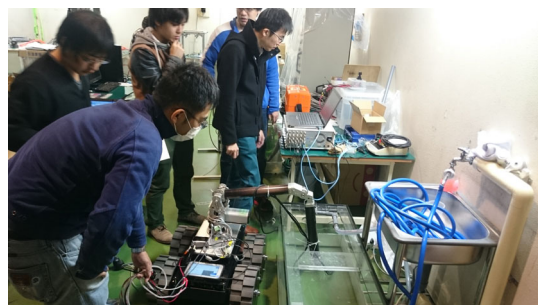
Figure 7: Students measured water flow in a tank by using ultrasonic sensors. Robot location and arm posture were remotely controlled by the students.
