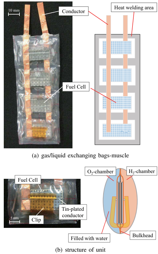
Fig. 6. Structure of the prototype gas/liquid conversion drive bags-muscle. PEFCs are built into each of contractile units.
