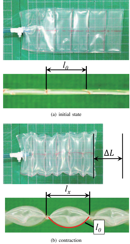
Fig. 4. Contraction of a bags-muscle which applied air pressure is 20 kPa
