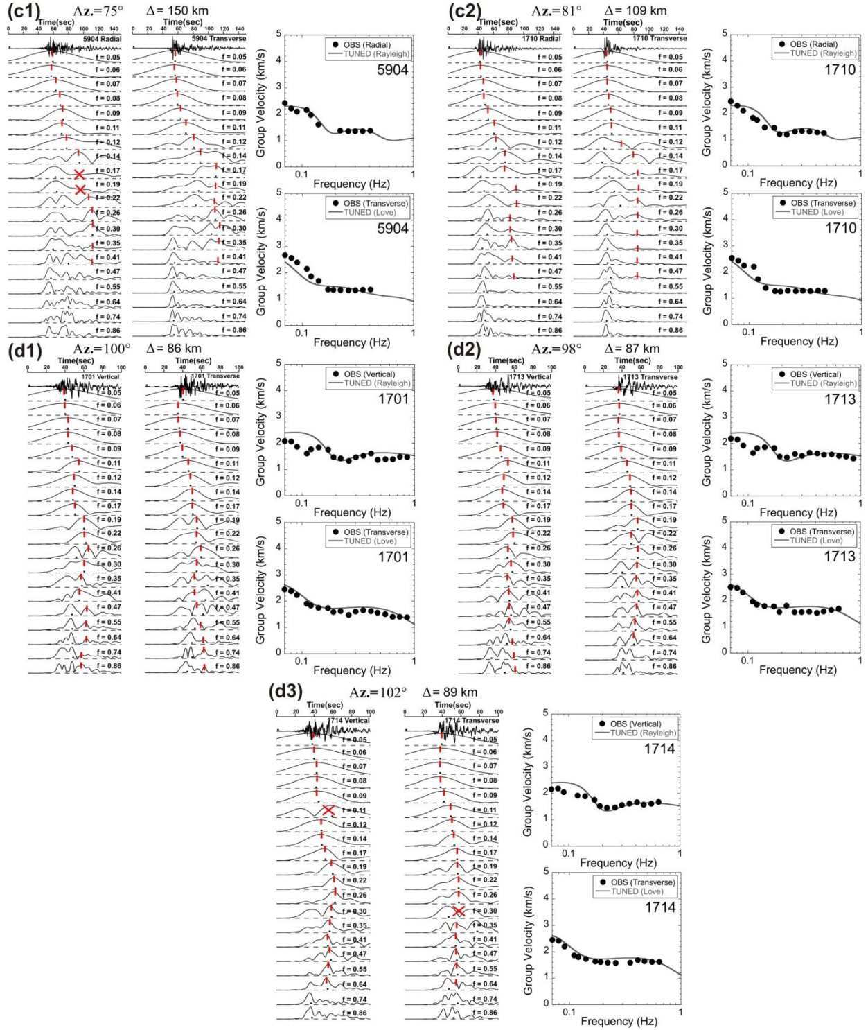
Figure 3.4 Result of multiple filter analysis for the radial or vertical (most left) and transverse (second from left) components at the stations in each azimuthal direction: 2201 (a), 5902, 5910, 5908, 5907, 5906 (b), 1710, 5904 (c), and 1701, 1713, 1714 (d). The envelopes of seismograms are given for the frequency range between 0.05 and 0.86 Hz. Red line shows the group delay time of surface waves at each frequency. Red cross shows the failure in reading the group delay time. The comparison between the group velocities of observed and tuned models for Rayleigh (top) and Love (bottom) waves are given on the right hand side of the seismograms.
