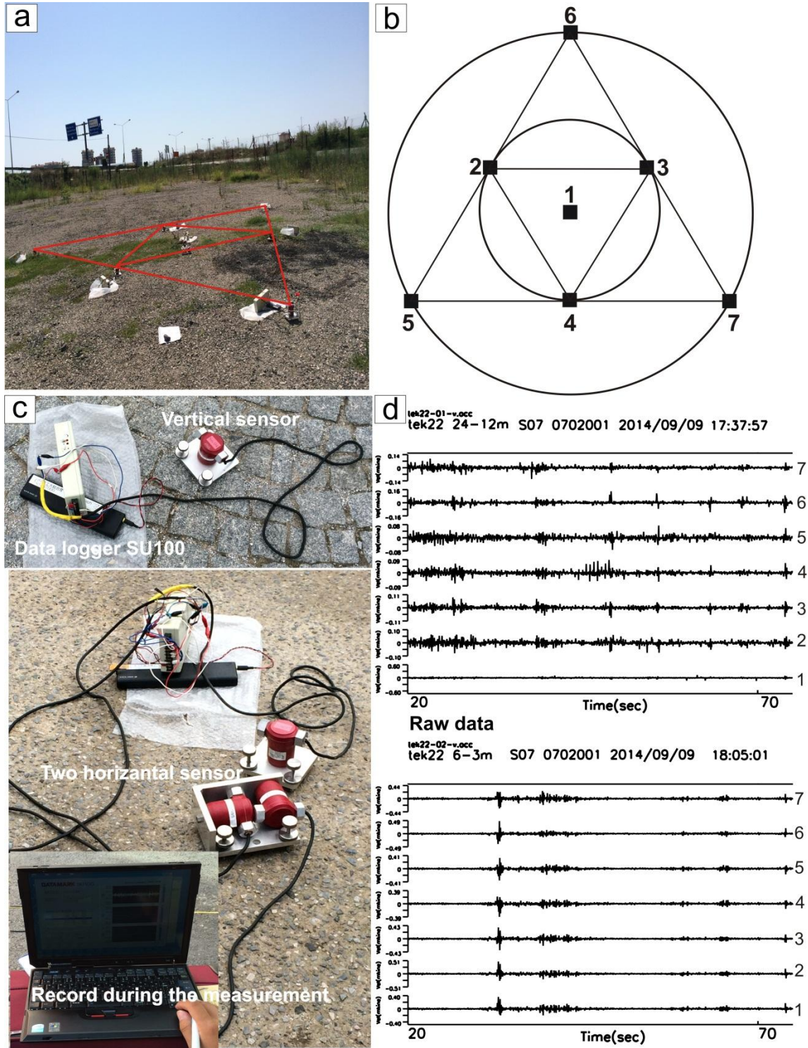
Figure 2.4 a) Example of vertical configuration at T22 (24-12, 6-3 m). b) Circular double triangular array configuration. Numbers show location of accelerometers. c) Vertical, horizontal sensors with data loggers d) Example of simultaneously seven vertical acceleration records of both arrays at site T22.
