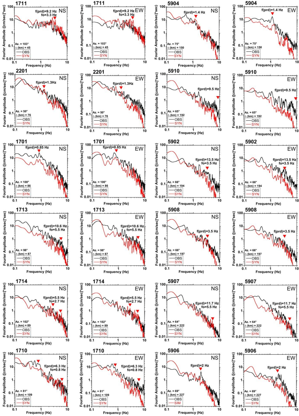
Figure 4.7 Comparison of the amplitude spectrums of the observed (black) and synthetics (red) velocity waveforms. f (prd) and f_0 are the predominant and fundamental frequencies that were obtained from site amplifications given in Figure 2.17, respectively, are shown by red inverted triangles. (a) Gokceada, Enez, Canakkale city center, Gelibolu stations (b) Tekirdag city center, Corlu, Marmara Ereglisi stations.
