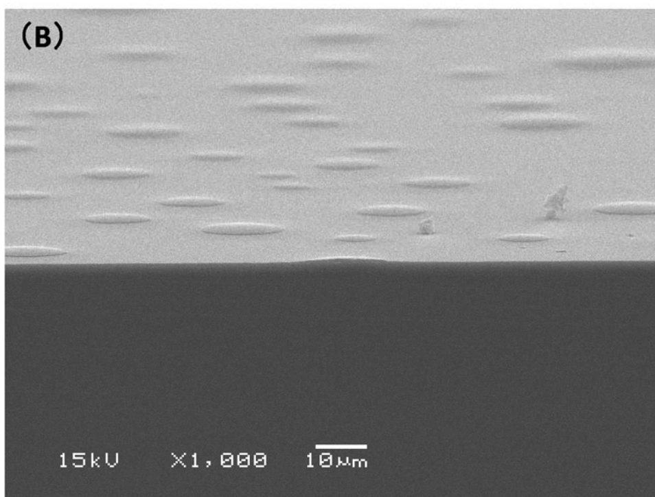
Fig. 4-1 (B). SEM image of the cross section of PI- Expt. No.1.
