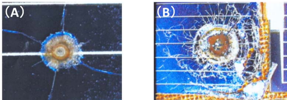
Fig. 2-3. Front-top impacts (2-10) .
