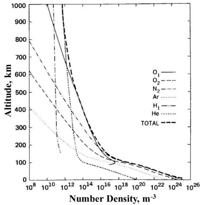
Fig. 1-9. Number density of individual species and total number density as a function of altitude (1-32) .
