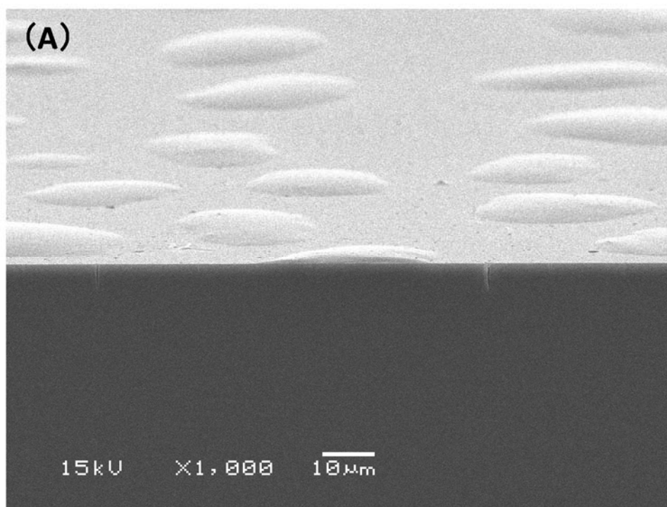
Fig. 4-1 (A). SEM image of the cross section of polyimide film as deposited with silicone contaminants.
