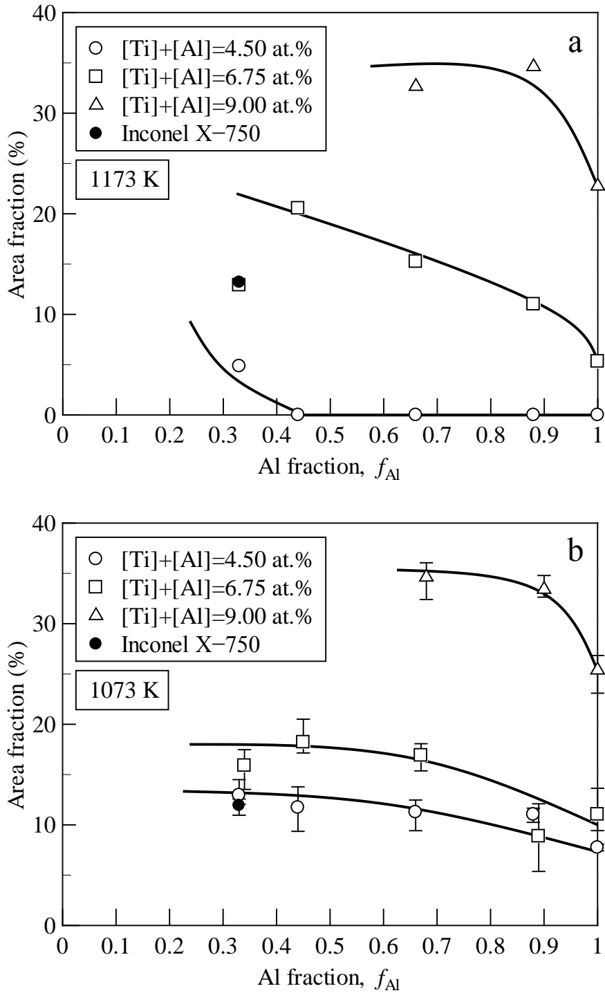
Fig. 4-13 Area fraction of \gamma' phase with function of Al fraction f_{Al} in Ti and Al modified alloys aged at (a) 1173 K/10 h and (b) 1073 K/ 100 h
