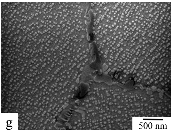
Fig. 2-7 SEIs of Inconel X-750 aged at 973 K for 0.05 h (a), 0.17 (b), 1 h (c), 5 h (d), 24h (e), 96h (f) and 750 h (g).
