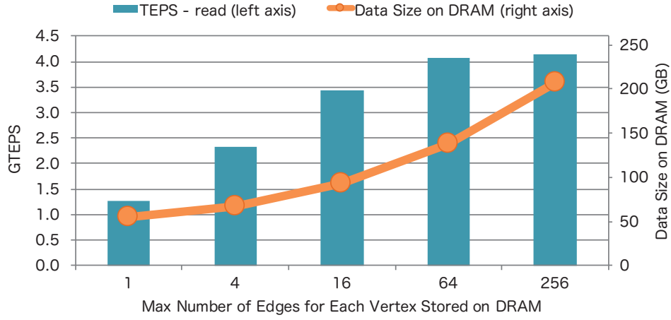
Figure 3.11: BFS Performance and Memory Consumption
