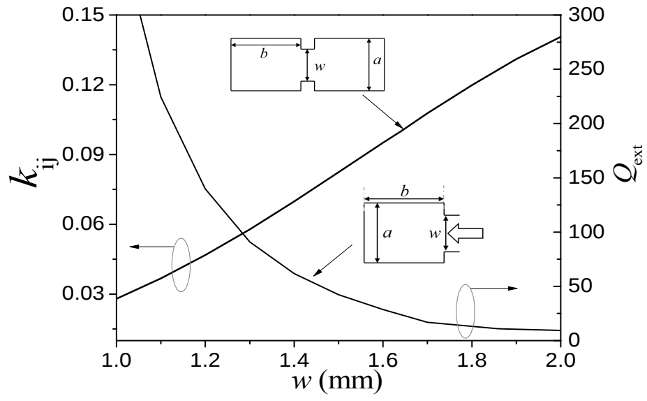
Fig. 2.5 Simulated k_{ij} and Q_{\text{ext}} as a function of w .
