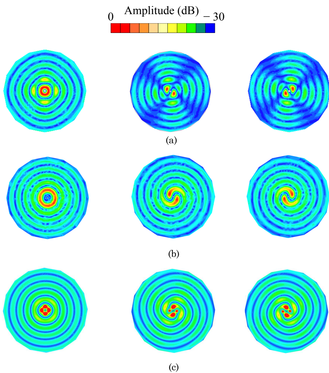
Fig. 4.8 Amplitude distribution of operation modes inside the PPW (from left to right are modes 0, -1 and +1 , respectively). (a) Bended slots. (b) Center ring slot. (c) Open posts.
