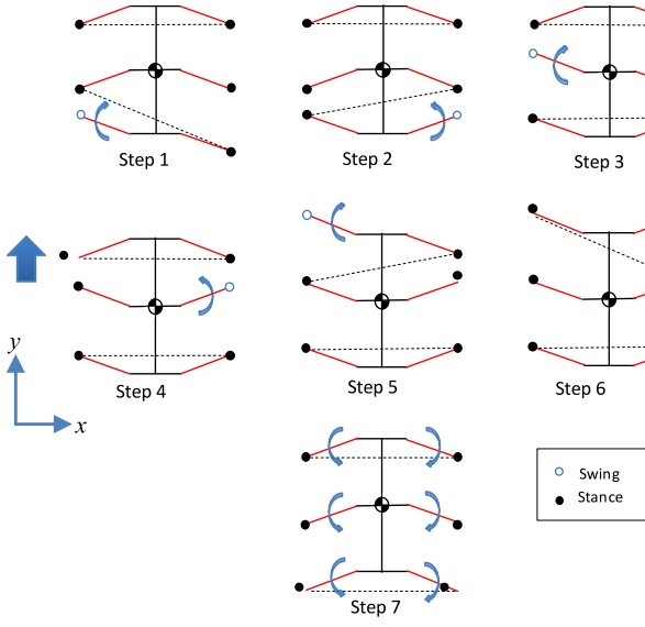
Fig. 6. Customized Wave gait walking pattern.
