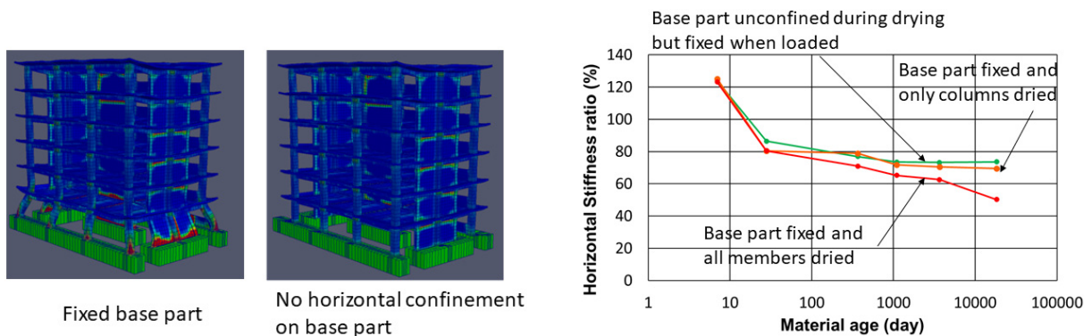
Fig. 12 Base part confinement to the columns on the first floor.
