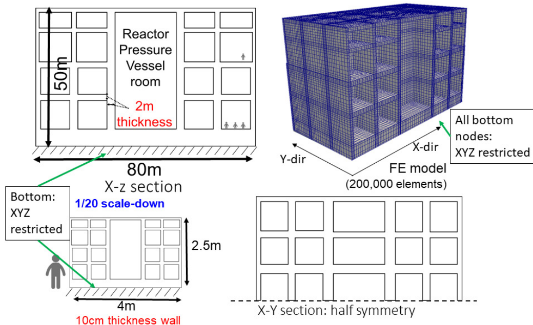
Fig. 6 Real scale mockup model of nuclear power plant and its scale down.
