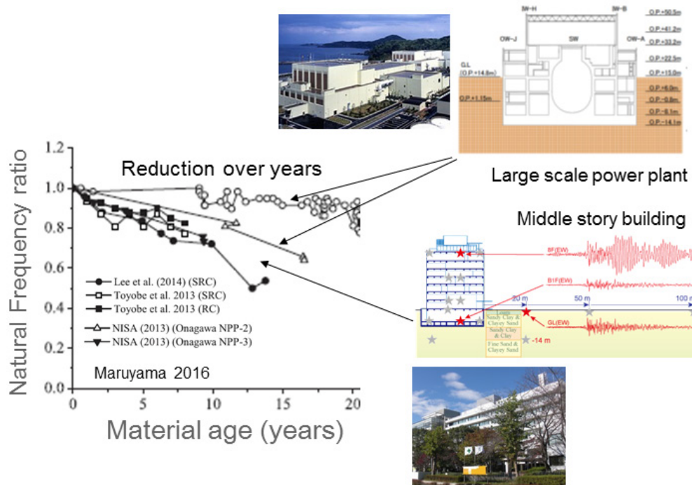
Fig. 1 Reduced natural frequency of concrete structures with different dimensions (Maruyama 2016).
