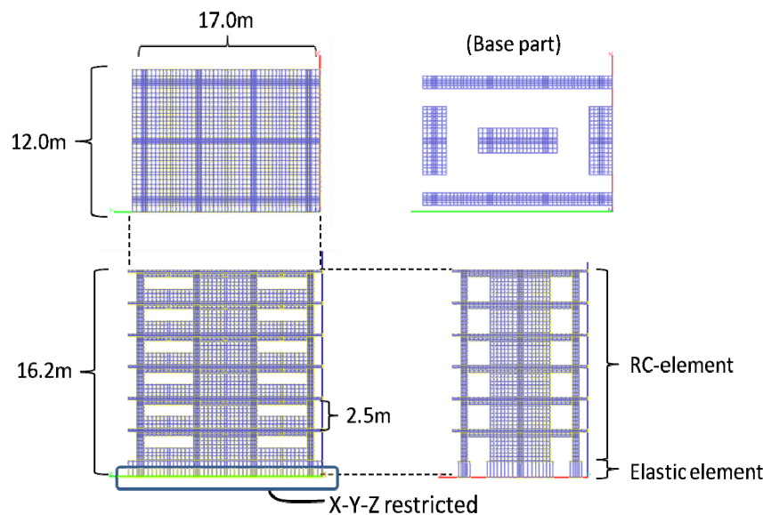
(a) Finite element discretization and member arrangement (Chijiwa and Maekawa 2016).
