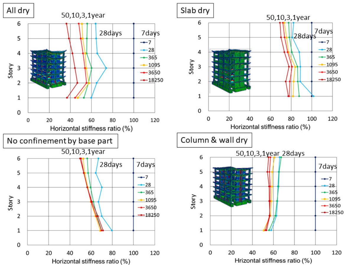
Fig. 11 Effect of partial drying shrinkage on the overall stiffness.
