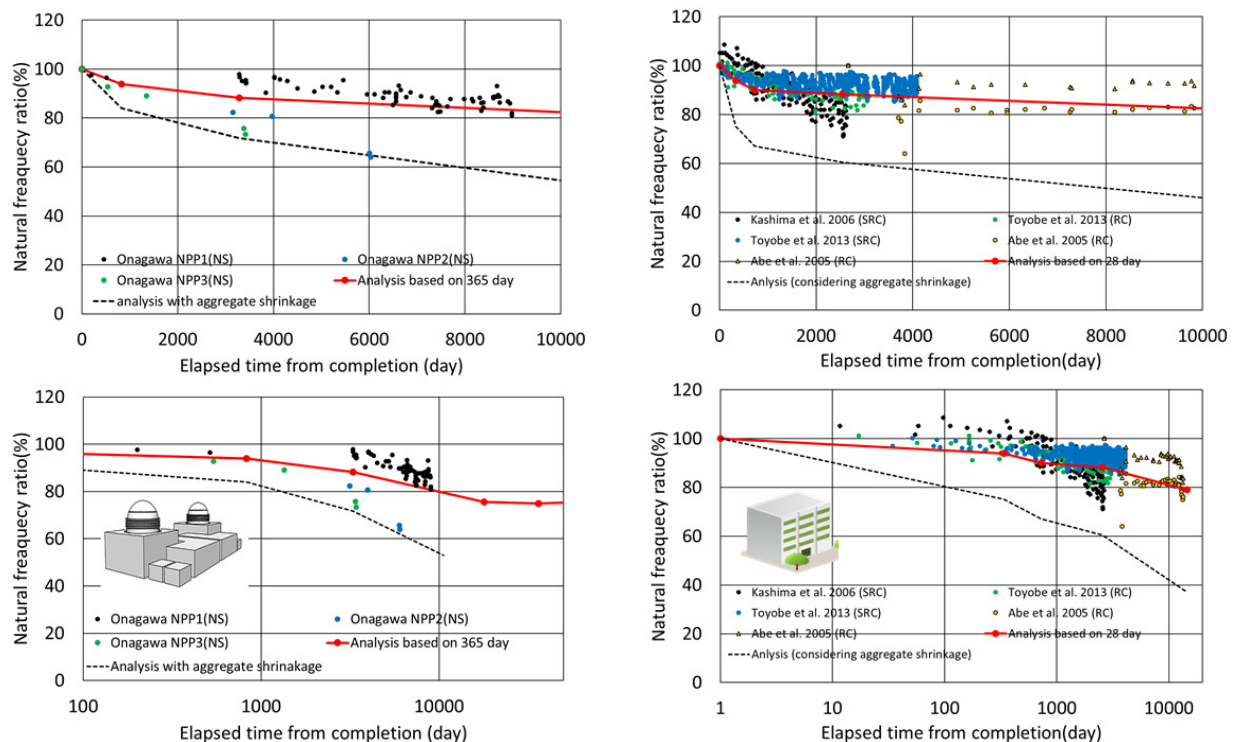
Fig. 9 Computed transient natural frequency over the life time of RC structures with largely different dimensions: left=nuclear plant, right=multi-story building.
