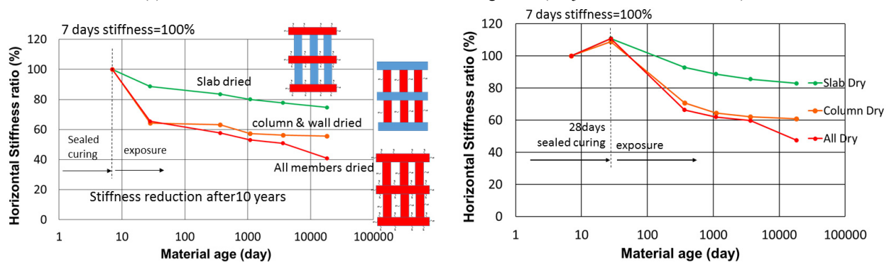
(b) Horizontal stiffness decay of each local drying condition.
