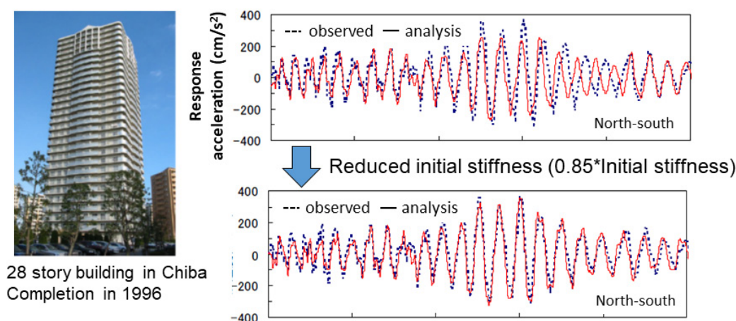
Fig. 3 Seismic analysis of 28-story RC building with reduced initial stiffness (Ikawa et al. 2012).
