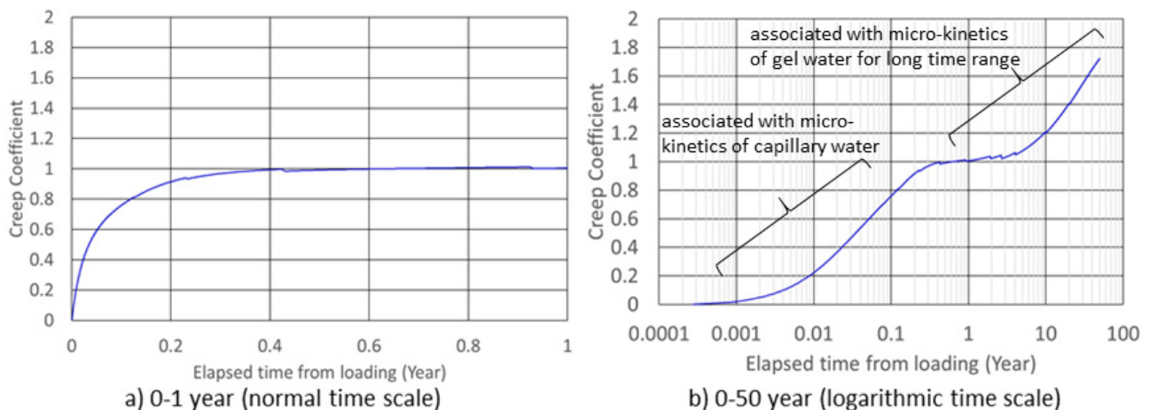
Fig. A2 Computed basic creep coefficients by thermo-hygral analysis.
