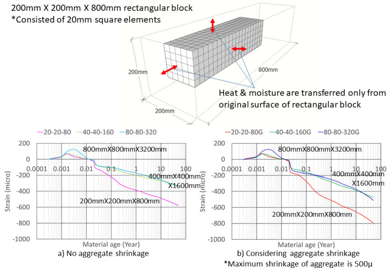
Fig. A1 Simulated drying shrinkage of the concrete specimen by thermo-hygral analysis.
