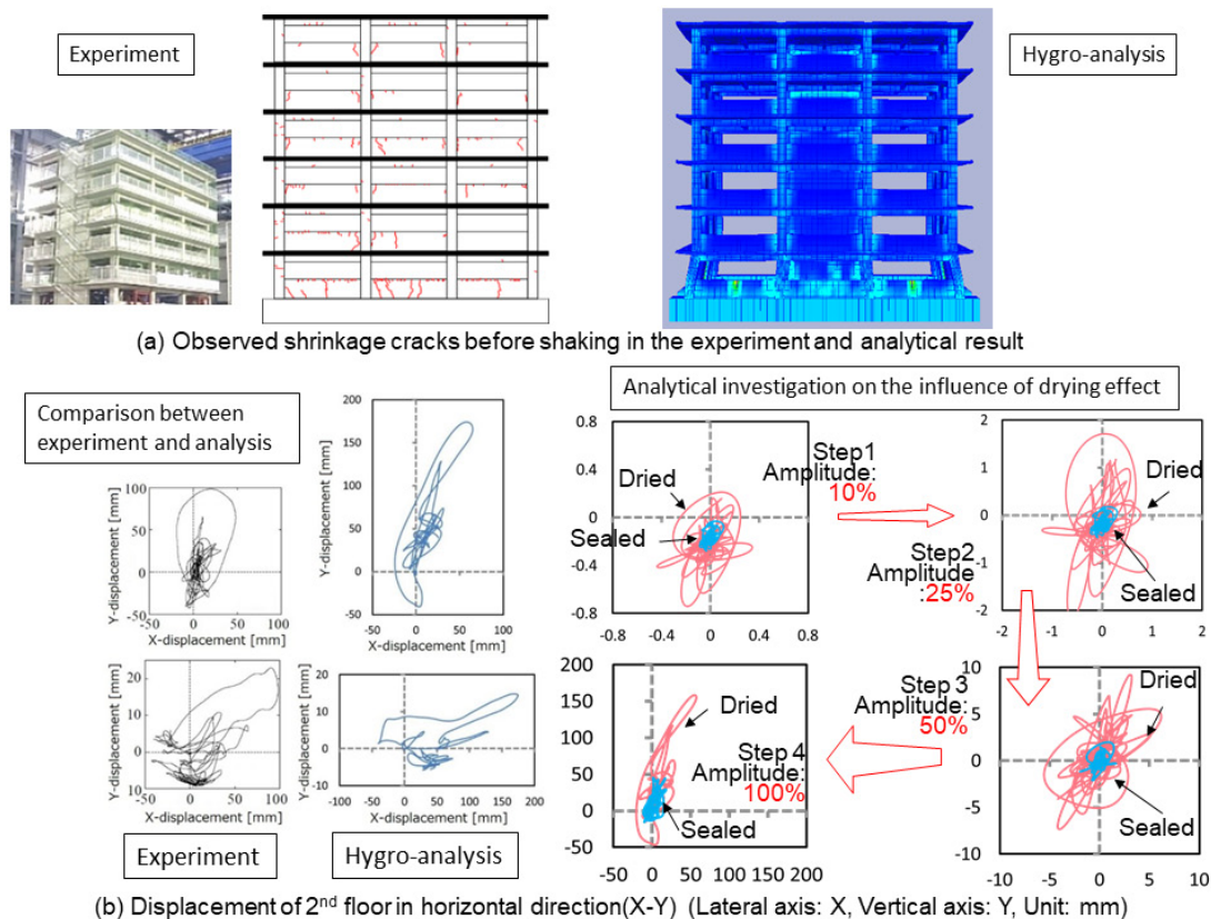
Fig. 2 Seismic response analysis of RC building with and without drying (Chijiwa and Maekawa 2016).
