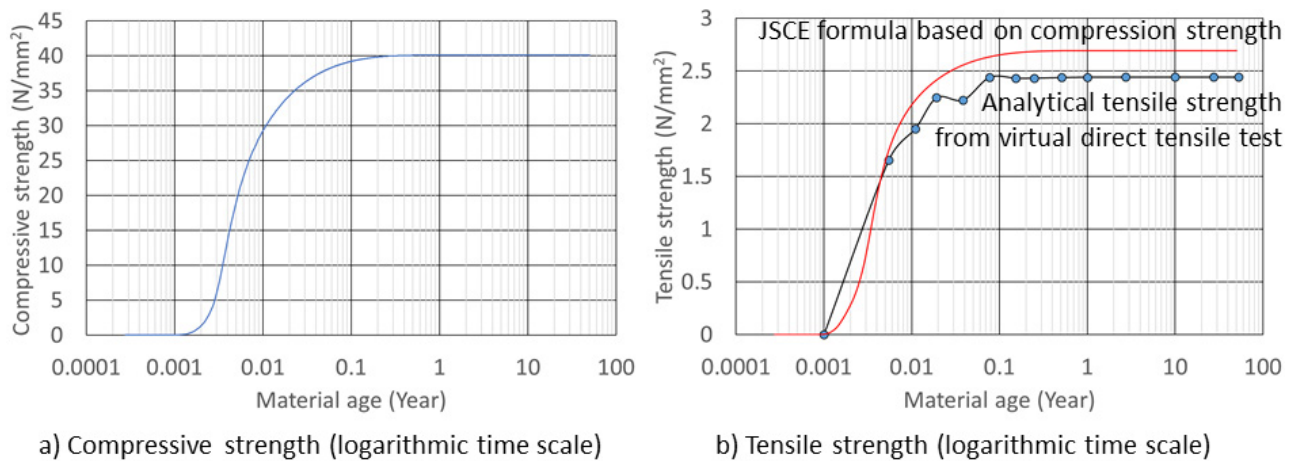
Fig. A3 Computed strength development by thermo-hygral analysis.
