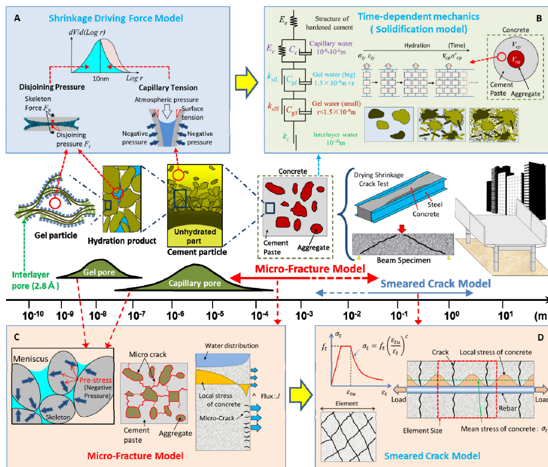
Fig. 4 Schematic platform of multi-scale thermo-hygro analysis (Yoneda et al. 2013, 2015).
