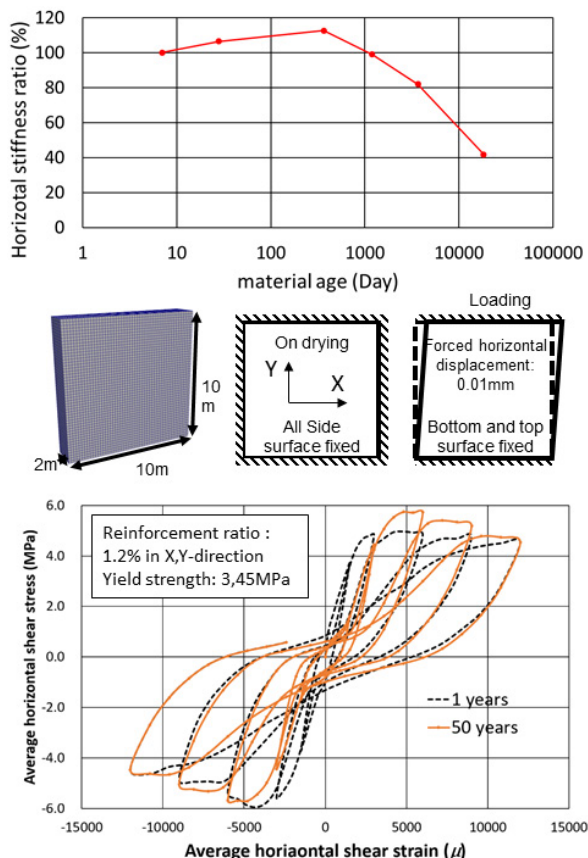
Fig. 8 Effect of shrinkage on the initial stiffness and the restoring force characteristics.
