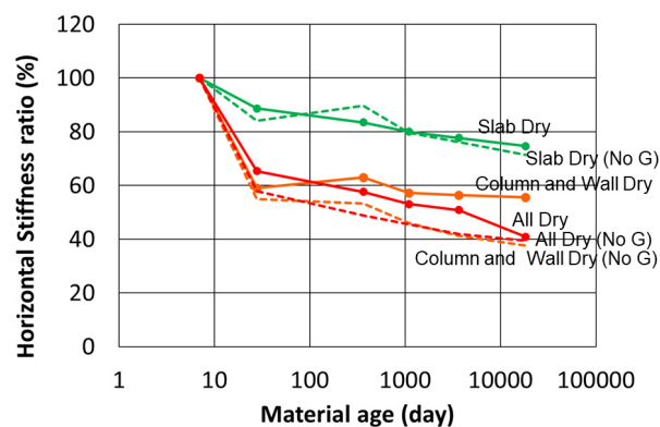
Fig. 13 Stiffness decay under zero gravity.
