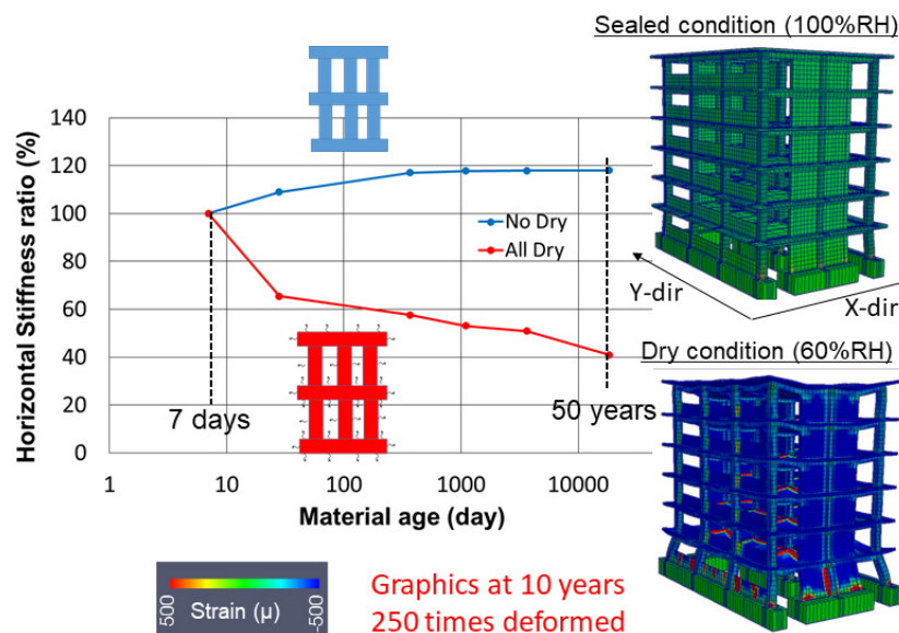
Fig. 5 Averaged drift stiffness of the whole structures.
