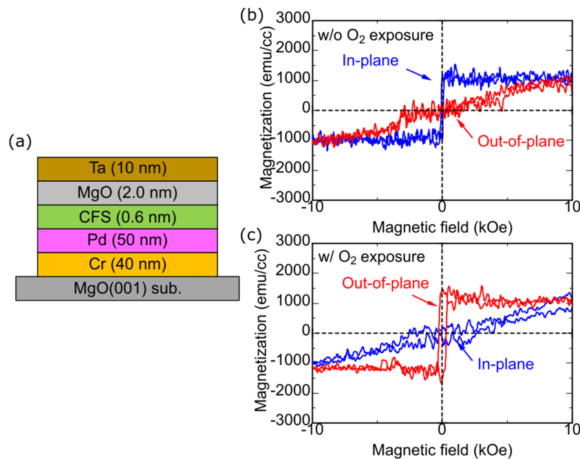
FIG. 1. (a) Stacking structure. In-plane (blue) and out-of-plane (red) M - H loops of CFS(0.6 nm)/MgO(2.0 nm) bilayer samples prepared (b) without and (c) with oxygen exposure after deposition of CFS layers.
