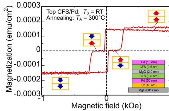
FIG. 3. Out-of-plane M - H loop of Cr (40 nm)/Pd (50 nm)/CFS(0.6 nm)/MgO(2.0 nm)/CFS(0.6 nm)/Pd (10 nm). The inset shows the sample structure.
