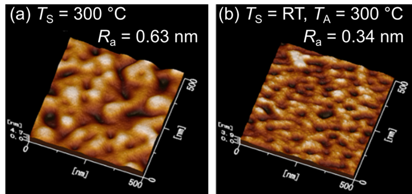
FIG. 2. AFM images of the surface of (a) the top CFS layer deposited at T_s = 300^\circ\text{C} and (b) at T_s = \text{RT} and subsequently annealed at T_A = 300^\circ\text{C} .
