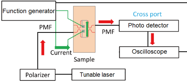
Fig. 8. Experimental setup for measuring temporal response.
