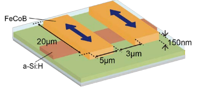
Fig. 2. Design of thin-film magnets.
