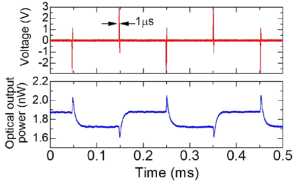
Fig. 9. Measured temporal response of MO switch to a pulsed current.
