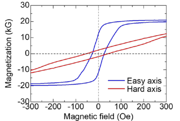
Fig. 4. Hysteresis loops of 20 \mu\text{m} \times 5 \mu\text{m} strip array of FeCoB.
