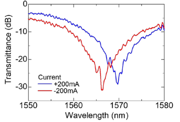
Fig. 7. Measured transmission spectra of MO switch several seconds after ceasing the current.
