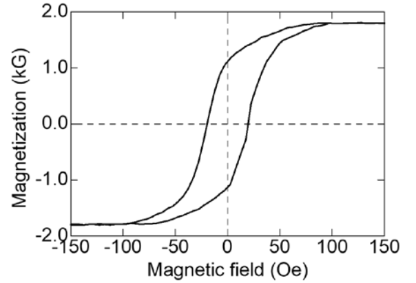
Fig. 3. Hysteresis loop of Ce:YIG.
