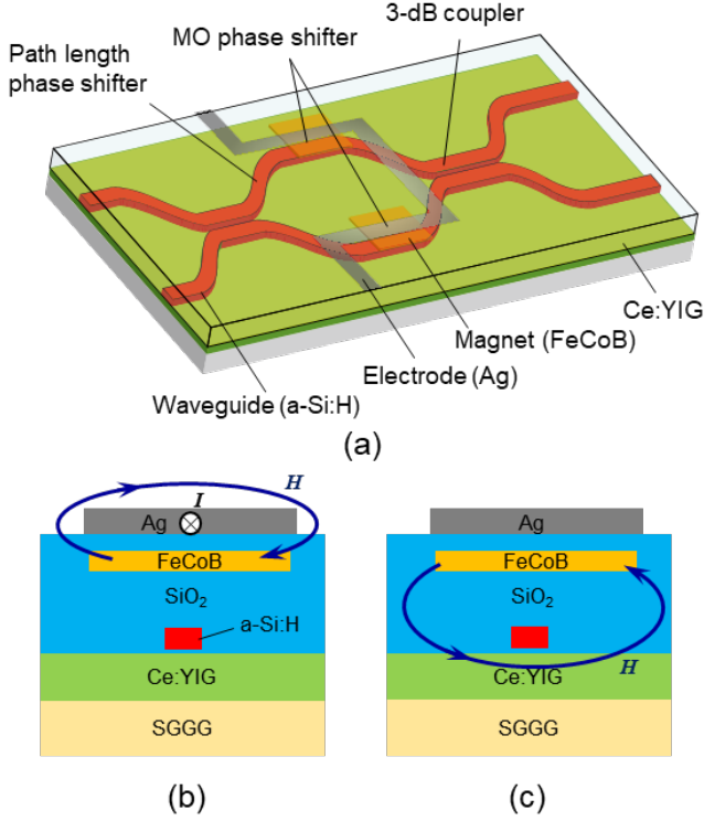
Fig. 1. (a) Configuration of proposed magneto-optical switch. (b) Changing switching state via current flow. (c) Maintaining switching state because of non-volatility of thin-film magnet.
