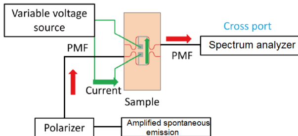
Fig. 6. Experimental setup for measuring wavelength characteristics.
