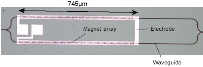
Fig. 5. Microscope image of fabricated MO switch.
