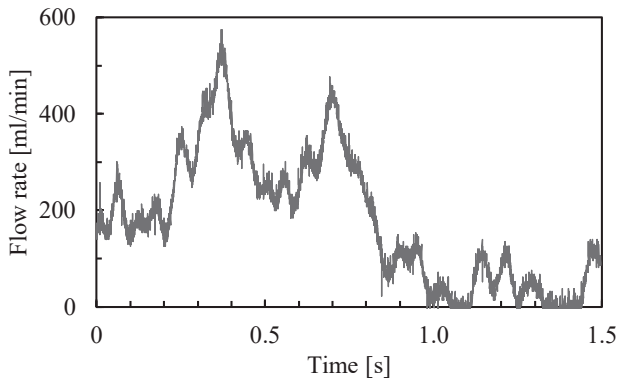
Fig. 15 Transition of flow rate, when the value of kinematic viscosity, applied pressure, and applied voltage were 2 \text{ mm}^2/\text{s} , 0.3 \text{ MPa} , and 80 V_{p-p} , respectively.
