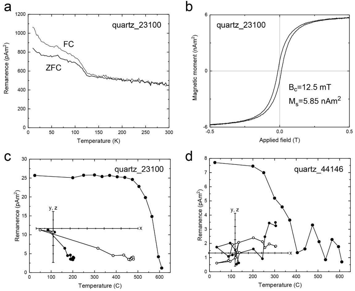
Fig. 7 Results of experiments on selected quartz. a Low-temperature remanence measurements. Solid lines for ZFC measurements and dotted lines for FC measurements.
