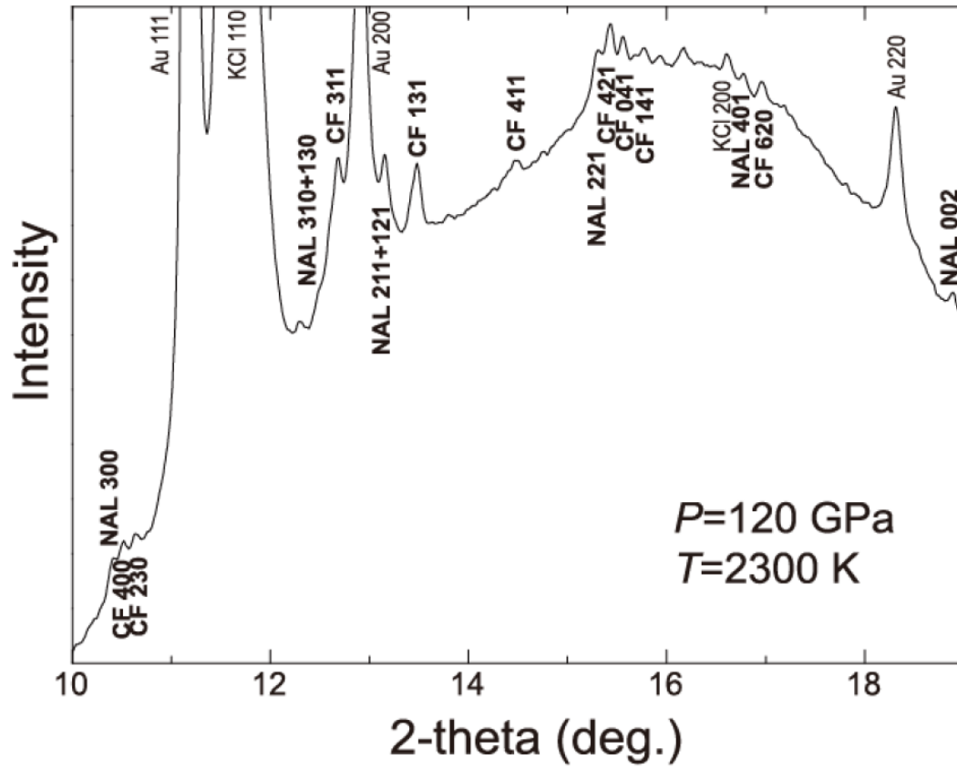
Figure S1. XRD pattern of \text{Na}_{0.75}\text{K}_{0.25}\text{Mg}_{2.00}\text{Al}_{4.80}\text{Si}_{1.15}\text{O}_{12} (Na75K25) bulk composition obtained during heating at 2300 K and 120 GPa.
