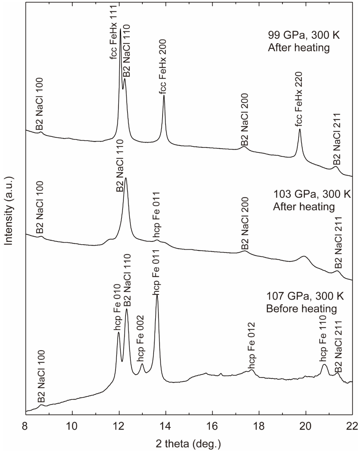
Fig. 2 Representative XRD patterns obtained in a series of laser heating for an iron sample and H 2 with NaCl pressure medium. (Lower pattern) The diffraction lines from hcp iron obtained at 107 GPa before laser heating. (Middle) XRD peaks from hcp Fe and halo taken at 103 GPa and 300 K after laser heating. (Upper) XRD peaks from fcc FeHx after laser heating.
