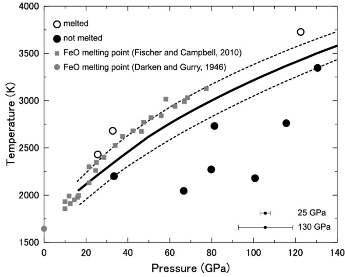
Fig.2. The solidus curve of \text{Fe}_2\text{SiO}_4 , corresponding to the eutectic melting curve in the \text{FeO-SiO}_2 binary system to the deep lower mantle. Melted and not-melted samples obtained in this study are shown by open and closed circles, respectively. Gray circle and squares indicate the previously determined melting temperatures of \text{FeO} at 1 bar (Darken and Gurry, 1946) and at high pressures (Fischer and Campbell, 2010). The upper and lower bounds of the melting curve are given by the melting temperature of \text{FeO} end-member and by not-melted experiments, respectively.
