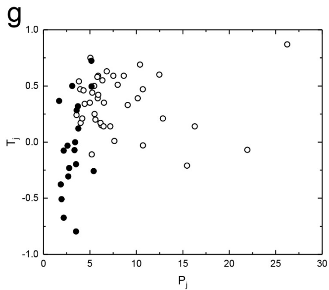
Fig. 8 (continued) g. The Jelinek diagram of single plagioclase crystals. Closed and circles for this study and Usui et al. (2015).
