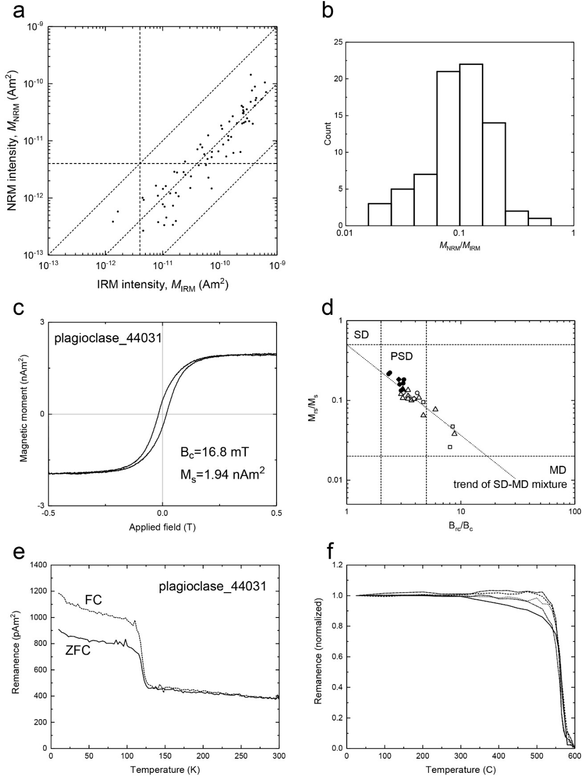
Fig. 8 Results of experiments on plagioclase. a . NRM intensity plotted as a function of IRM intensity. Horizontal and vertical dashed lines indicate the threshold for significant remanence. b . Histogram of NRM intensity divided by IRM intensity. c . Hysteresis loop measurement. d . Day plot of quartz and
