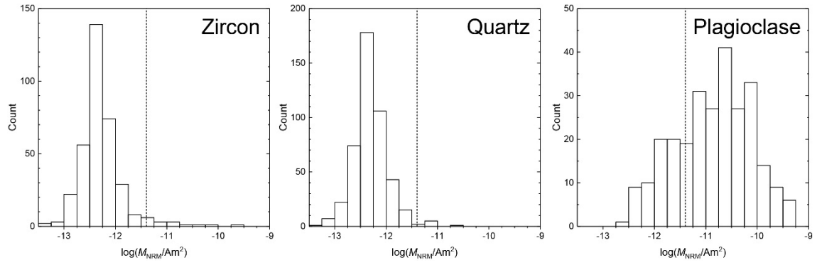
Fig. 5 Histogram of NRM intensity of zircon, quartz and plagioclase. Dotted lines indicate the threshold for significant remanence.
