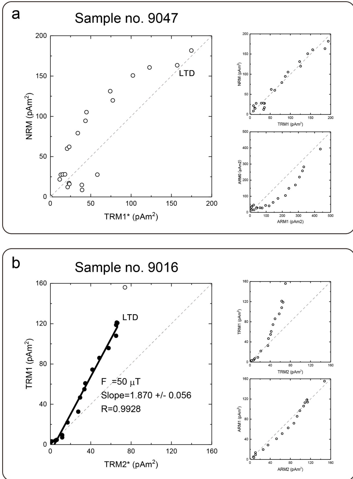
Fig. 10 Examples of failed paleointensity measurements by the Tsunakawa-Shaw method on single plagioclase grain. a No linear portion in the NRM/TRM1* plot. b TRM1/TRM2* slope severely exceeds 1.
