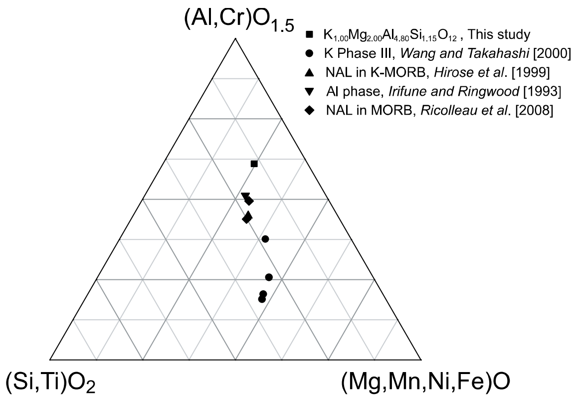
Figure S3. Chemical compositions of NAL projected onto the (\text{Al,Cr})\text{O}_{1.5} – (\text{Si,Ti})\text{O}_2 – (\text{Mg,Mn,Ni,Fe})\text{O} plane from (\text{K, Na})_2\text{O} . All Fe calculated as \text{Fe}^{2+} .
