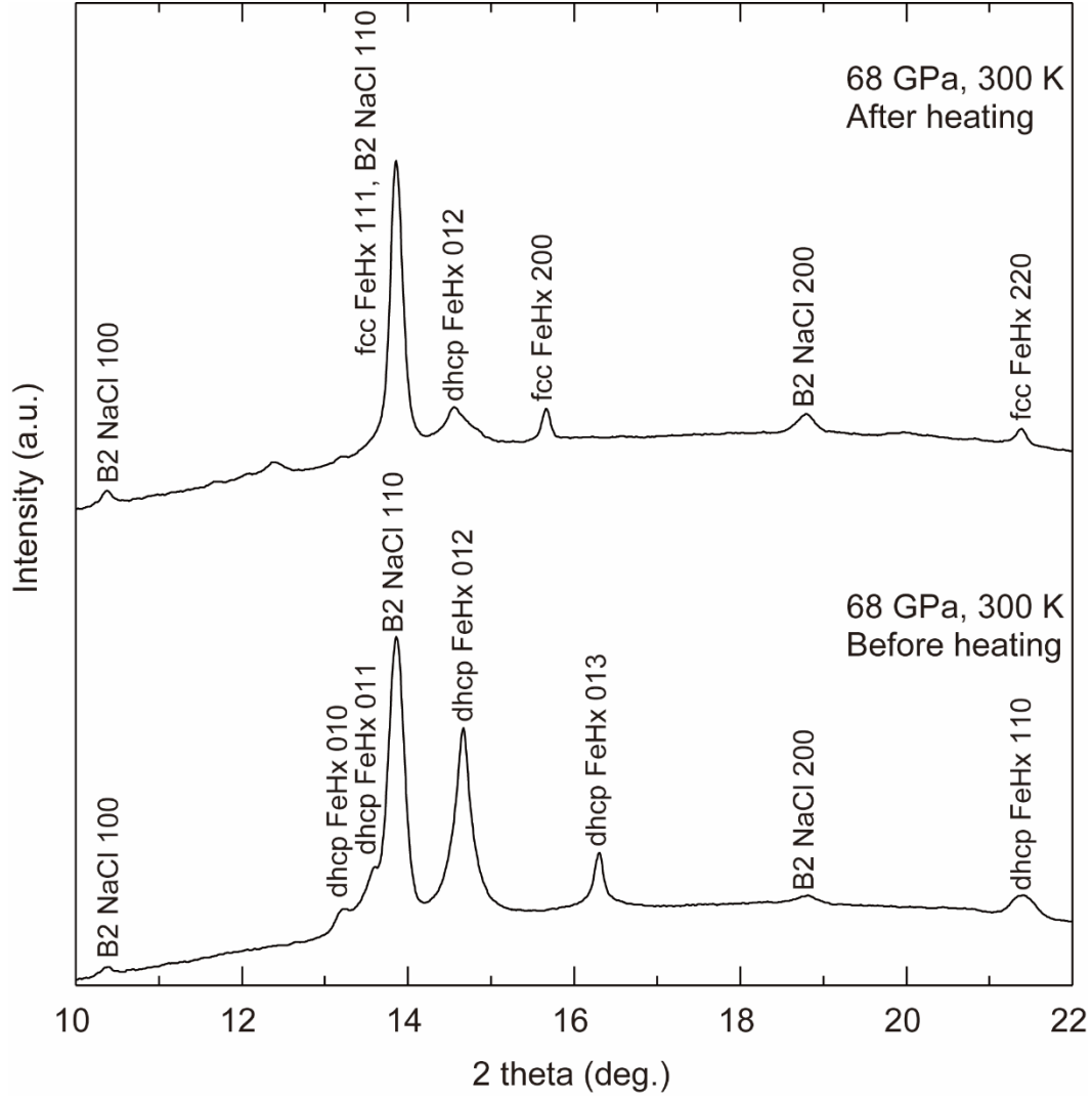
Fig. 3 Representative XRD patterns obtained in a series of laser heatings for an iron sample and H 2 with NaCl pressure medium. (Lower pattern) The diffraction lines from dhcp FeHx that are products of reaction of pure iron and H 2 at relatively low pressure and temperature during liquid H 2 sealing and compression. (Upper) XRD peaks from fcc FeHx after laser heating.
