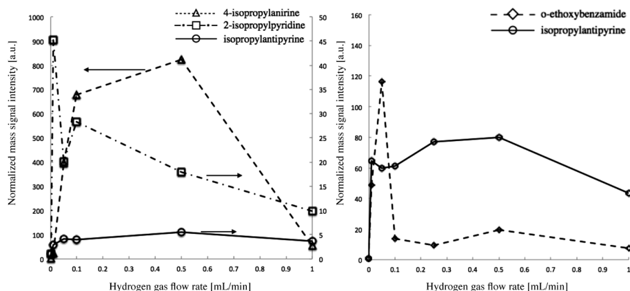
Fig. 9. (a) Relation between the hydrogen gas flow rate added to helium and normalized signal intensity in isopropylantipyrine, 2-isopropylpyridine, and 4-isopropylaniline, determined using an amazon-SL-AI ion trap mass spectrometer (MS1). The results were improved by 6, 45, and 824 times when the hydrogen gas was added to the helium base gas at flow rates of 0.5, 0.01, and 0.5 mL/min, respectively. (b) Relation between the hydrogen gas flow rate added to helium and normalized signal intensity in isopropylantipyrine and o -ethoxybenzamide, determined using the Agilent 1100 Series LC/MSD ion trap mass spectrometer (MS2). The results were improved by 80 and 117 times when the hydrogen gas was added to the helium base gas at flow rates of 0.5 and 0.05 mL/min, respectively.
