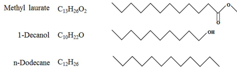
Figure 4- 1 Chemical structure of main fuel used in this chapter for a comparison study.
