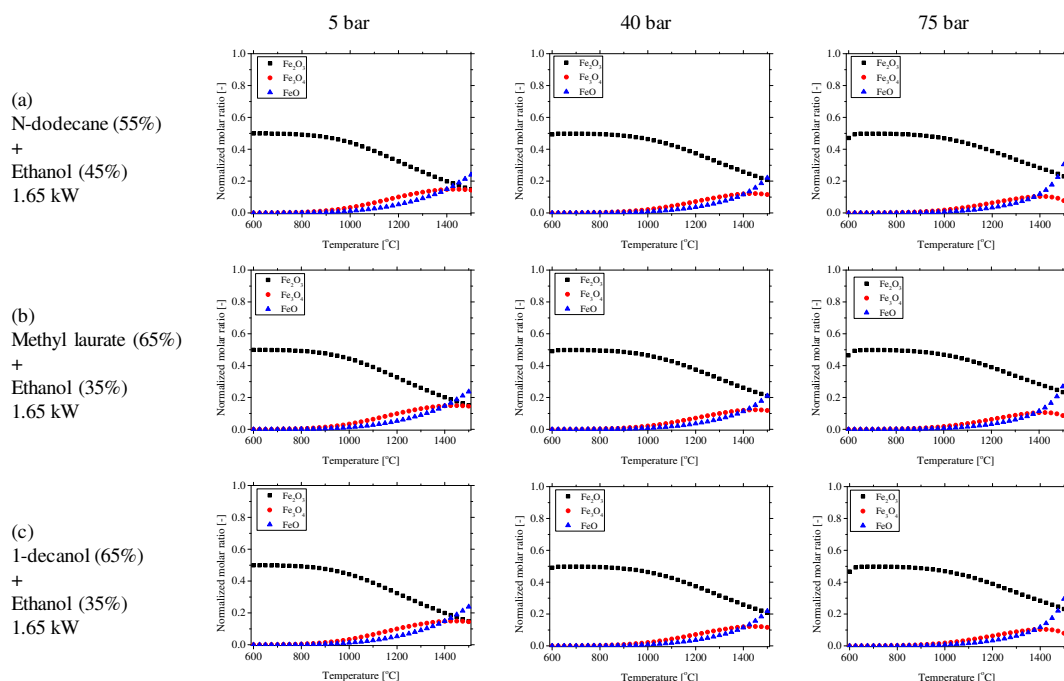
Figure S4- 6 Equilibrium calculations of chemical state of iron under different stating fuel and different pressures by means of Outokumpu HSC Chemistry for Windows (ver. 2.0). Dominant state of Fe in our experimental circumstances is oxidized one, being independent on pressure and fuel condition. Mean adiabatic combustion temperatures in our system are below 1,500 °C, and thus both \text{Fe}_2\text{O}_3 and FeO are mainly formed from the equilibrium point of view, being consistent with XPS analysis.
