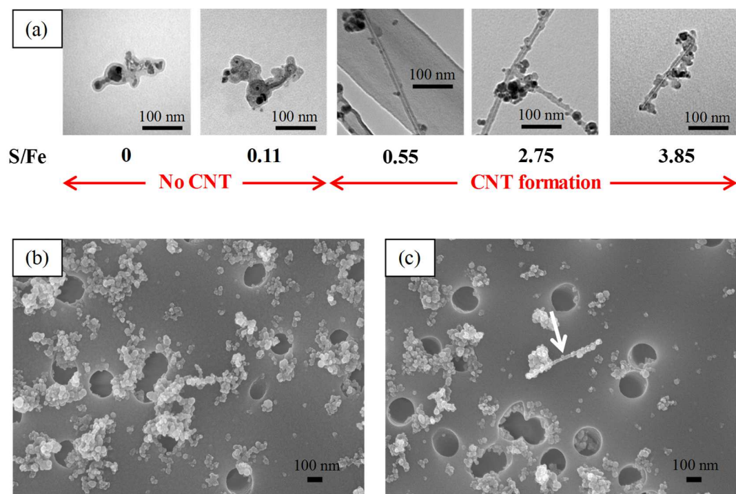
Figure 2- 5 (a) TEM images of synthesized carbon materials when the S/Fe ratio was varied from 0 to 3.85. SEM images (b) without sulfur (S/Fe = 0) and (c) with sulfur (S/Fe = 0.55) as a reference. Fuel condition was gas oil (80 volume%)/ethanol (20 volume%).
