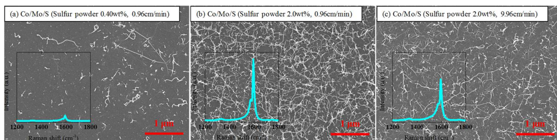
Figure 7- 2 SEM images after a CVD process at 800 °C for 30 minutes when sulfur amounts coated on a substrate were changed. Raman spectra were inserted in each SEM image. The images (a–c) were taken for a sample as a function of sulfur powder which dissolved in toluene. For the case (c), since the upper limit of sulfur powder which could dissolve in toluene was approximately 2.0 wt% in our work, a drawing speed from a toluene solution with 2.0 wt% of sulfur powder was increased from 0.96 cm/min to 9.96 cm/min, which was corresponding to sulfur amount of about 9.5 wt% in toluene on the basis of 0.96 cm/min as a drawing speed.
