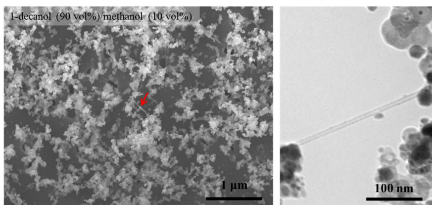
Figure S4- 3 SEM and corresponding TEM images when methanol is employed as an alternative of ethanol. Main fuel is 1-decanol and ferrocene concentration is 5,000 ppm by weight with Mo ( \text{Mo/Fe} = 0.01 ) and sulfur ( \text{S/Fe} = 2.2 ).
