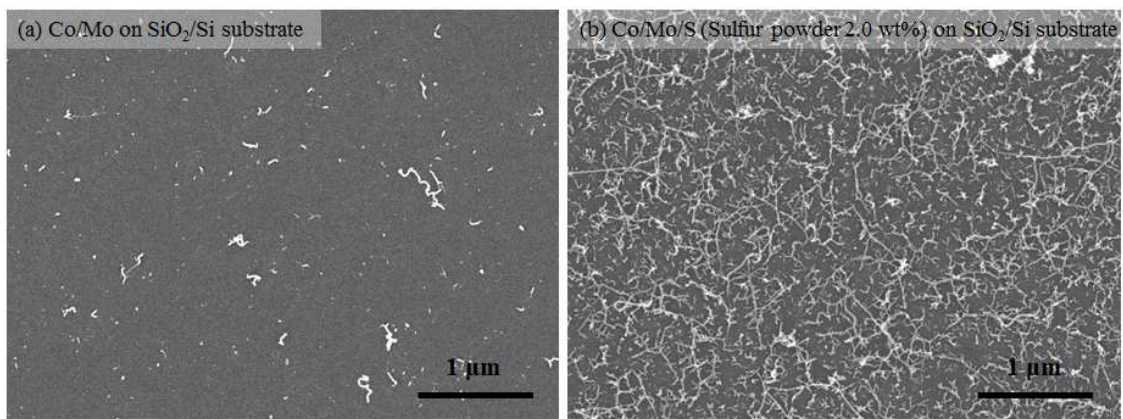
Figure S7- 3 SEM micrograph in the employment of SiO_2/Si substrate instead of quartz. (a) Co/Mo free from sulfur and (b) Co/Mo/S (Sulfur powder 2.0 wt%). CVD was performed at 800 °C for 30 minutes. It is obvious that the addition of sulfur is effective as well when SiO_2/Si substrate is used.
