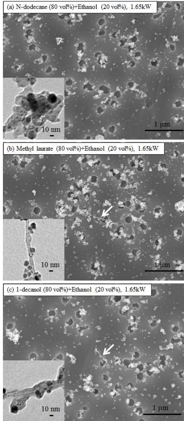
Figure 4- 5 Typical SEM images with inserted TEM images of synthesized CNTs when main fuel was varied while an ethanol fraction (20 volume %) and an engine load (1.65 kW) were identical. (a) n-dodecane (80 volume %)/ethanol (20 volume %) mixture, (b) methyl laurate (80 volume %)/ethanol (20 volume %) mixture and (c) 1-decanol (80 volume %)/ethanol (20 volume %) mixture. Synthesized CNTs are indicated by arrows in SEM images.
