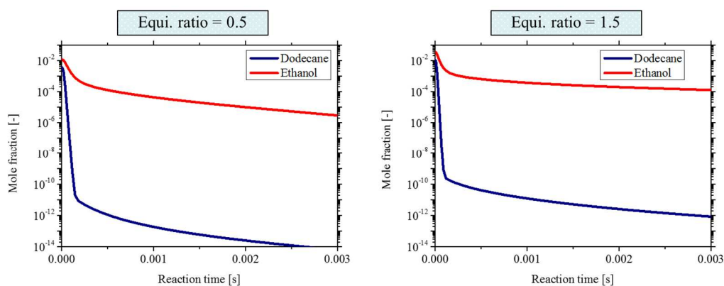
Figure S5- 3 The profile of normalized mole fraction of feedstock (n-dodecane/ethanol) simulated by CHEMKIN-PRO using a closed homogeneous reactor at 1250 K and 50 amt. Fuel condition was the mixture of n-dodecane (55 vol%) and ethanol (45 vol%). In both fuel rich/lean condition, consumption rate of n-dodecane is faster than that of ethanol, meaning that n-dodecane is easier to be oxidized.
