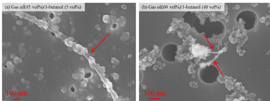
Figure S2- 1 SEM images when gas oil/1-butanol mixing fuel was used. A 1-butanol fraction in fuel was (a) 5 volume% and (b) 40 volume%. Ferrocene concentration was 10,000 ppm by weight, ratio of Mo/Fe was 0.01, and ratio of S/Fe was 0.55. An engine load was 1.05 kW. Observed CNTs are indicated by arrows. The formation of CNT was also confirmed when 1-butanol was used instead of ethanol.
