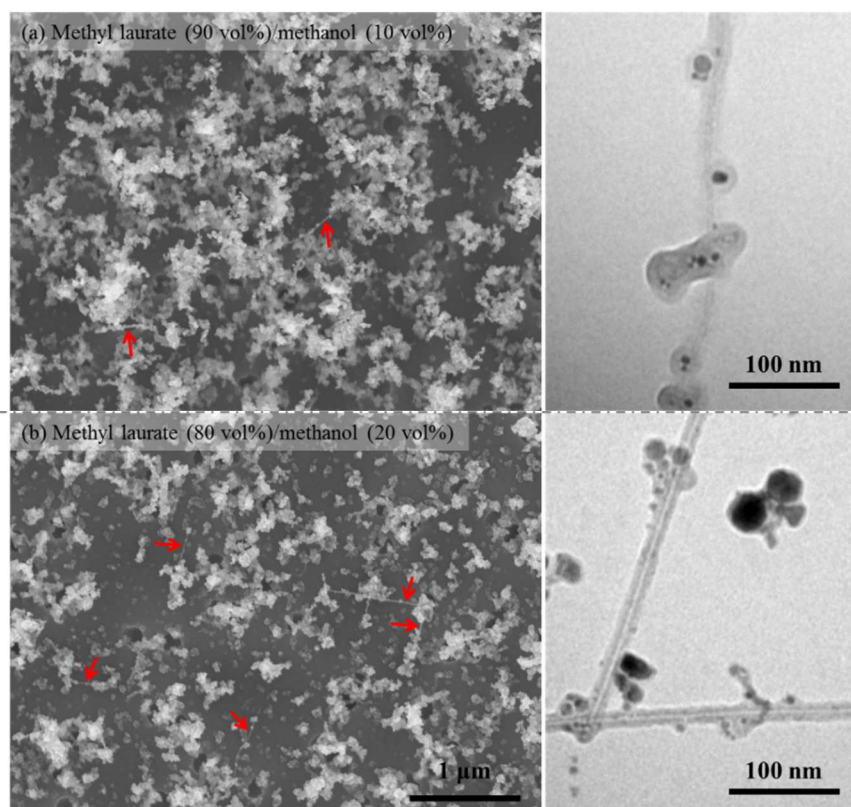
Figure S4- 2 SEM and corresponding TEM images when methanol is employed as an alternative of ethanol. Main fuel is methyl laurate and ferrocene concentration is 5,000 ppm by weight with Mo ( \text{Mo/Fe} = 0.01 ) and sulfur ( \text{S/Fe} = 2.2 ). An engine load is 1.65 kW. As a methanol content is increased, CNT production is also increased.
