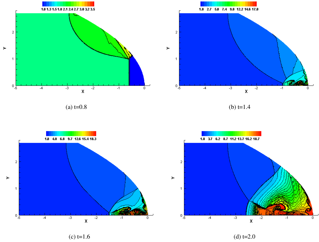
FIGURE 6.37: Temperature contours of the shock focusing problem with right-moving Mach 2.2 at different time
