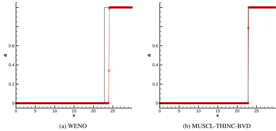
FIGURE 3.11: As for Fig. 3.8 but for mass fraction.
