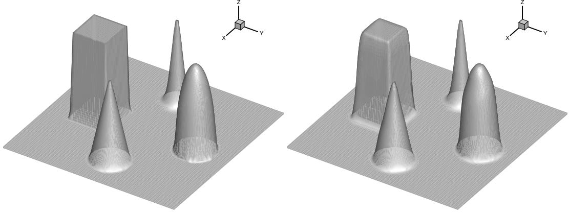
FIGURE 5.10: Numerical result of 2D rotation of complex wave after one period with 100 \times 100 cells. shown are initial profile (left panel) and numerical result (right panel).
