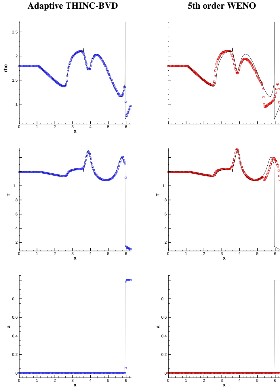
FIGURE 3.37: Numerical results of density, temperature and mass fraction fields for C-J detonation wave with the Heaviside chemical reaction model for the interaction between a detonation wave and an oscillatory profile problem. Reference solutions are represented by black solid lines. Comparisons are made between the WENO (right panels) and the proposed scheme (left panels).
