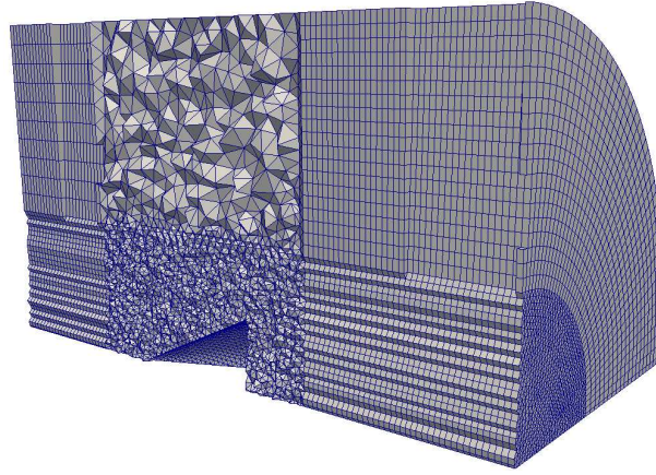
FIGURE 6.41: A view of the hybrid unstructured grid used for the computation of the shock-cone interaction test.
