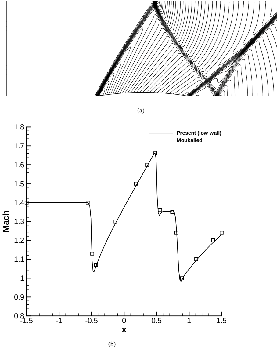
FIGURE 6.29: The Mach number contours for supersonic bump flow at steady state on 158 \times 78 quadrilateral elements (a), and the plot of the Mach number along the lower wall in comparison with the results from [215] (b).
