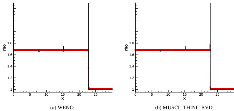
FIGURE 3.12: As for Fig. 3.10 but with finer mesh.
