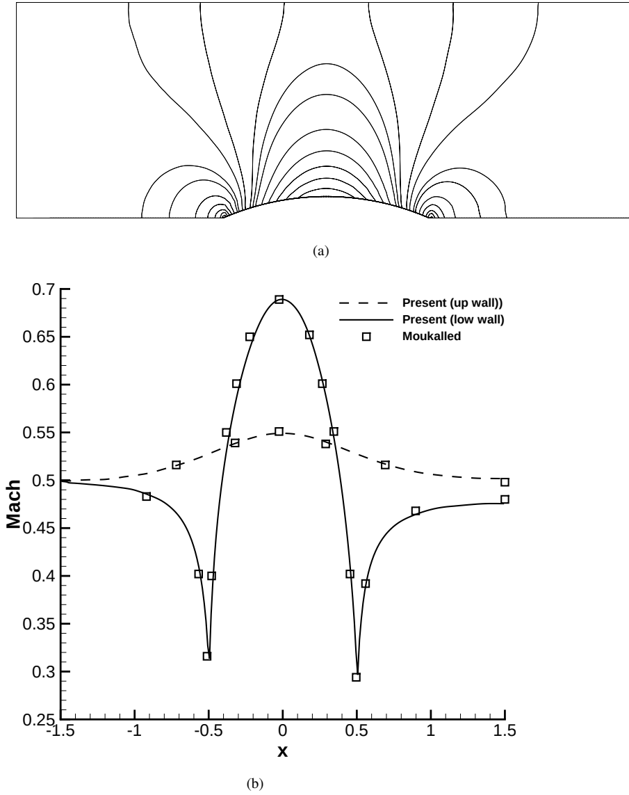
FIGURE 6.31: Same as Fig. 6.29, but for subsonic flow regime.
