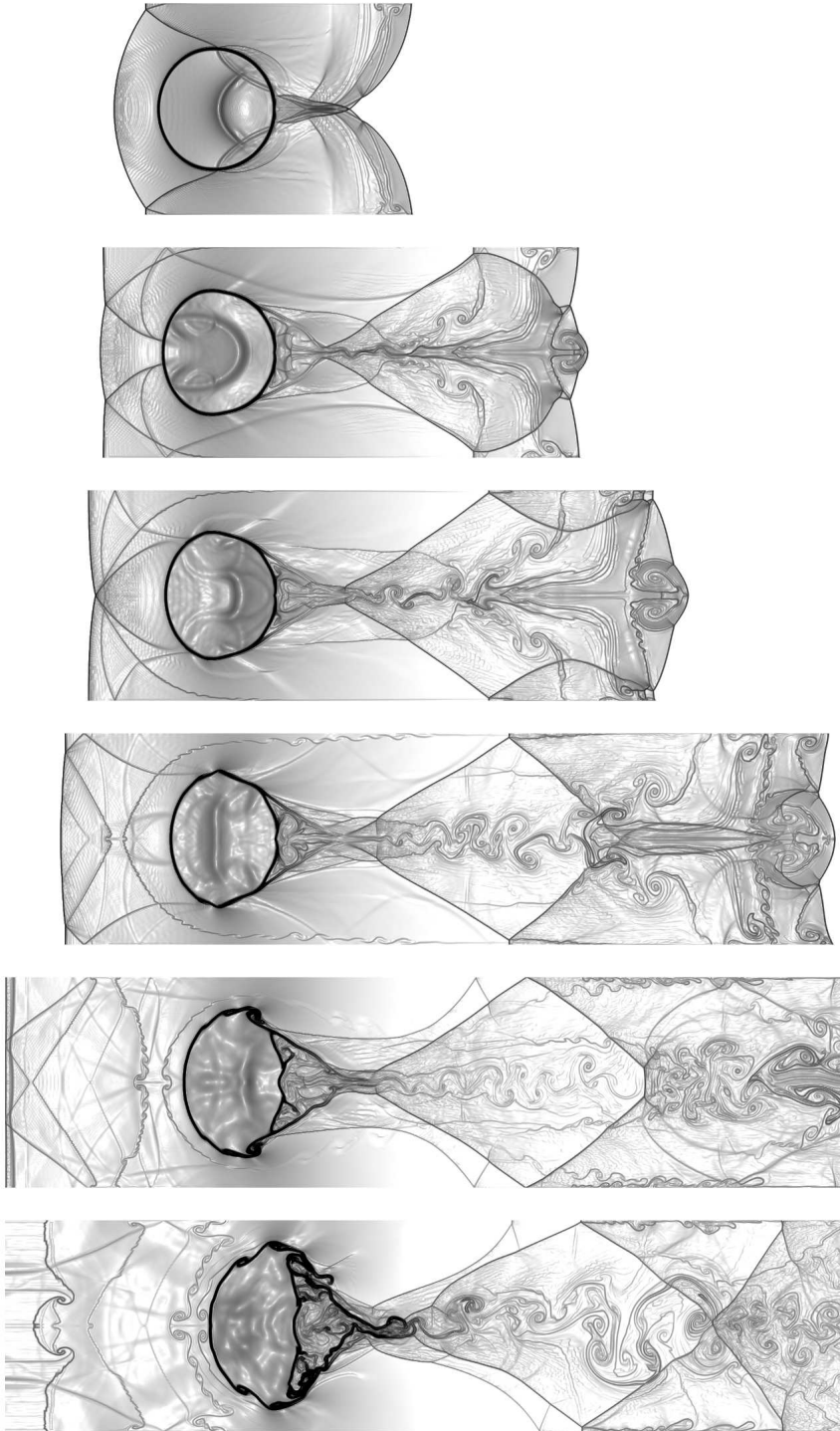
FIGURE 4.13: Schlieren images of density fields for the Mach 6.0 shock-water interaction benchmark test at instants t = 0.5, 0.75, 0.89, 1.1, 1.5 , and 2.15 solved by the MUSCL-THINC-BVD scheme on a 2000 \times 500 uniform grid.
