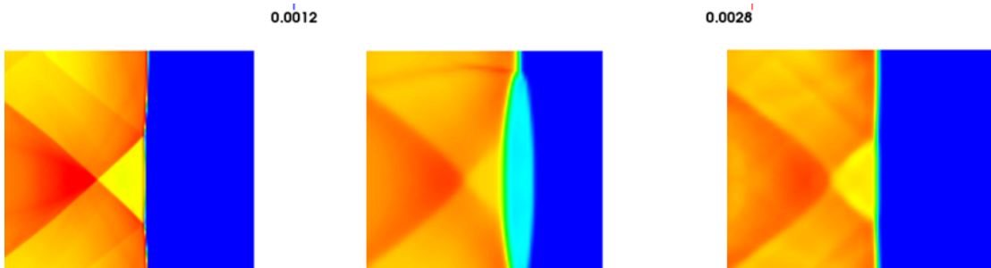
FIGURE 3.30: As for Fig. 3.28 but at t = 1.7 \times 10^{-7} .
