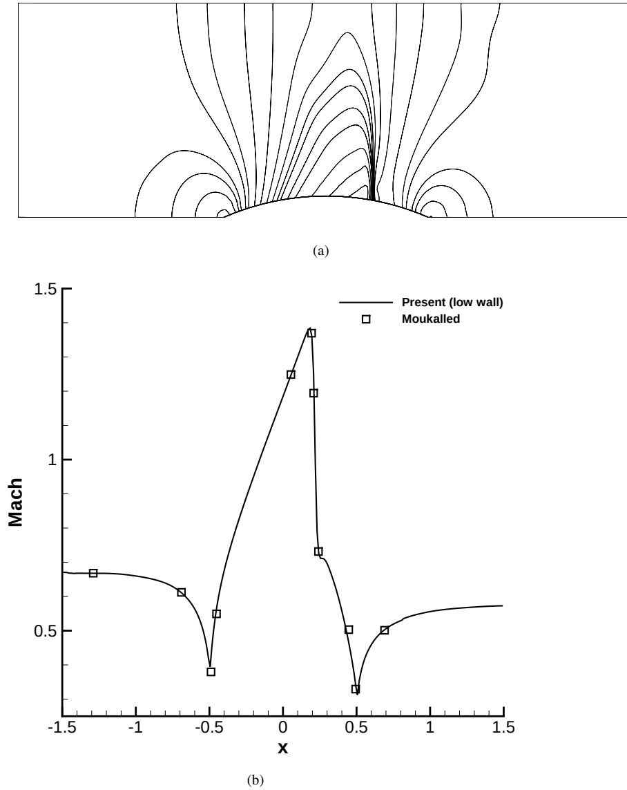
FIGURE 6.30: Same as Fig. 6.29, but for transonic flow regime.
