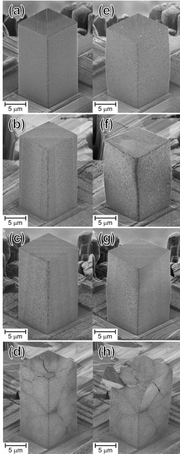
FIG. 3.4. SIM images of the Au-Cu alloy micro-pillars (a–d) before and (e–h) after the micro-compression tests. The micro-pillars were fabricated from the films electroplated at current density = (a, e) 3, (b, f) 5, (c, g) 6, and (d, h) 8 mA/cm 2 .
