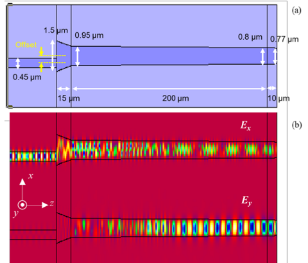
Fig. 2. (a) Structure of the tapered half mode converter.
