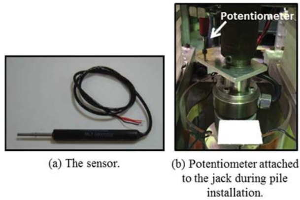
Figure 3.15. Potentiometer.
