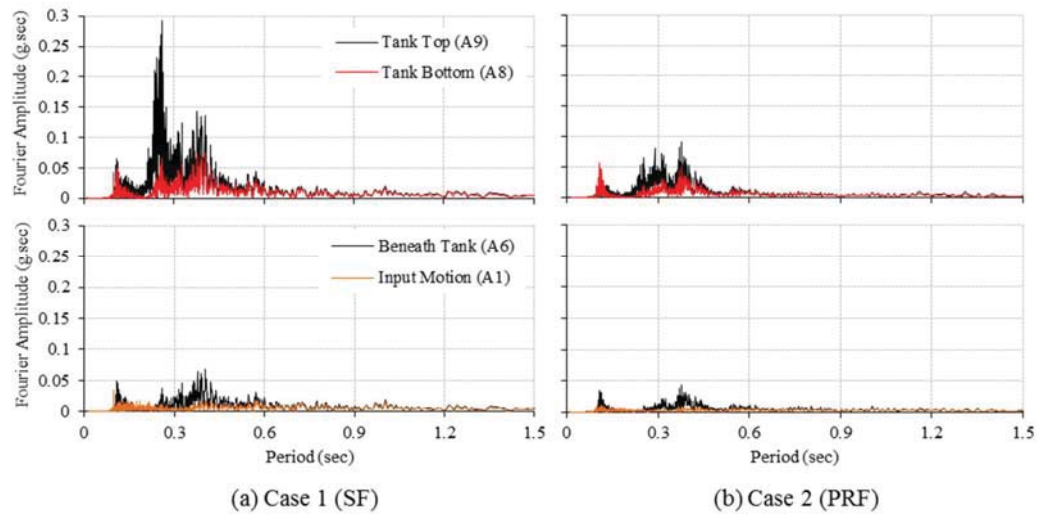
Figure 04.5. Ground and tank responses during White noise (Dry sand).
