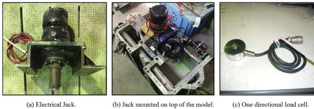
Figure 3.16. Electrical Jack and load cell.
