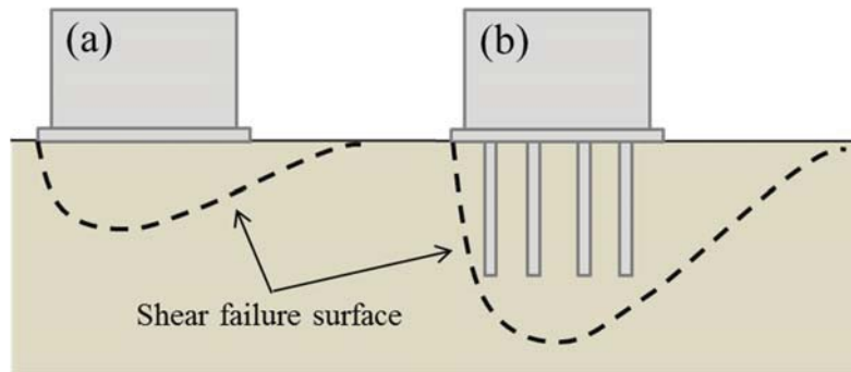
Figure 5.7. Shear failure surface, (a) Raft foundation, (b) Piled raft foundation.
