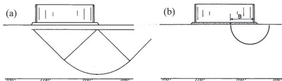
Figure 5.6. Tank stability failure mechanism, (a) Base shear failure, (b) Edge shear failure (Duncan et al., 1984)
