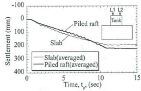
(d) Tank settlement during shaking.
