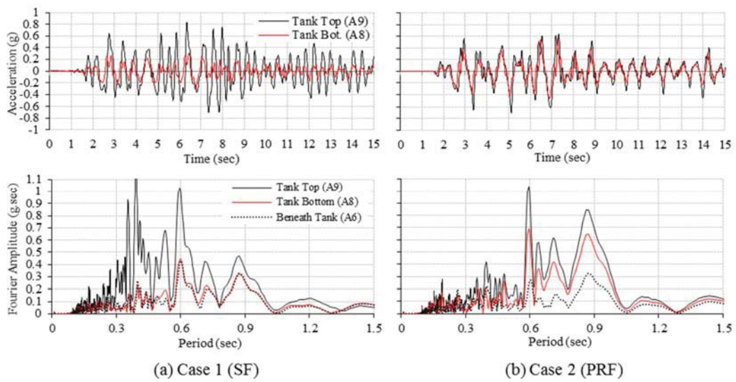
Figure 4.4. Tank responses in Shake 1 (Dry sand).
