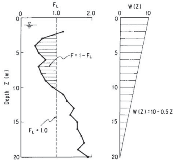
Figure 5.10. Example of F_L value and weight function w(z) (Iwasaki, 1986).
