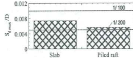
(b) Normalized differential settlement.
