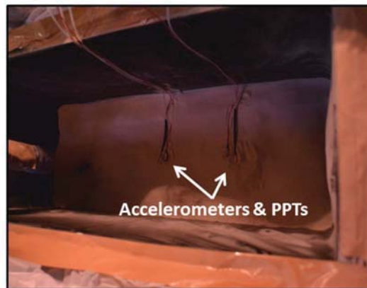
(c) Model ground sensors during sand pouring.
