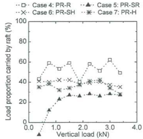
Figure 2.10 (d). Vertical load vs load proportion relationship (Matsumoto et al., 2010).
