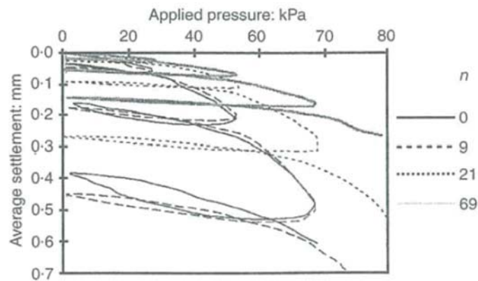
Figure 2.13 (a). Average settlement of tank during loading test ( n =piles number) (Horikoshi et al., 1996).
