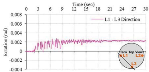
(b) Case 2 (PRF)
