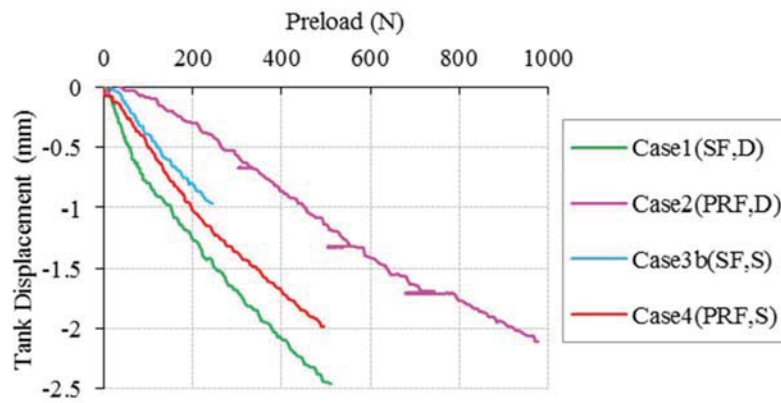
Figure 3.31. Exerted loads during preloading process.
