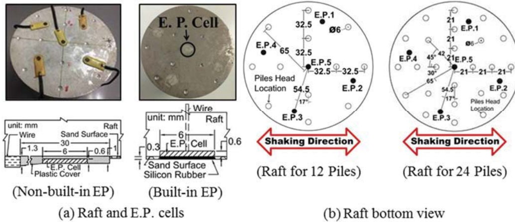
Figure 3.4. Raft model.
