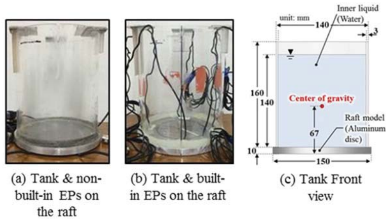
Figure 3.3. Tank model.
