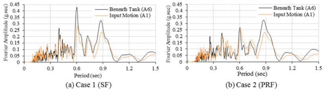
Figure 4.3. Ground responses in Shake 1 (Dry sand).
