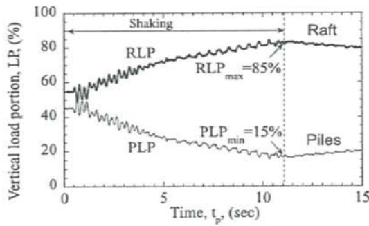
(c) Variation of vertical load portion during shaking.
