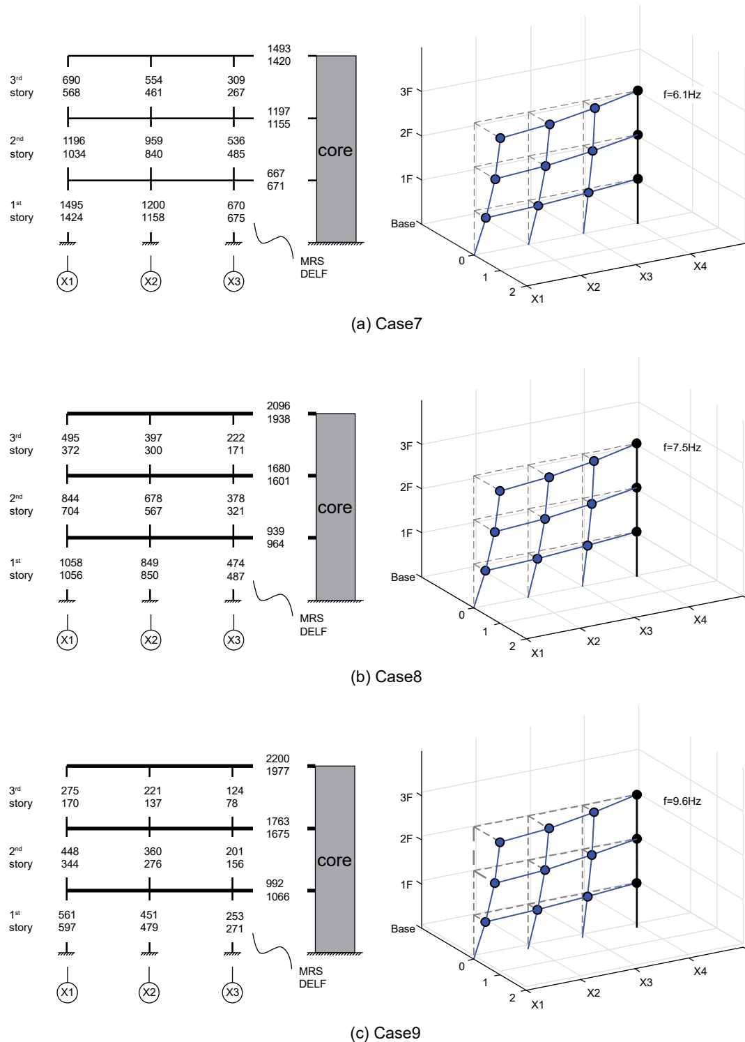
Fig. 5.8 Peak shear force of the shear wall and diaphragm by DELF and MRS, PGA=0.1g, unit:N, (a) Case7, \delta=1 , (b) Case8, \delta=2 , (c) Case9, \delta=4
