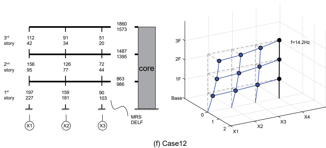
Fig. 5.8 Peak shear force of the shear wall and diaphragm by DELF and MRS, PGA=0.1g, unit:N, (d) Case10, \delta=6 , (e) Case11, \delta=8 , (f) Case12, \delta=10
