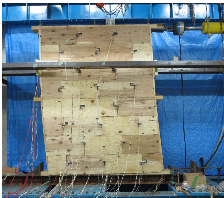
Fig. B.8 Deformation pattern of the specimen D100 at the drift of 1/10 rad
