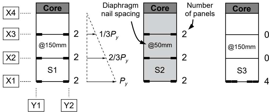
Fig. C.1 Configuration of specimens and distribution of design base shear force in S1
