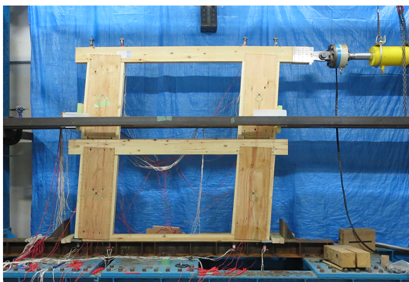
Fig. B.6 Deformation pattern of the specimen 2S2W at the drift of 1/15 rad
