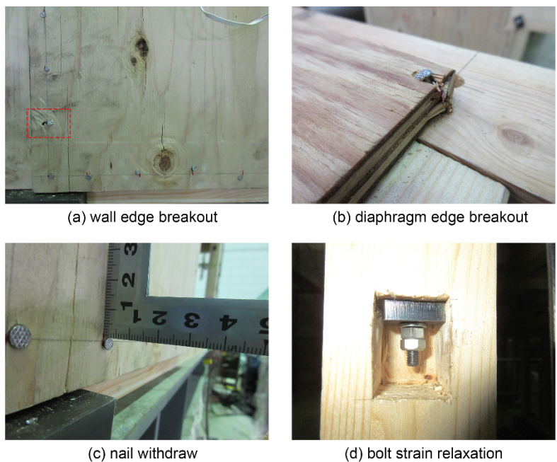
Fig. 2.3 Failure mode observed of the nail and the beam-column joint after input of 0.8g
