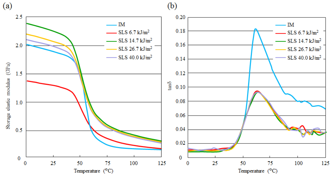
Fig. 12: DMA results for IM specimen and SLS specimens under assumed laser energy densities of 6.7, 14.7, 26.7, and 40.0 kJ/m 2 : (a) storage elastic modulus and (b) \tan \delta .
