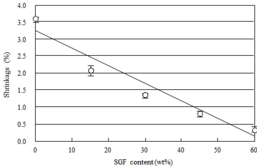
Fig. 14: Comparison of shrinkage of cPBT, cPBT/15-wt%-SGF, cPBT/30-wt%-SGF, cPBT/45-wt%-SGF, and cPBT/60-wt%-SGF specimens.
