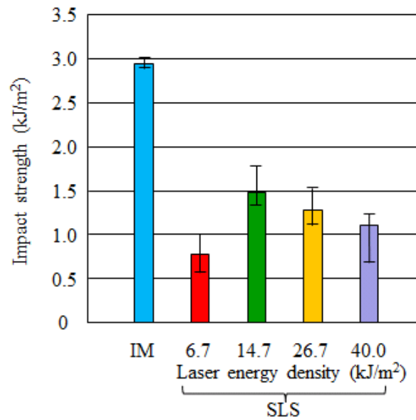
Fig. 11: Comparison of Charpy impact strength of IM specimen and SLS specimens under assumed laser-energy densities of 6.7, 14.7, 26.7, and 40.0 kJ/m².
