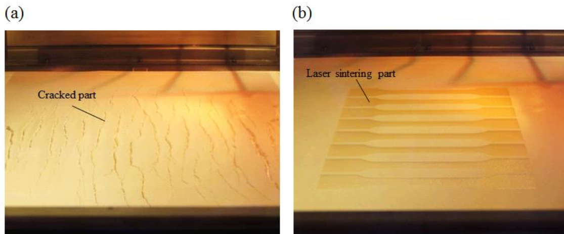
Fig. 8: External appearance of the powder bed during SLS processing: powder-bed temperature (a) 193 °C and (b) 190 °C.
