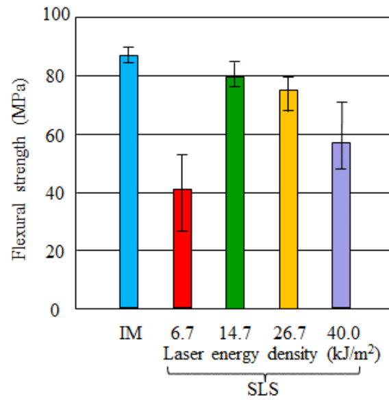
Fig. 10: Comparison of flexural strength of IM specimen and SLS specimens under assumed laser-energy densities of 6.7, 14.7, 26.7, and 40.0 kJ/m².
