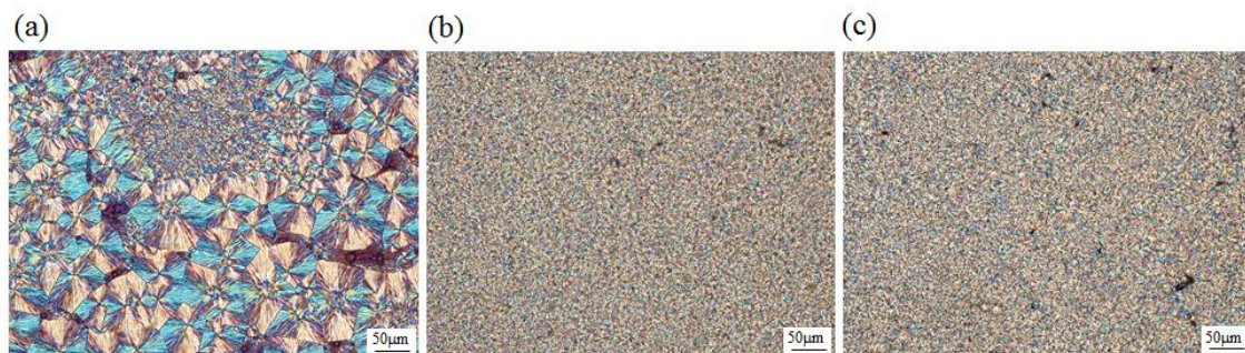
Fig. 7: Polarization-microscope images of pellets and powder obtained at RT after temperature crystallization at 190 °C for 60 min: (a) pellets and (b) powder (c) powder with 0.1-wt% addition of fumed silica.
