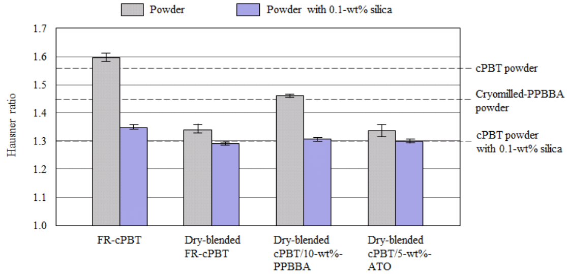
Fig. 3: Comparison of HR of FR-cPBT powder, dry-blended FR-cPBT powder, dry-blended cPBT/10-wt%-PPBBA powder, and dry-blended cPBT/5-wt%-ATO powder with or without 0.1-wt% added silica.
