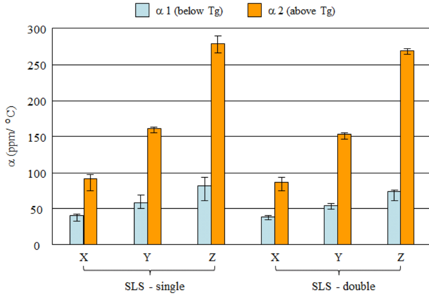
Fig. 14: Comparison of linear-expansion coefficient below and above glass-transition temperature ( T_g ) of SLS specimens formed with single- and double-scan methods and arranged in the X-, Y-, and Z-build directions.
