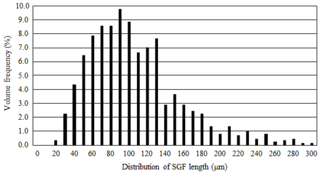
Fig. 1: Distribution of SGF length.
