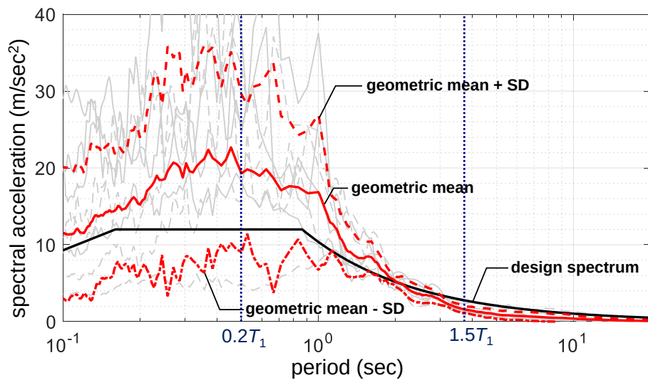
Figure 4.5.7 Spectra of the scaled ground motions used for 32-story Single and SingleElastic models in NLRHA (SD = standard deviation)
