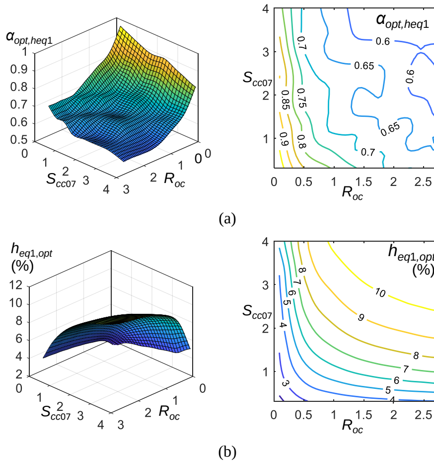
Figure 9.4.2 The (a) \alpha_{opt,heq1} and (b) h_{eq1,opt} distributions with respect to S_{cc07} and R_{oc}
