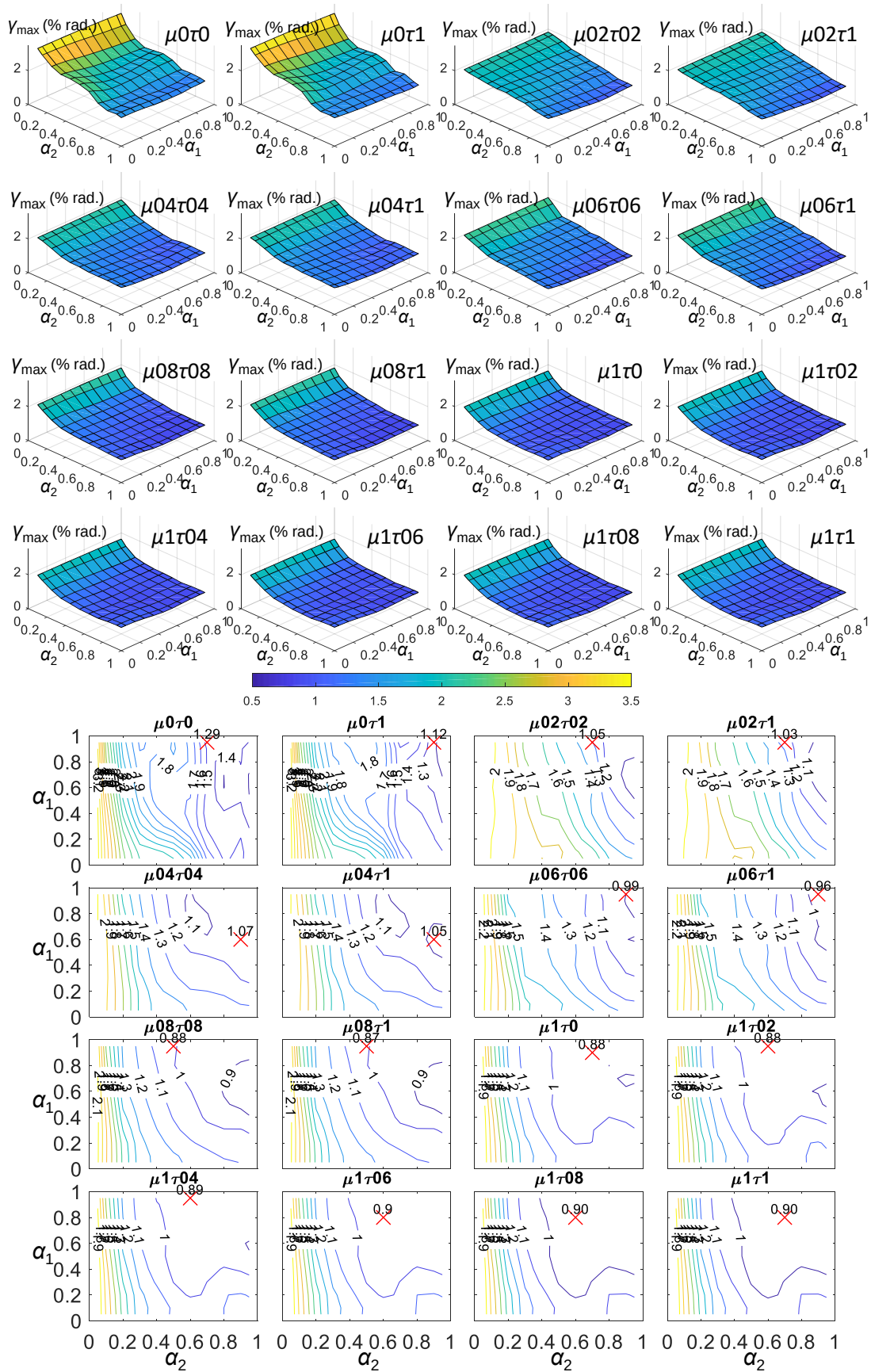
Figure 10.3.12 The \gamma_{\max} of the 40-story dual BRB-outrigger example model calculated from the NLHRA with BCJ-L2 ground motion (unit: % rad.)
