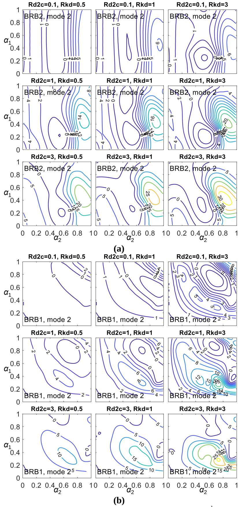
Figure 6.4.10 The (a) E_{d2}/E_s and (b) E_{d1}/E_s distributions of the 2 nd mode response under different BRB yield cases and \theta_r
