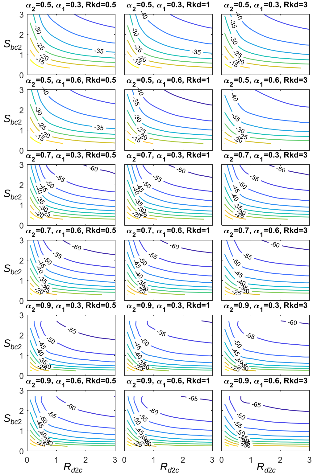
Figure 7.3.17 The \gamma_{\max} reduction factor distributions with various R_{d2c} and S_{bc2}
