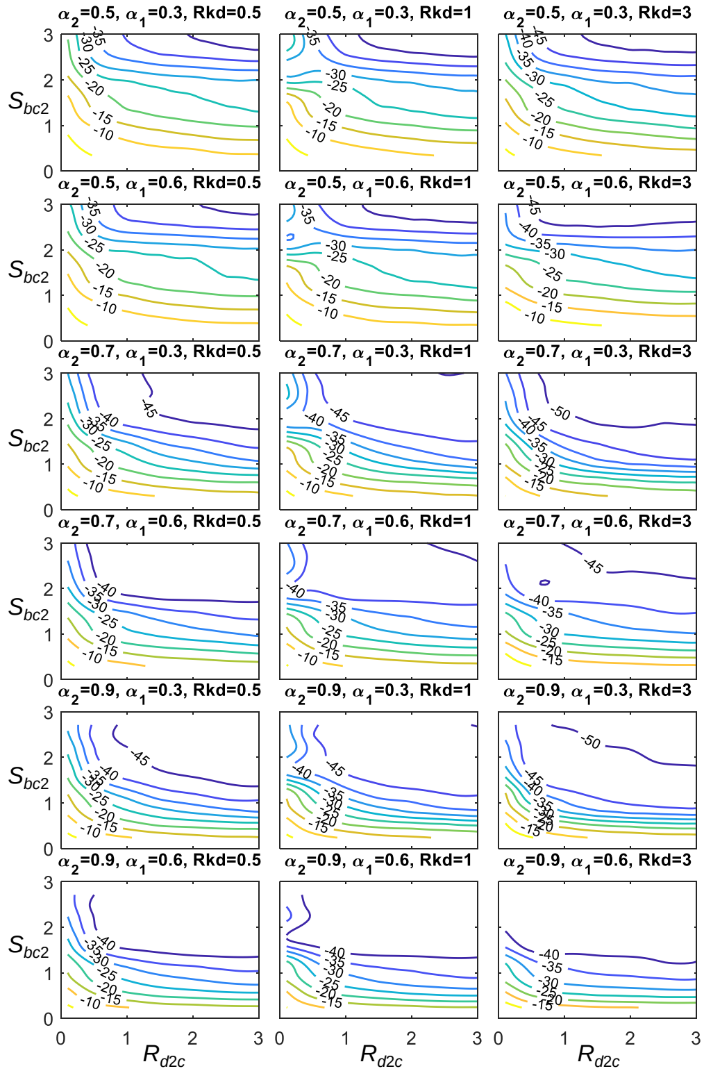
Figure 7.3.25 The M_{c,max} reduction factor distributions with various R_{d2c} and S_{bc2}
