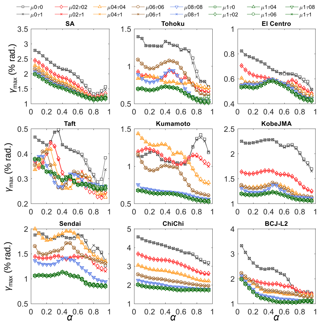
Figure 10.3.4 Relationship between \gamma_{\max} and \alpha of the 40-story single BRB-outtrigger example model with various \mu and \tau values
