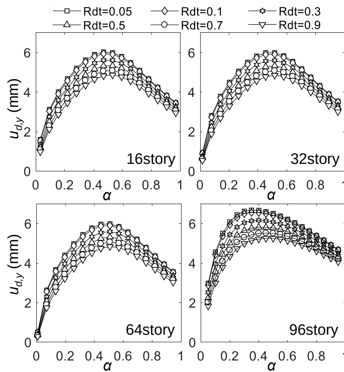
Figure 6.3.7 Relationship between u_{d,y} and \alpha for different R_{dt}
