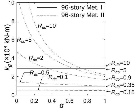
Figure 3.4.8 Relationships between k_g and \alpha of 96-story model
