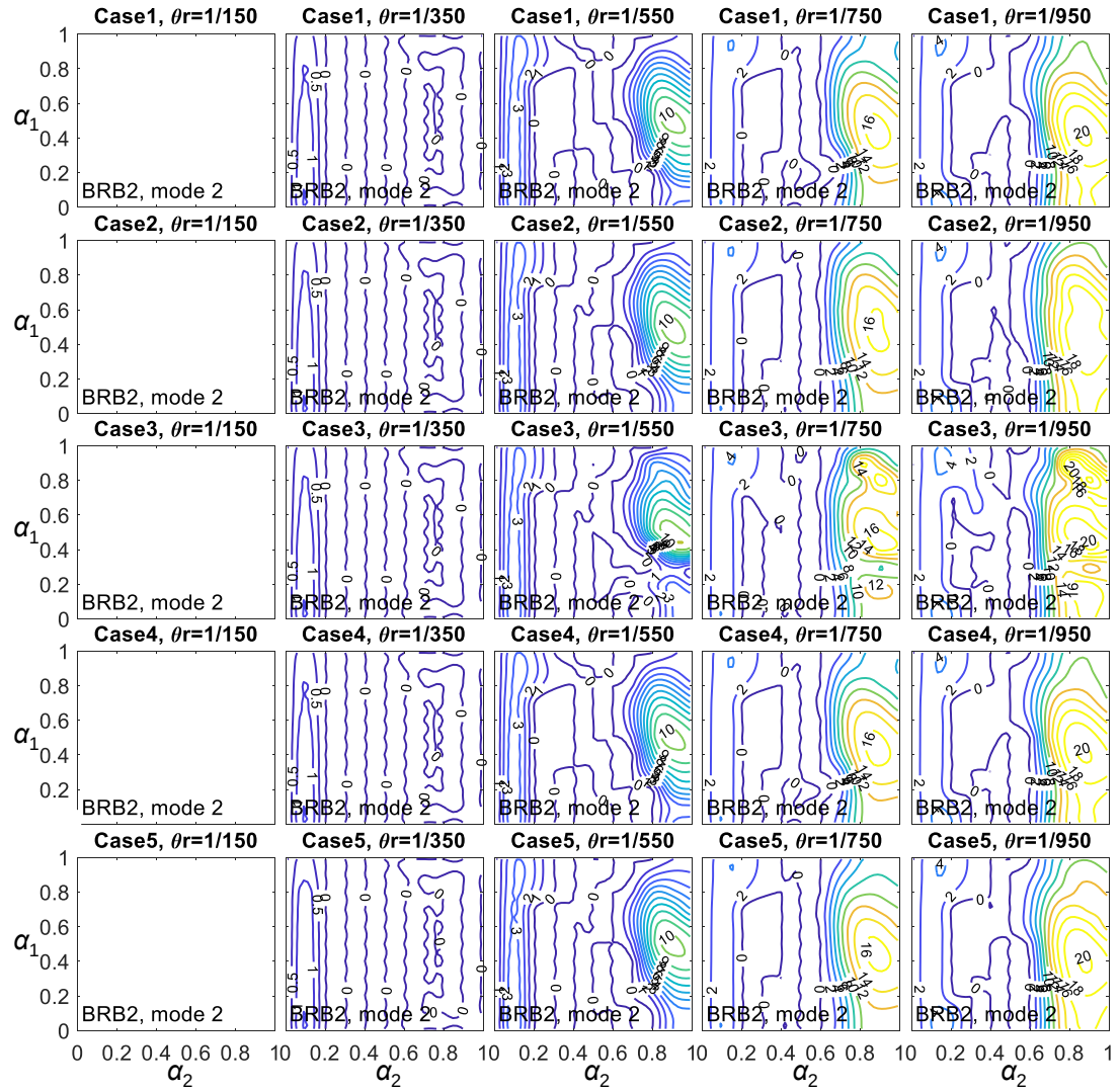
Figure 6.4.5 The E_{d2}/E_s distributions of the 2 nd mode response under different BRB yield cases and \theta_r
