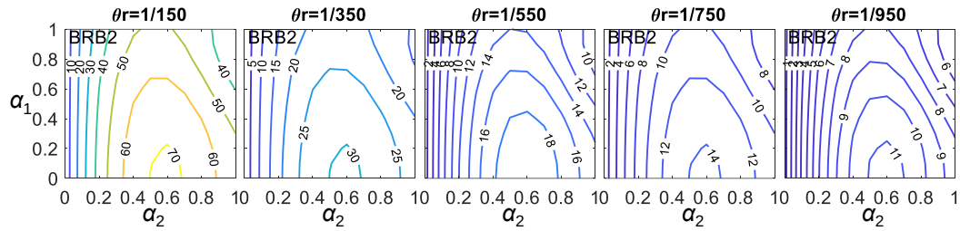
Figure 6.4.1 The u_{d,y2} under different yield cases and \theta_r (unit: mm)
