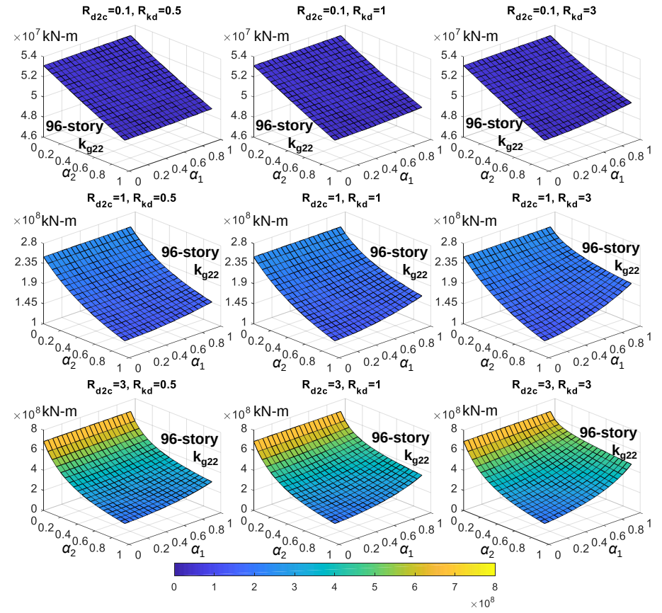
Figure 3.4.16 Relationships between k_{g22} and outrigger elevations for the 96-story dual BRB-outrigger model
