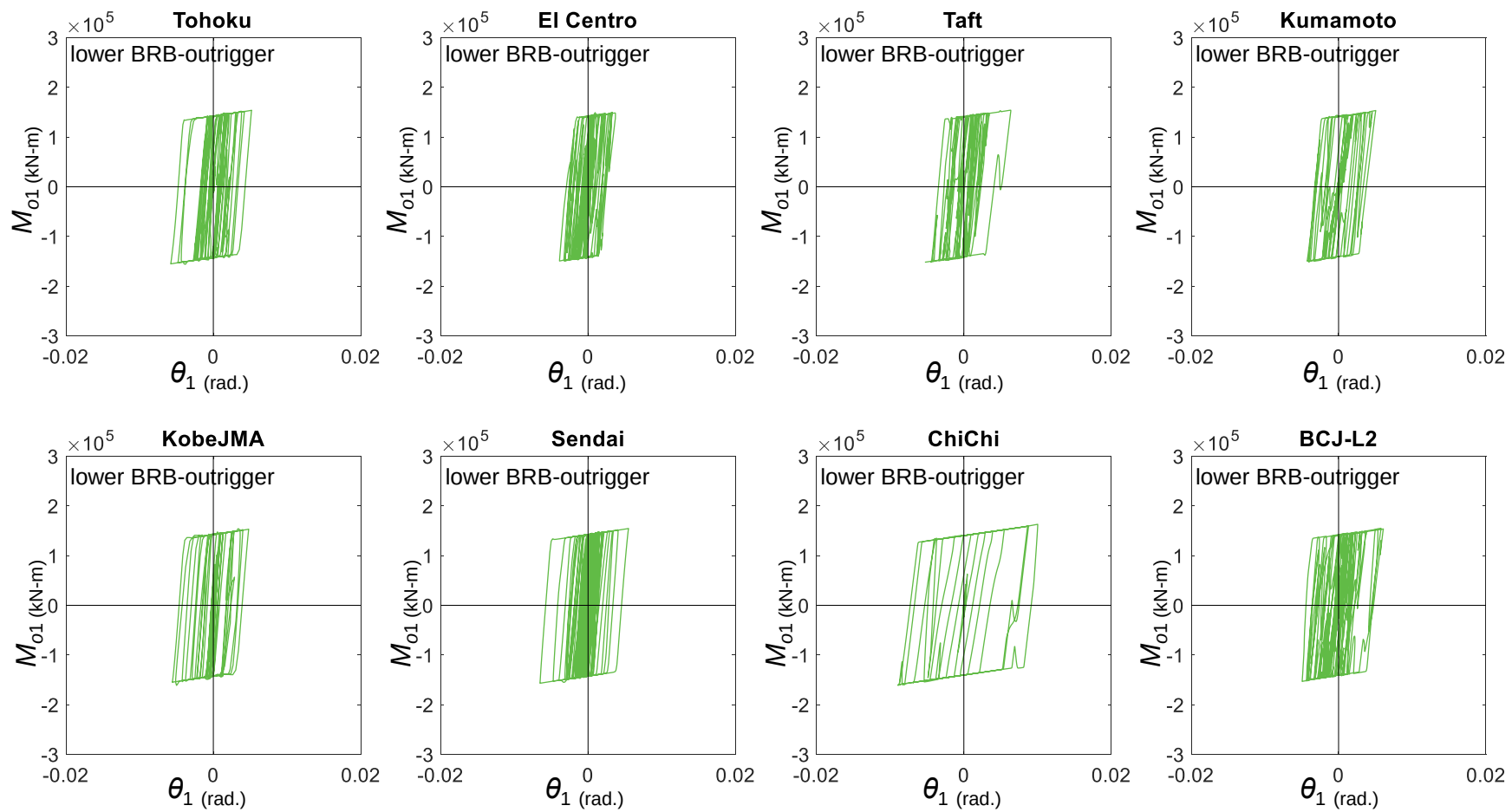
Figure 4.5.32 The relationship between M_{o1} and \theta_1 for the 96-story Dual model
