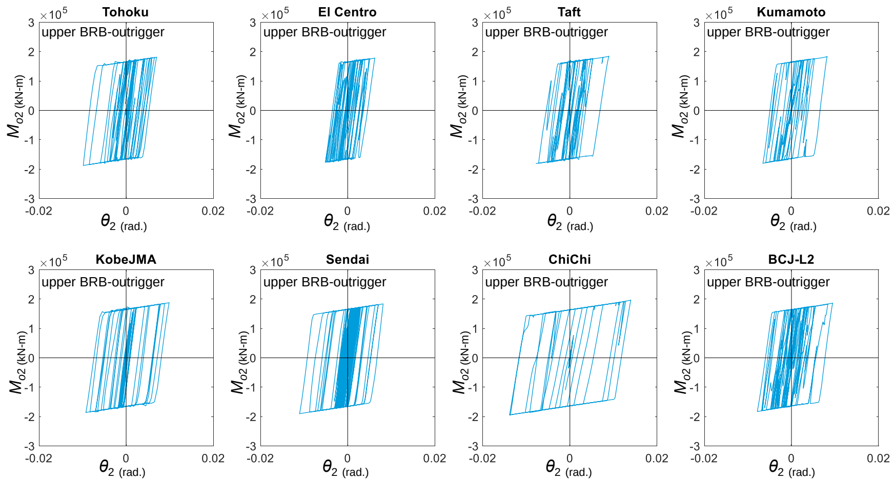
Figure 4.5.31 The relationship between M_{o2} and \theta_2 for the 96-story Dual model
