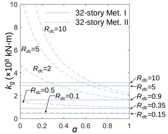
Figure 3.4.6 Relationships between k_g and \alpha of 32-story model
