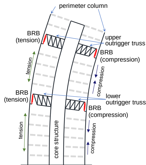
Figure 1.3.2 The laterally deformed structure with two layers of BRB-outrigger
