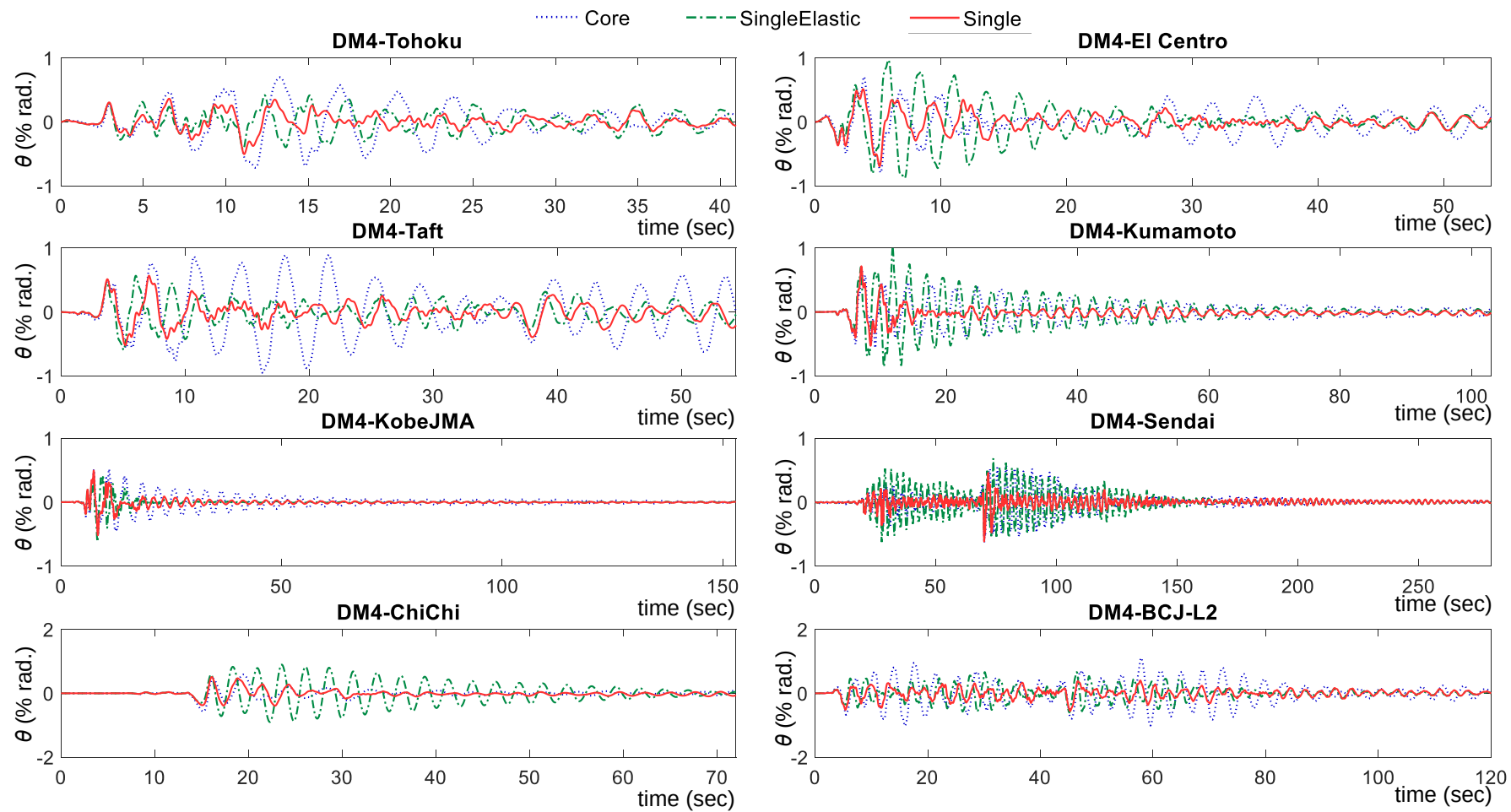
Figure 4.5.9 The roof drift history of the 32-story example model under different ground motions from NLRHA using DM4 models
