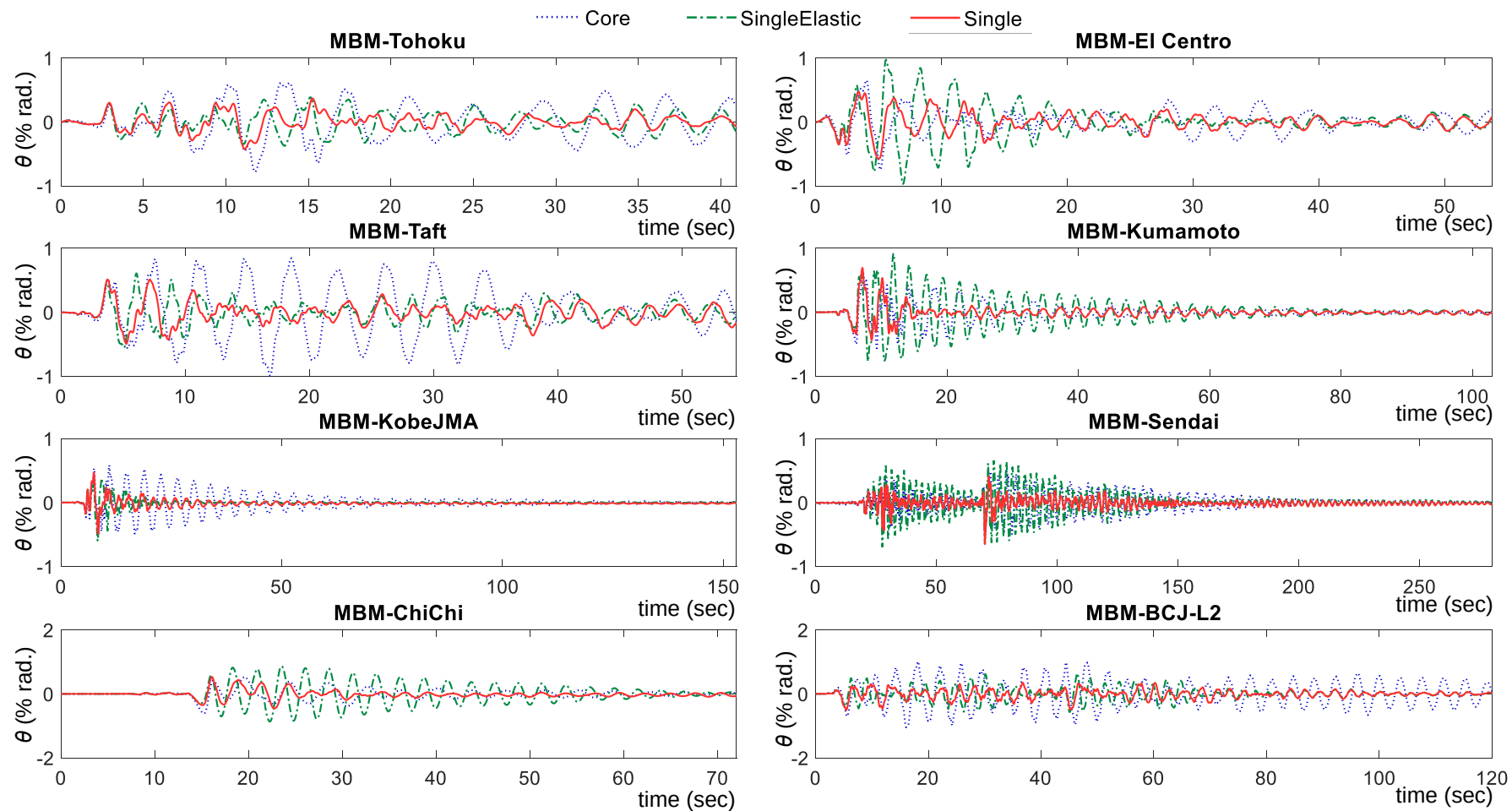
Figure 4.5.10 The roof drift history of the 32-story example model under different ground motions from NLRHA using MBM models
