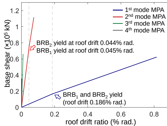
Figure 4.5.34 The MPA curves of the 96-story Dual model
