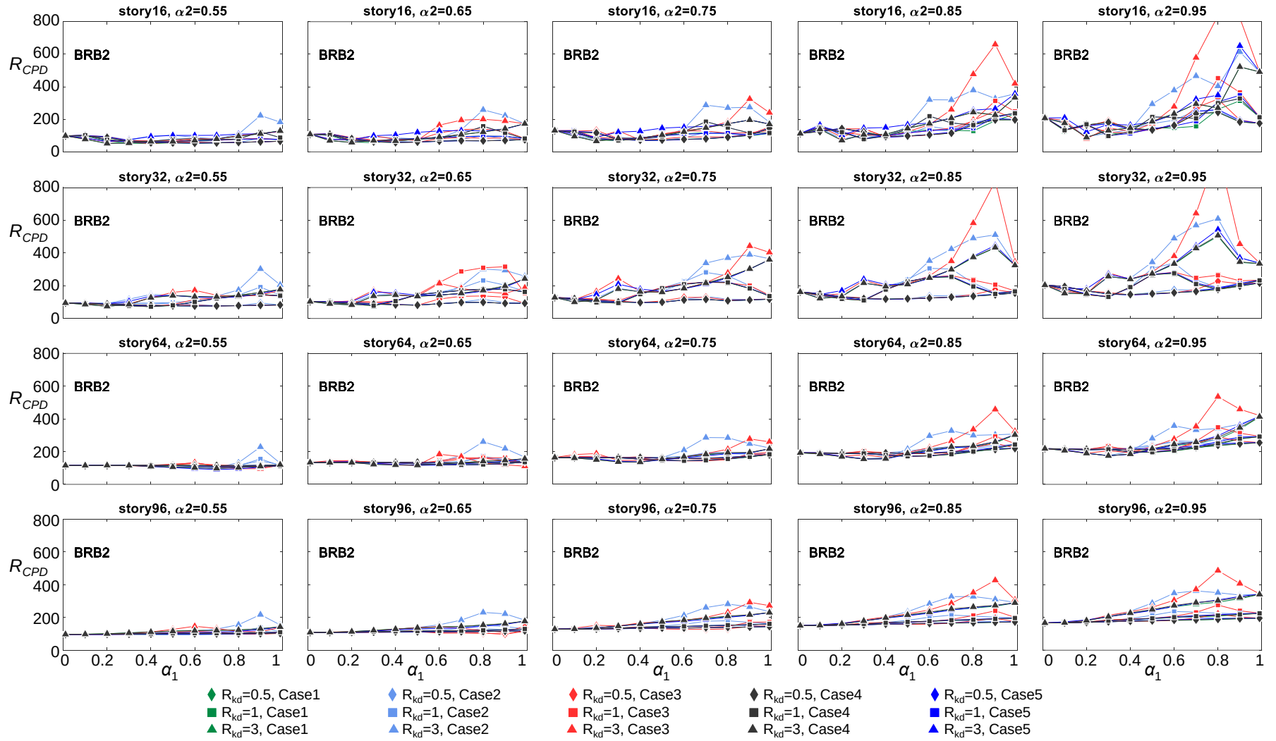
Figure 6.3.17 R_{CPD} ratio of BRB_2 calculated from NLRHA
