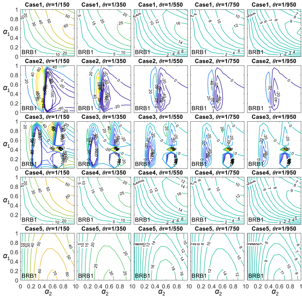
Figure 6.4.2 The u_{d,y1} under different yield cases and \theta_r (unit: mm)
