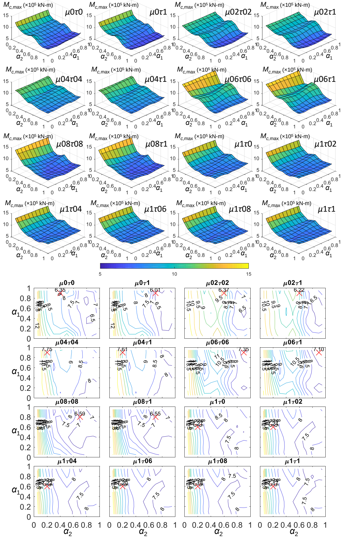
Figure 10.3.13 The M_{c,max} of the 40-story dual BRB-outrigger example model calculated from the NLHRA with BCJ-L2 ground motion (unit: \times 10^5 kN-m)
