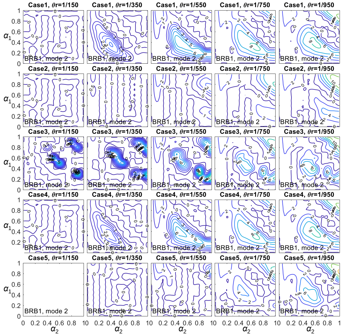
Figure 6.4.6 The E_{d1}/E_s distributions of the 2 nd mode response under different BRB yield cases and \theta_r
