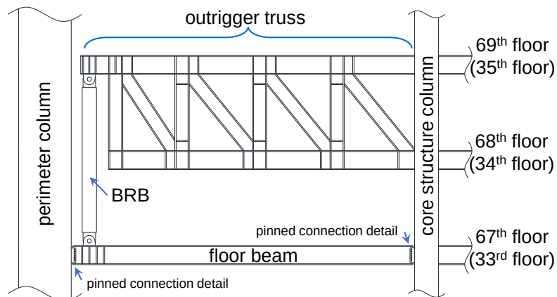
Figure 3.5.6 Enlargement of the BRB-outrigger detail in the 96-story MBM model
