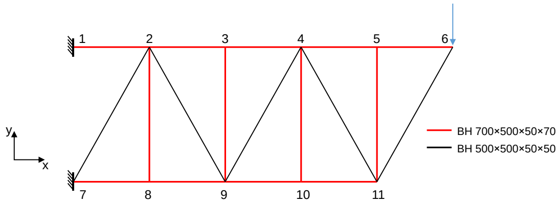
Figure 8.2.4 Analytical model of the outrigger truss
