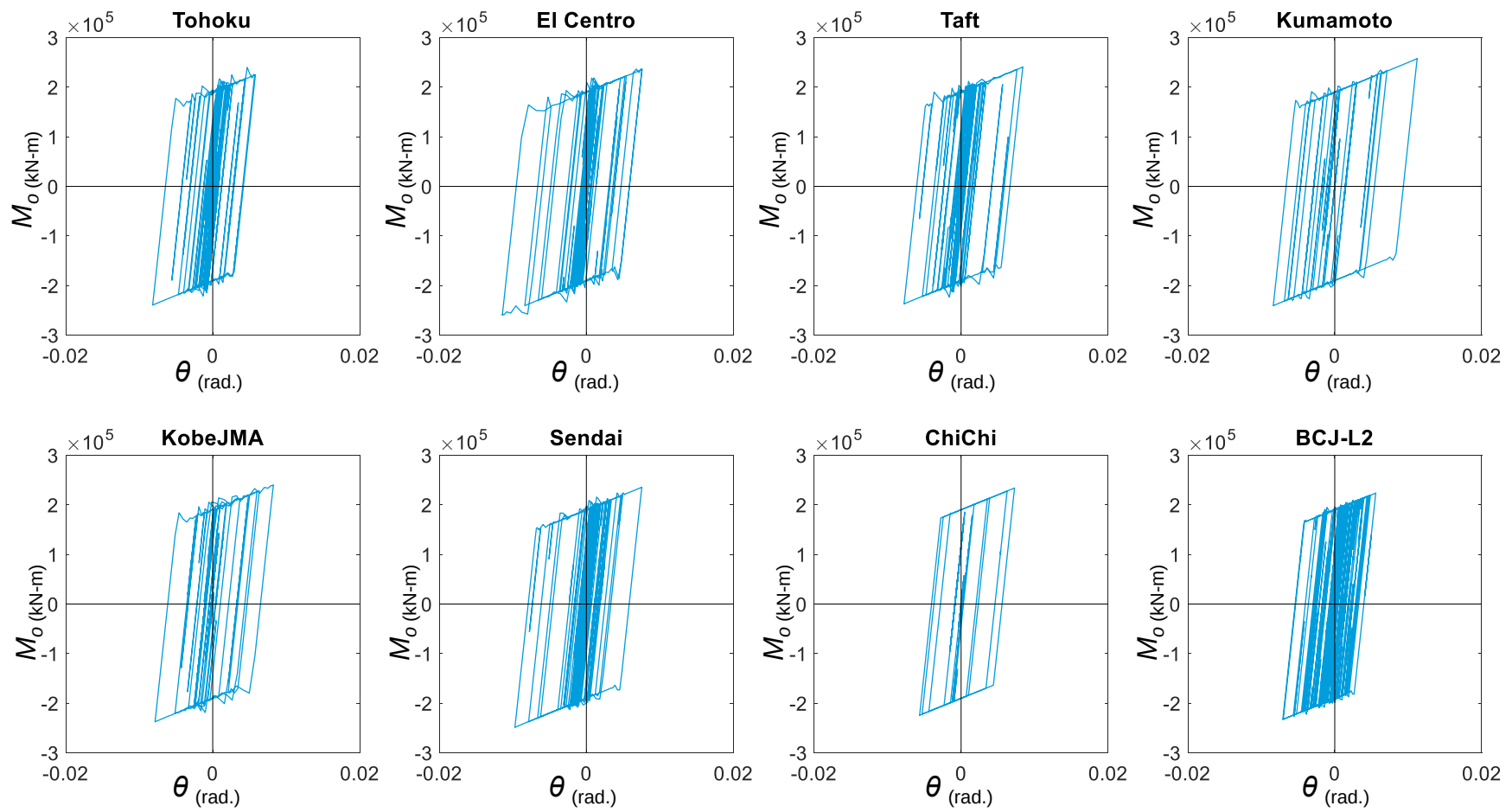
Figure 4.5.17 The relationship between M_o and \theta for the 32-story Single model
