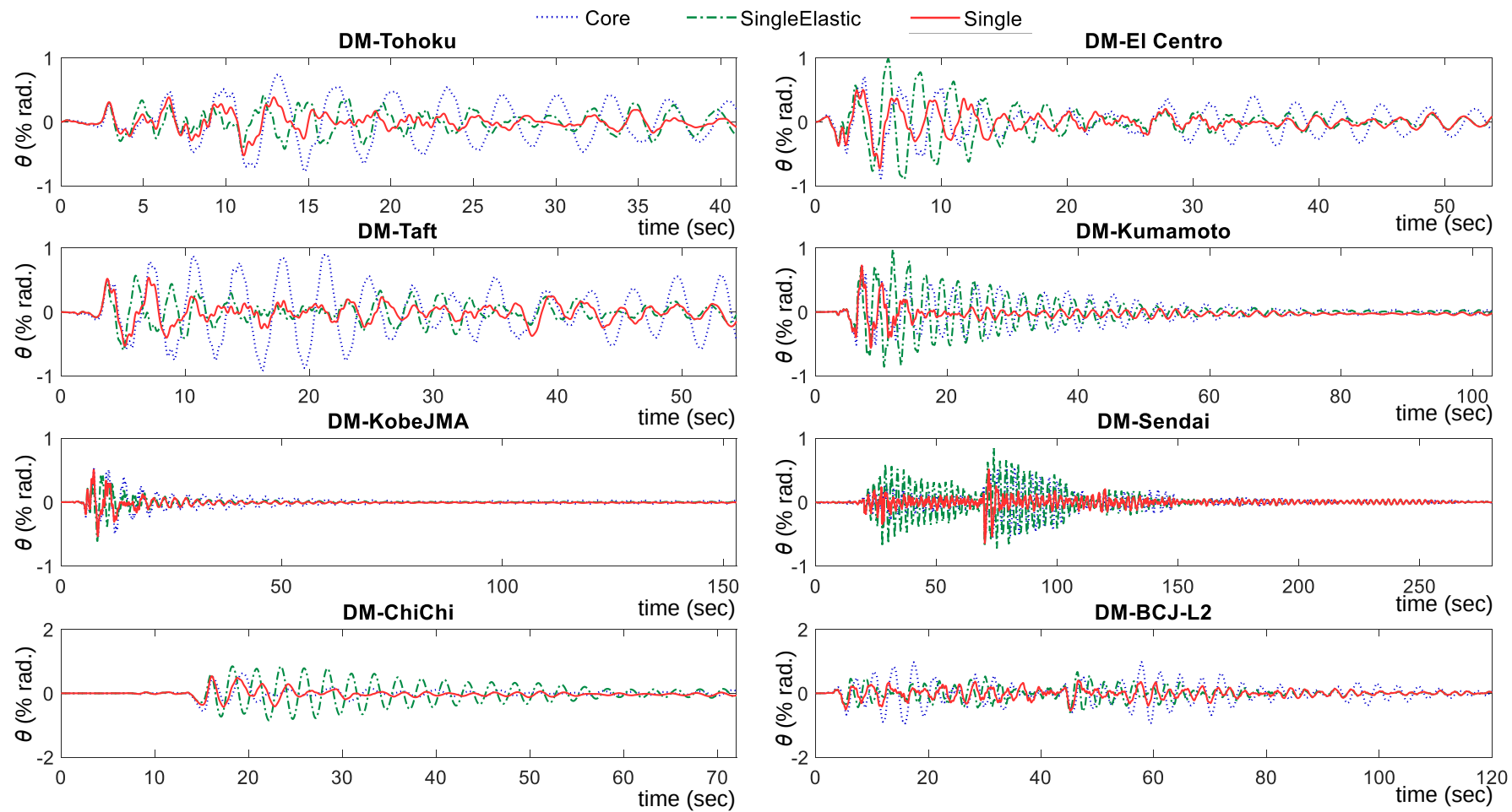
Figure 4.5.8 The roof drift history of the 32-story example model under different ground motions from NLRHA using DM models
