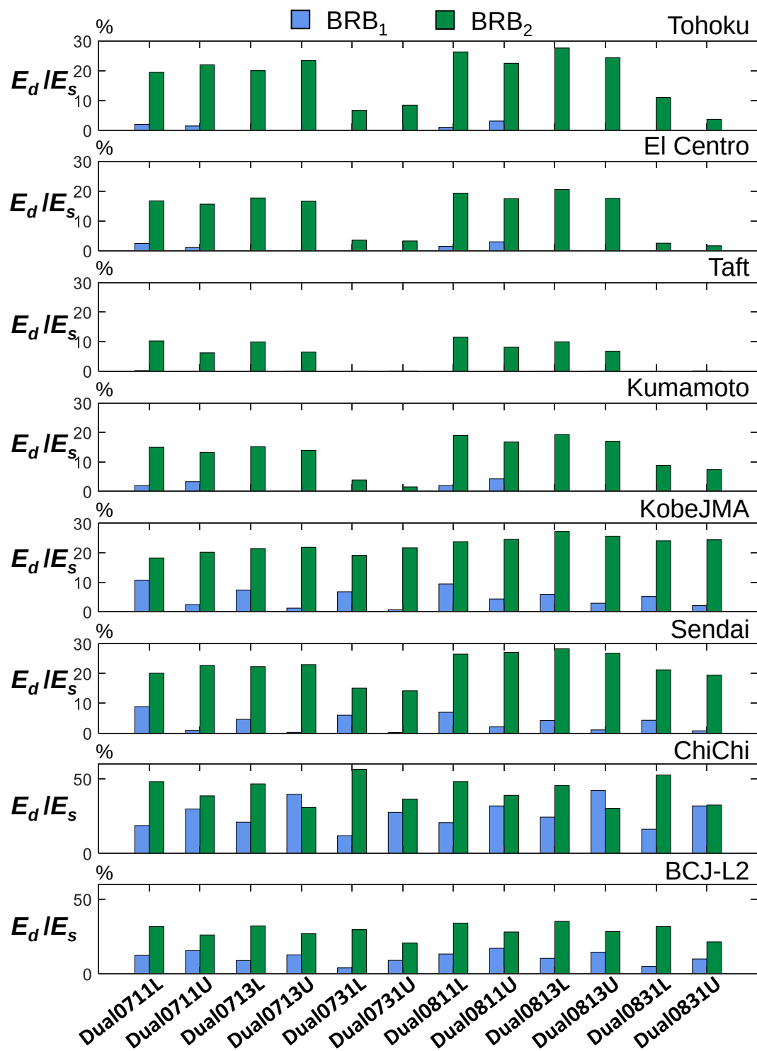
Figure 8.3.13 The E_d/E_s responses of the dual BRB-outrigger system calculated from the NLRHA
