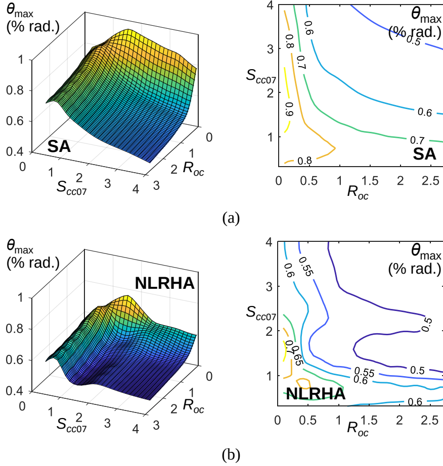
Figure 9.4.4 Distribution of \theta_{\max} with respect to S_{cc07} and R_{oc} calculated from (a) SA and (b) NLRHA
