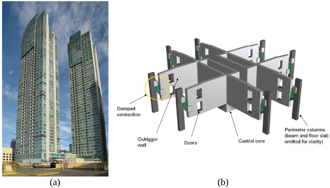
Figure 1.2.8 The (a) photo and (b) concrete outrigger walls connect to perimeter column with viscous dampers
