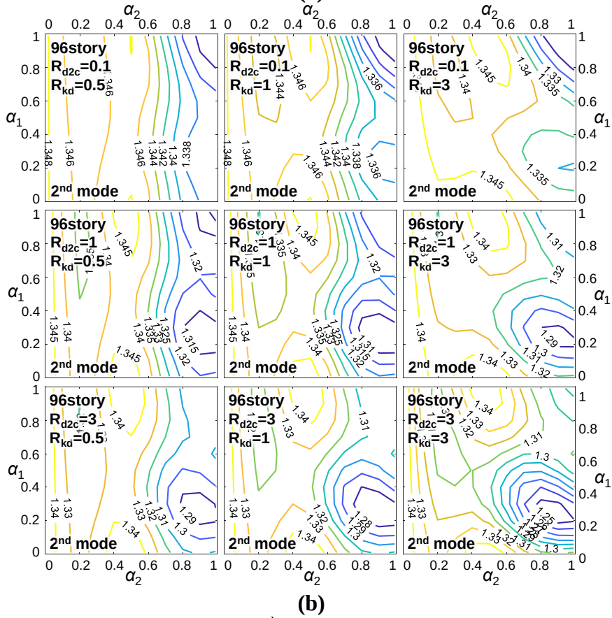
Figure 6.2.5 The (a) 1 st and (b) 2 nd mode vibration periods for 96-story model
