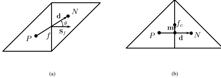
FIGURE D.1: Schematic diagrams for mesh non-orthogonality (a) and skewness (b).
