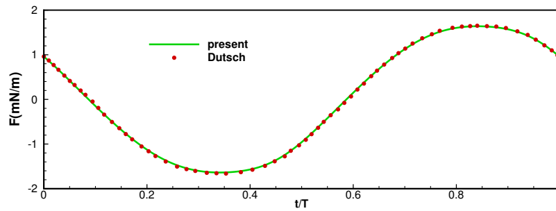
FIGURE 5.10: Comparison of inline force between present results and Dütsch's results [3].
