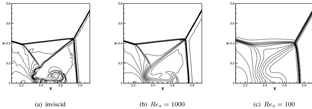
FIGURE 4.7: Comparison of (a) inviscid case (b) Re_s = 1000 and (c) Re_s = 100 at t = 0.2 with 296,418 triangular elements. 31 density isolines in the interval [1,17] .
