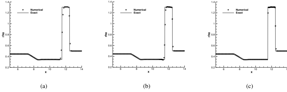
FIGURE 3.1: The density results for Lax problem with the present ALE scheme: (a) Eulerian ( u_g = 0 ); (b) ALE ( u_g = 0.5u ); (c) Lagrangian ( u_g = u ).
