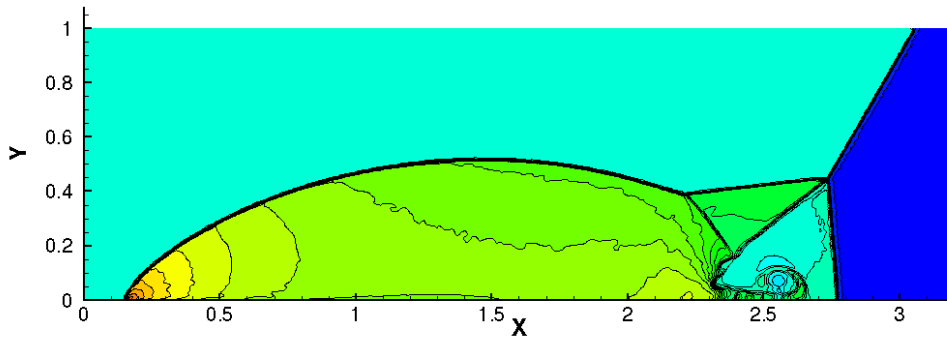
FIGURE 4.6: Numerical results of inviscid double Mach at t = 0.2 with 296,418 triangular elements. 31 density isolines in the interval [1,17] .
