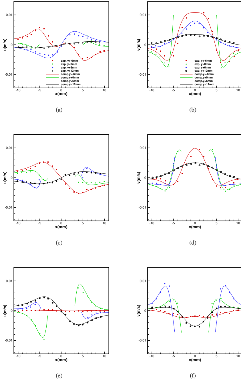
FIGURE 5.9: Comparisons of numerical and experimental results of x-component (left column) and y-component (right column) of fluid velocity in four different cross-sections at three phases: (1) 180^\circ : (a) (b); (2) 210^\circ : (c) (d); (3) 330^\circ : (e) (f).
