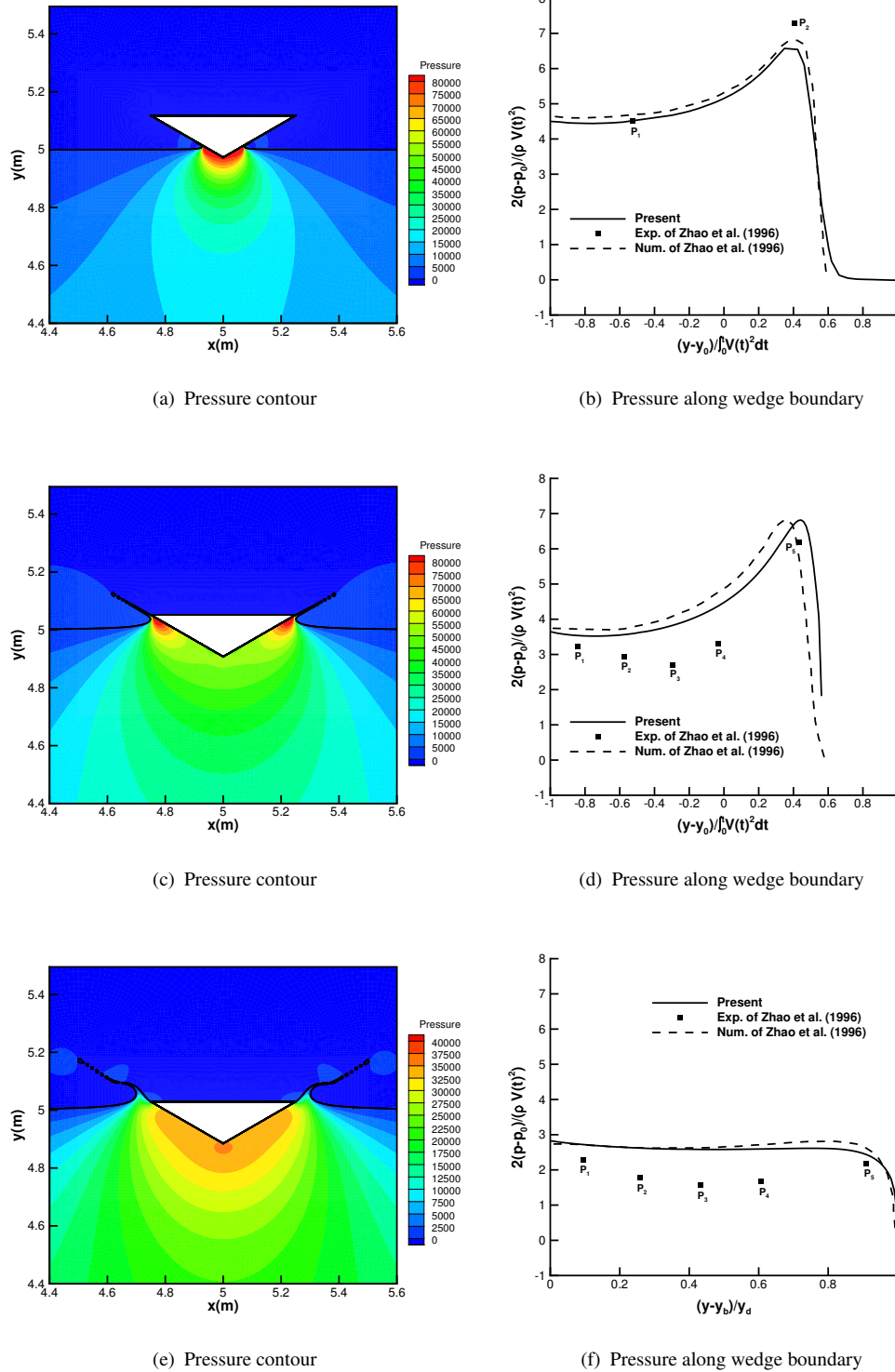
FIGURE 6.12: Pressure contour (left panels) and the comparisons of pressure along the wedge boundary (right panels) for different time instants. (a) (b) t=0.00435s ; (c) (d) t=0.0158s ; (e) (f) t=0.0202s . V(t) denotes the wedge velocity at time t . y is the vertical coordinate on the wedge surface. p_0 is the initial pressure at the nose of wedge. y_0 is the initial vertical coordinate of wedge nose, i.e. y_0 = 5m . y_b is the vertical coordinate of wedge nose at time t and y_d is the draft of the body.
