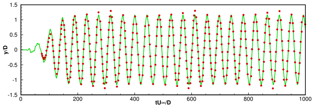
FIGURE 5.19: The y -component displacement of a square cross-section body \Lambda = 1 in a free-stream at Re = 250 , U_y^* = 40 , \zeta_y = 0.0037 and m^* = 20 . — is the present simulation and • denotes the results by a spectral element simulation [5].
