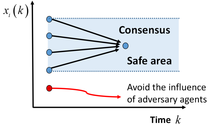
Figure 2.2: Resilient consensus problem
