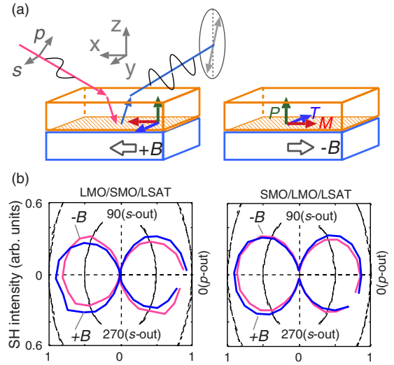
FIG. 2. (Color online) (a) Experimental geometry and coordination for the NMOKE measurement. s -polarized fundamental light incidents on the sample and polarization of the output SH is analyzed. The expected interface dipole ( \mathbf{P} ), magnetic ( \mathbf{M} ), and toroidal ( \mathbf{T} ) moments are shown by arrows. (b) Detected polarization rotation for LMO/SMO and SMO/LMO samples at 30 K under the in-plane magnetic field of 0.1 T (indicated with \pm B ). By reversing the external magnetic field, the direction of polarization rotation changes.
