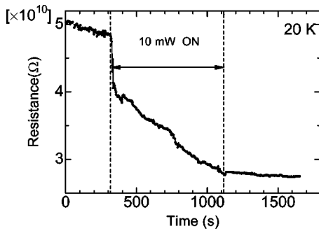
FIG. 4. Resistance as a function of time at 20 K. The sample was irradiated with a cw laser ( h\nu=2.33 eV) at the power density of 10 mW/ 0.01 cm ^2 .
