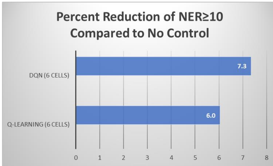
Figure 5. 19 Comparison among Q-learning (0.9 km), DQN (0.9 km)
