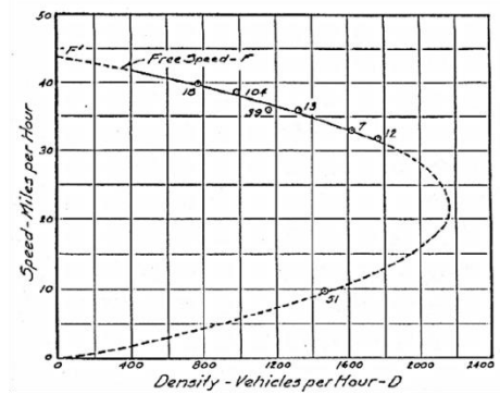
Figure 2. 1 Speed–density relation V (Greenshields 1934) and The first Fundamental Diagram as q-v diagram (Ku'hne,R.D.,2011)
