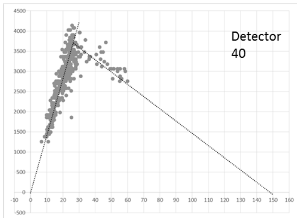
Figure 2. Individual and aggregated fundamental diagram (detector 48-39), June3
