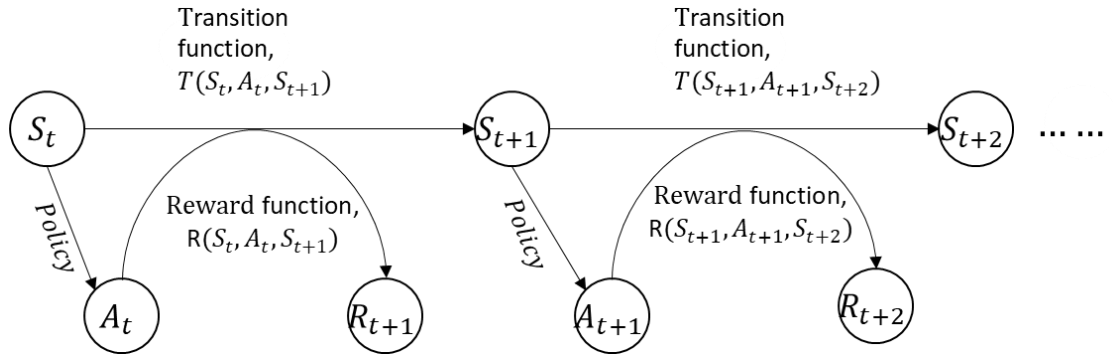
Figure 5. 6 Illustration of MDPs (Levet et al, 2018)
