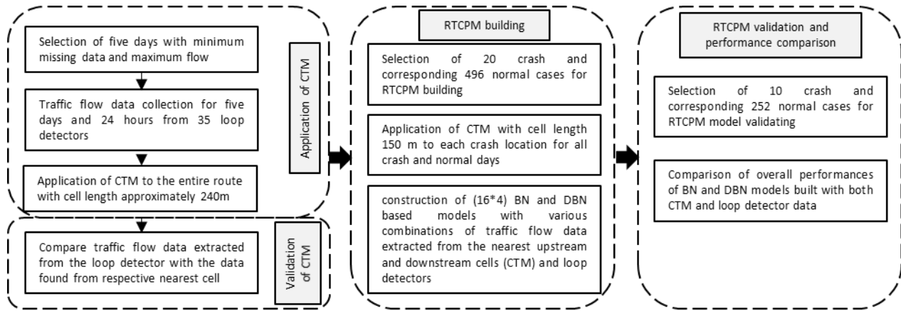
Figure 3. 2 Workflow diagram
