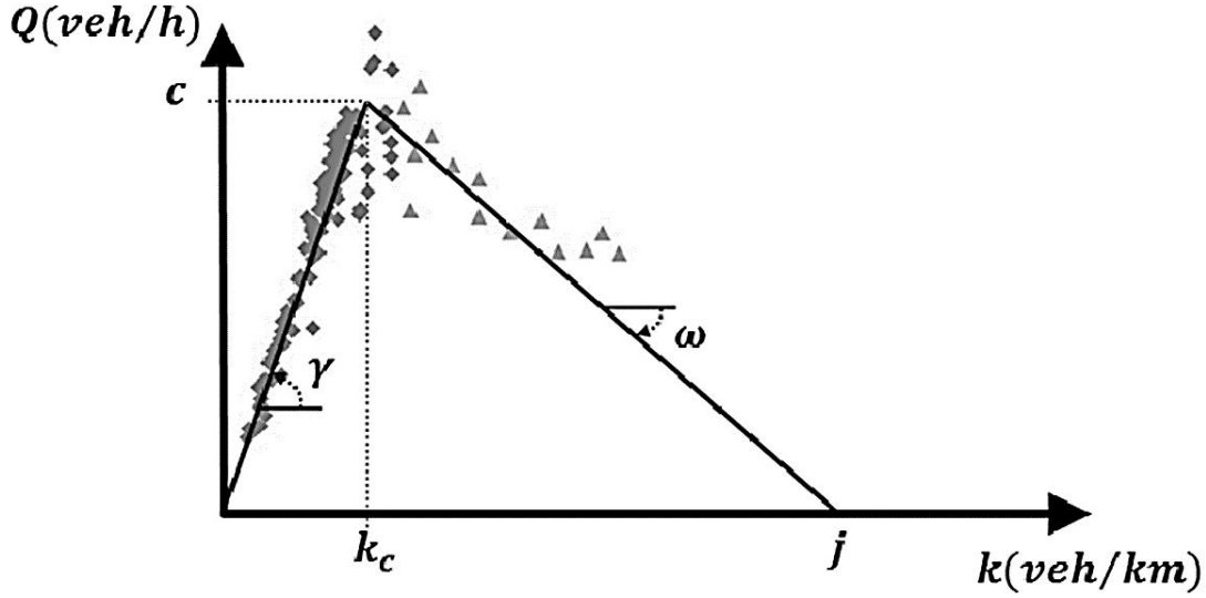
Figure 2. 2 Speed–density relation V (Greenshields 1934) and The first Fundamental Diagram as q-v diagram (Ku'hne,R.D.,2011)
