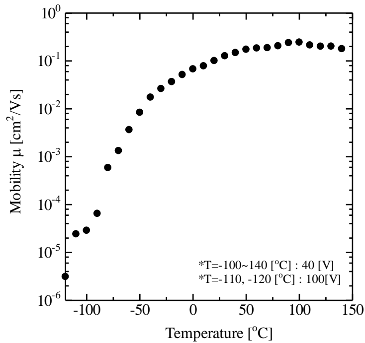
図 4.13: Temperature dependence of hole mobility of Ph-BTBT-4O-3.
