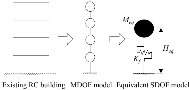
Fig. 2 – Simplification of the RC building to SDOF model
