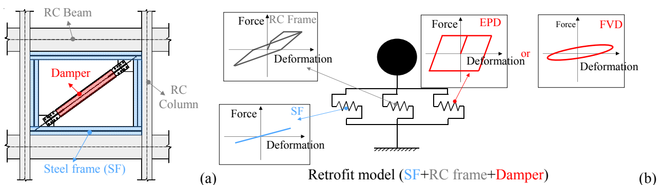
Fig. 1 –Retrofitted concept (a) Configuration and (b) Simplified SDOF model
