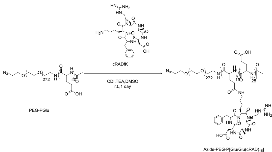
Figure 2.2.4. Synthesis of Azide-PEG-P[Glu/Glu(cRAD) 15 ].
