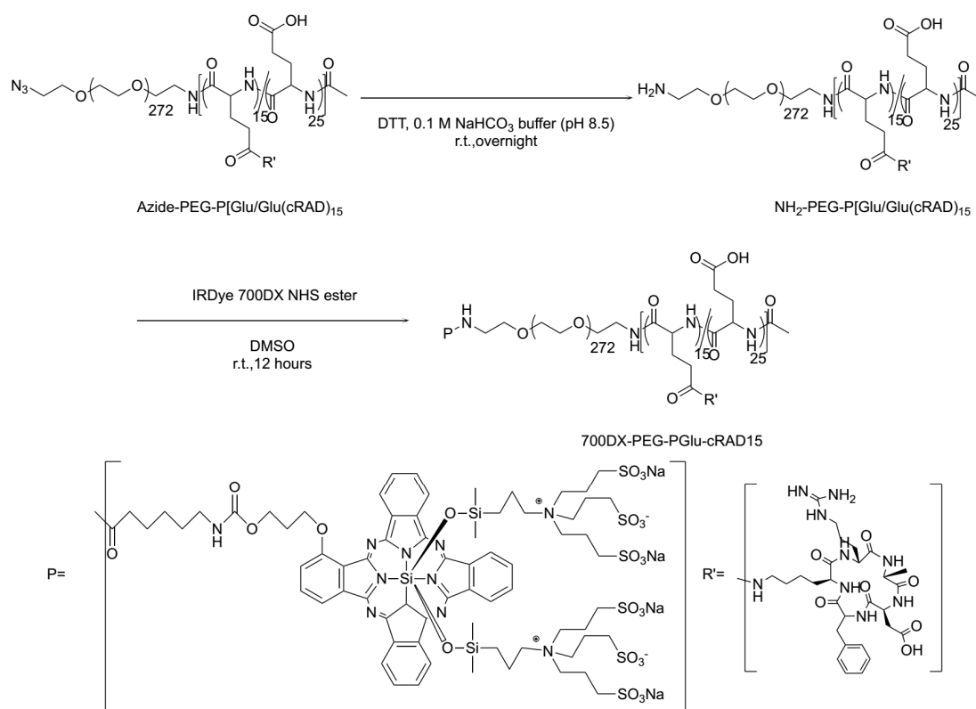
Figure 2.2.6. Synthesis of 700DX-PEG-PGlu-cRAD15.
