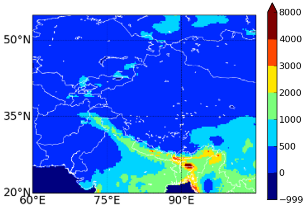
Figure 5.4: Annual precipitation in APHRODITE ( mm \ year^{-1} )
