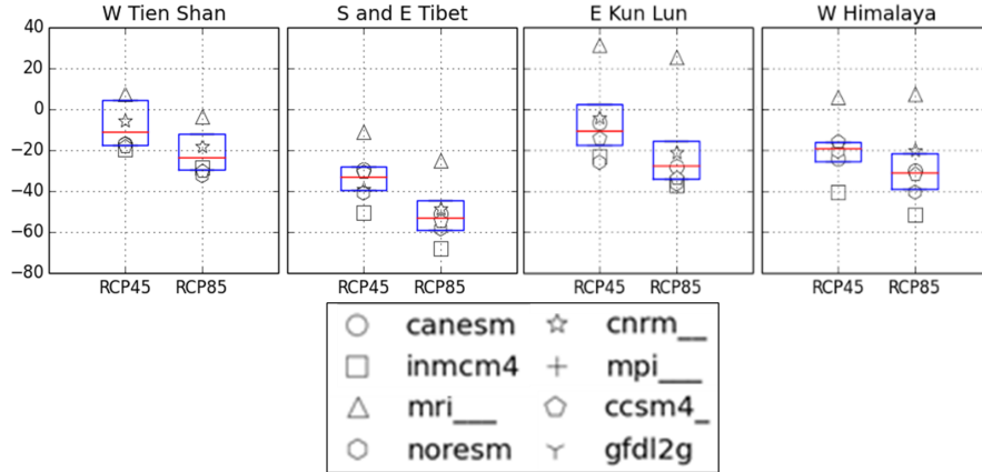
Figure A.3: A preliminary experiment. We used the HYOGA2 model with several ensembles of GCM simulations to select typical GCMs. Examples of projected changes in snowfall (%) within West Tien Shan, South and East Tibet, East Kun Lun, and the West Himalaya are shown. We used eight GCMs and two RCPs.
