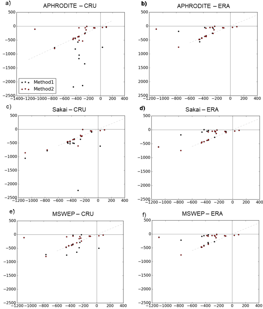
Figure A.5: Comparisons of modeled (y-axis) and observed (x-axis) average annual glacier mass changes ( \text{mm w.e. year}^{-1} ) from 1980 to 2004, using (a) APHRODITE precipitation and CRU temperature data; (b) APHRODITE precipitation and ERA-Interim temperature data; (c) Sakai precipitation and CRU temperature data; (d) Sakai precipitation and ERA-Interim temperature data; (e) MSWEP precipitation and CRU temperature data; and (f) MSWEP precipitation and ERA-Interim temperature data. The DDFs (the C_p , the DDFs, and the dT ) were calibrated using Method 1 (Method 2).
