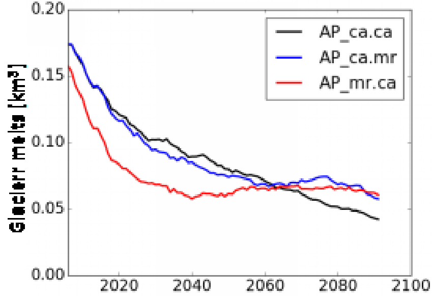
Figure A.7: Differences of “default experiments” and “shuffle experiments” of GCM air temperature and precipitation. Total glacier melt ( km^3 ) for selected 304 glaciers. CCCma-CanESM2 air temperature and precipitation were used as the default experiment. CRU and APHRODITE were used as observed past air temperature and precipitation. Red: shuffle GCM air temperature; Blue: shuffle GCM precipitation; ca: CCCma-CanESM2; cc: NCAR-CCSM4; mr: MRI-CGCM3.
