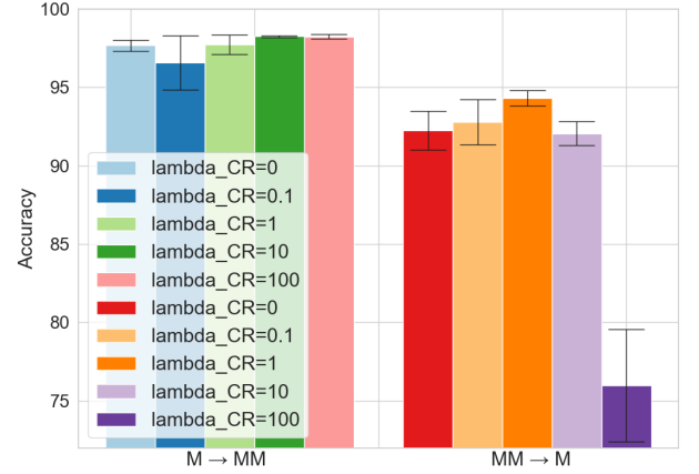
Fig. 6: Different choices of \lambda_{\text{Real}} . \lambda_{\text{CR}} stands for the value of \lambda_{\text{Real}} . The bars of \lambda_{\text{Real}} = 0 denote the CycleGAN baseline and the others are CR-CycleGANs.
