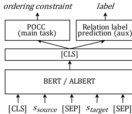
FIGURE 5.2: My architecture for fine-tuned POCC models.
