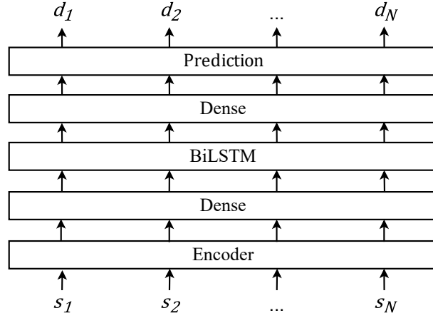
FIGURE 4.1: BiLSTM-softmax (SEQTG).
