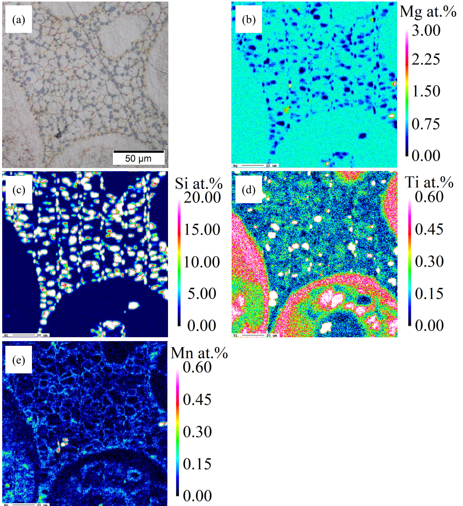
Fig. 2-20. Optical micrograph of the eutectic region etched by Weck's reagent (a) and results of EPMA analysis, (b) Mg, (c) Si, (d) Ti and (e) Mn.
