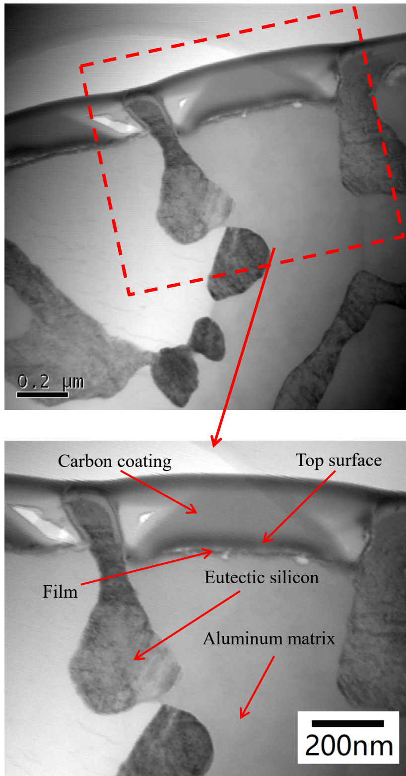
Fig. 2-13. Cross-section of the eutectic solidified region of as-cast specimen observed by STEM.
