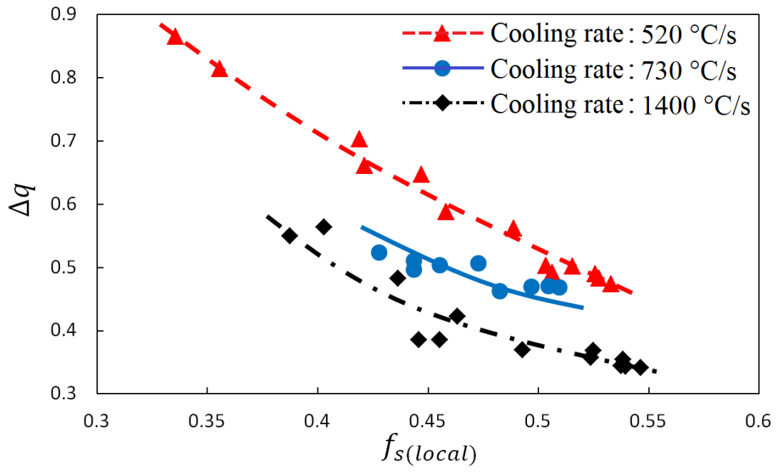
Fig. 4-10. Quantitative analysis result of the amount of grain growth during water quenching, \Delta q , under the different local solid fractions.
