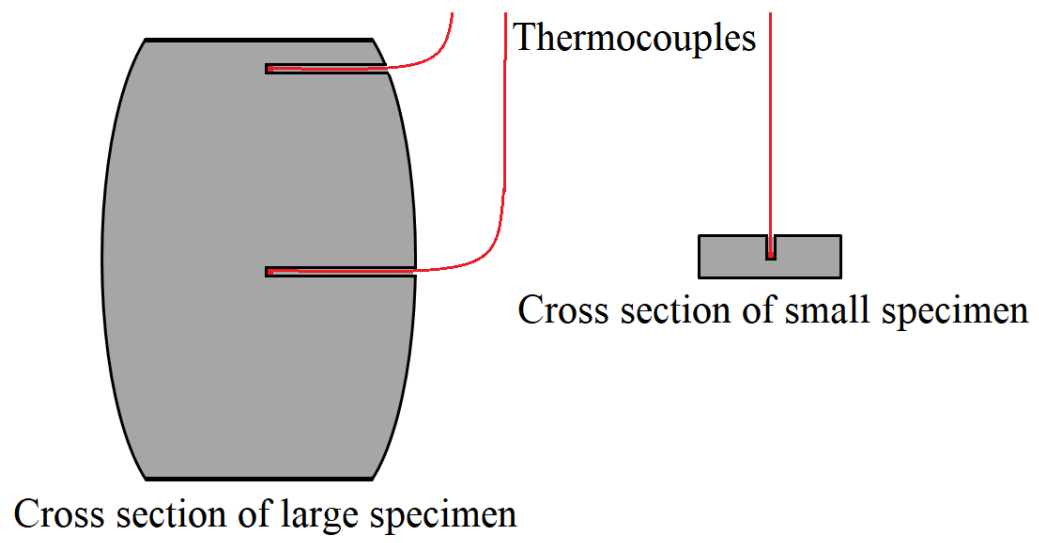
Fig. 4-2. Schematic of thermocouples insert in the specimens in in this chapter.
