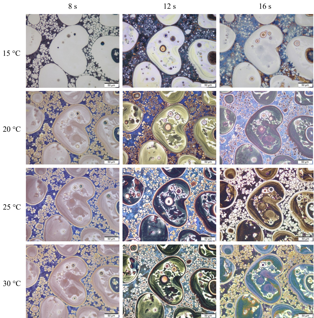
Fig. 3-11. The temperature-time chart of color contrast of the as-cast specimen etched with different etching conditions
