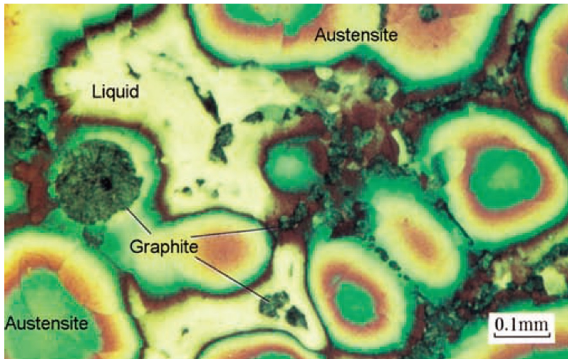
Fig. 1-2. An example of color etched austenite showing different color which is caused by Si micro-segregation [9].
