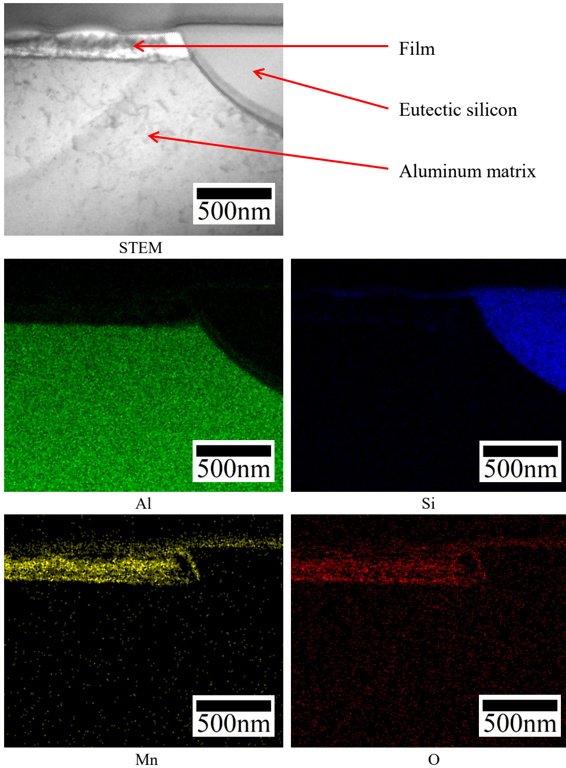
Fig. 2-16. Composition analysis of solution-treated specimen by STEM equipped with EDS.
