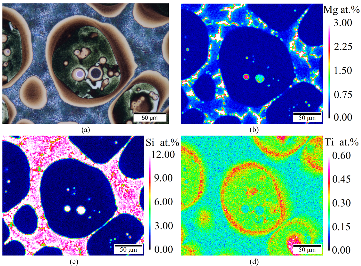
Fig. 4-6. Optical micrograph of the specimen etched by Weck's reagent (a) and results of EPMA analysis, (b) Mg, (c) Si, (d) Ti.
