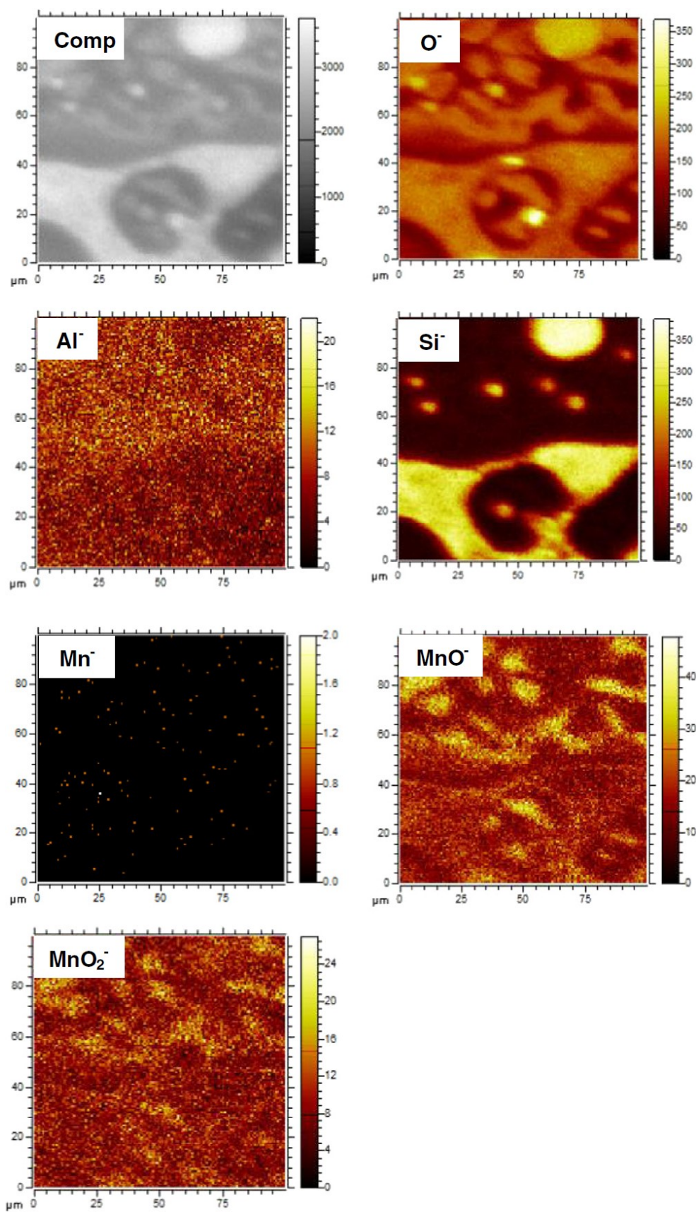
Fig. 1-15. Mapping of negative ions from the film analyzed by TOF-SIMS [17].
