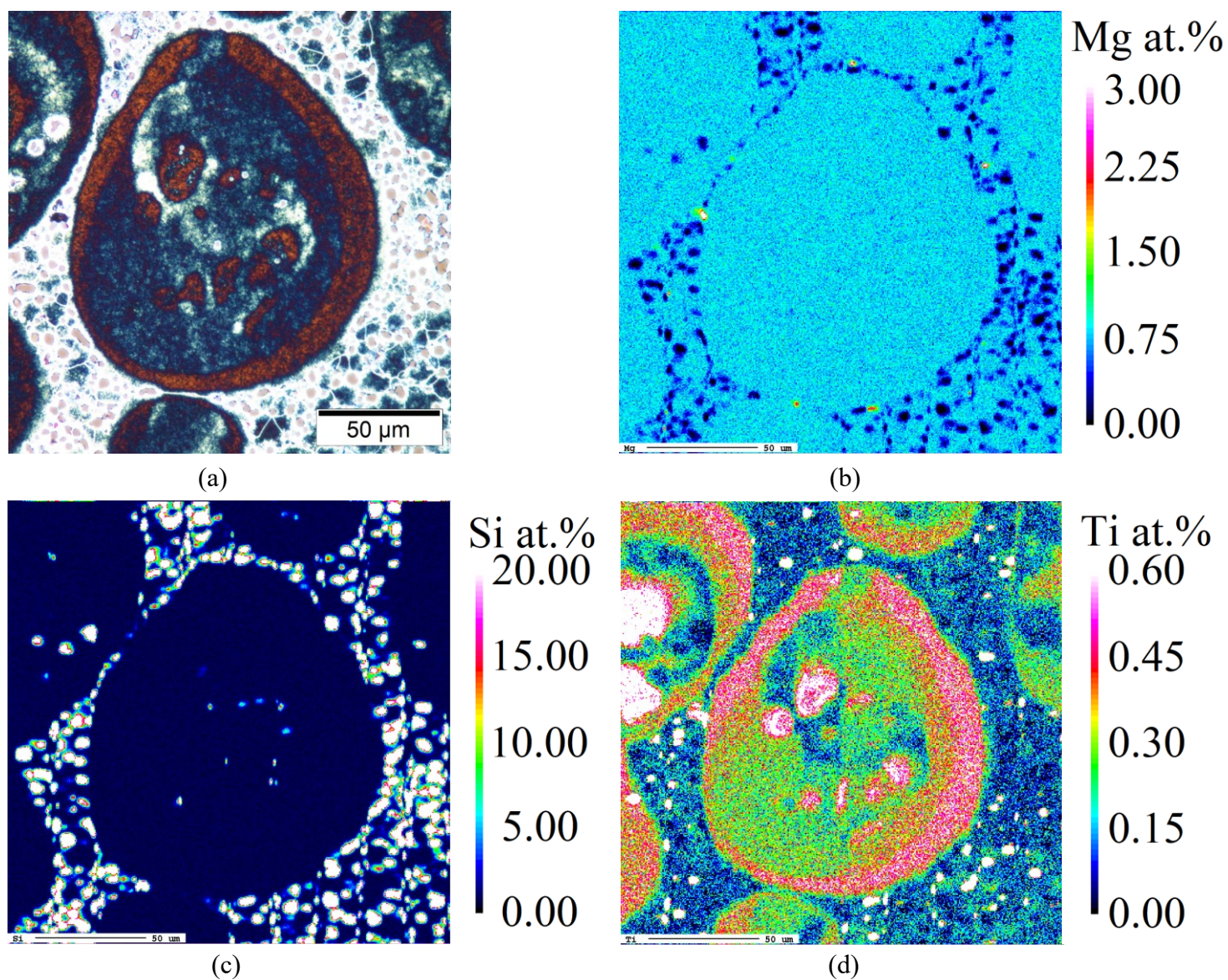
Fig. 2-17. Optical micrograph of the large primary \alpha -Al grain etched by Weck's reagent (a) and results of EPMA analysis, (b) Mg, (c) Si, (d) Ti.
