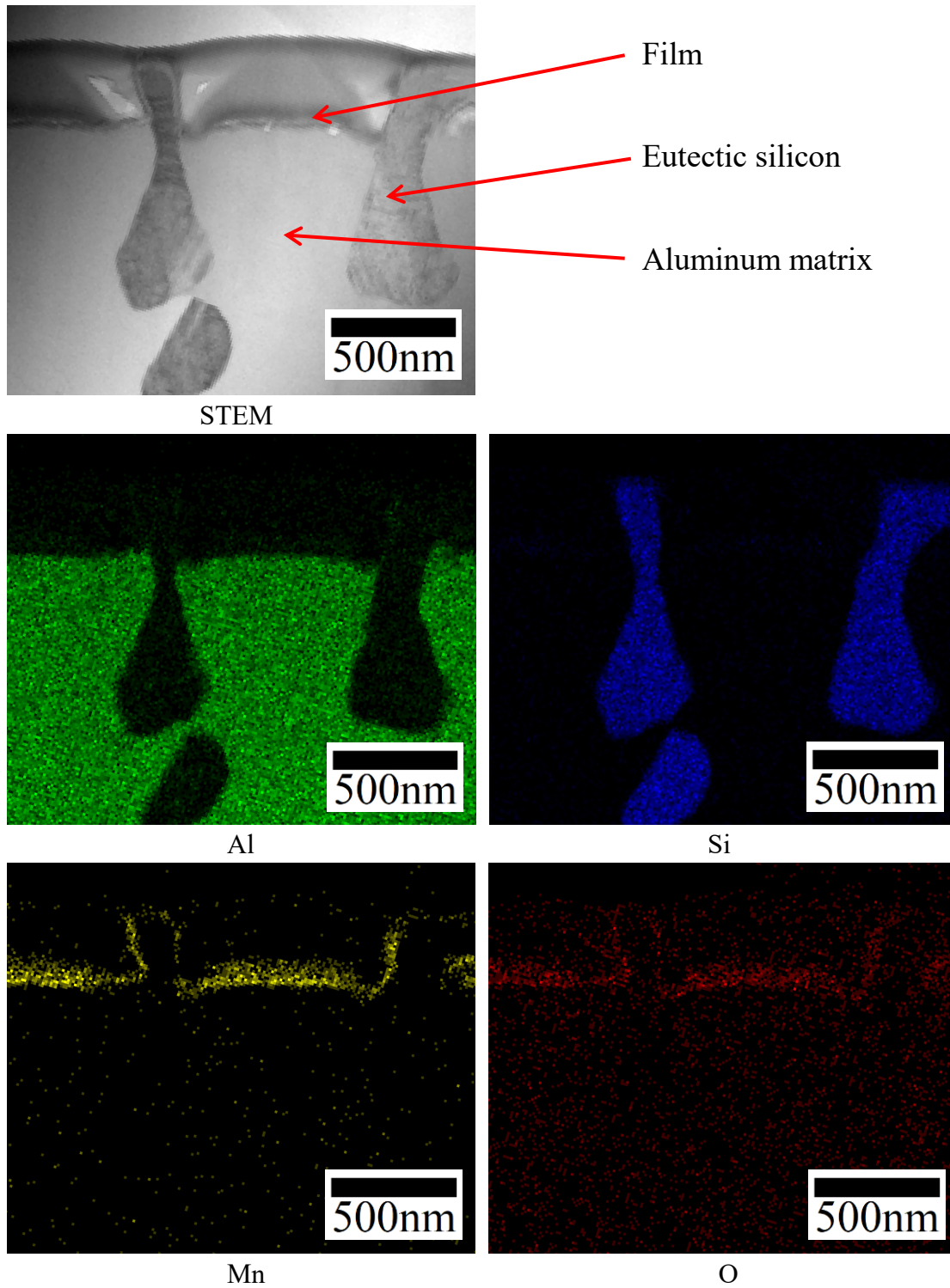
Fig. 2-14. Composition analysis of as-cast specimen by STEM equipped with EDS.
