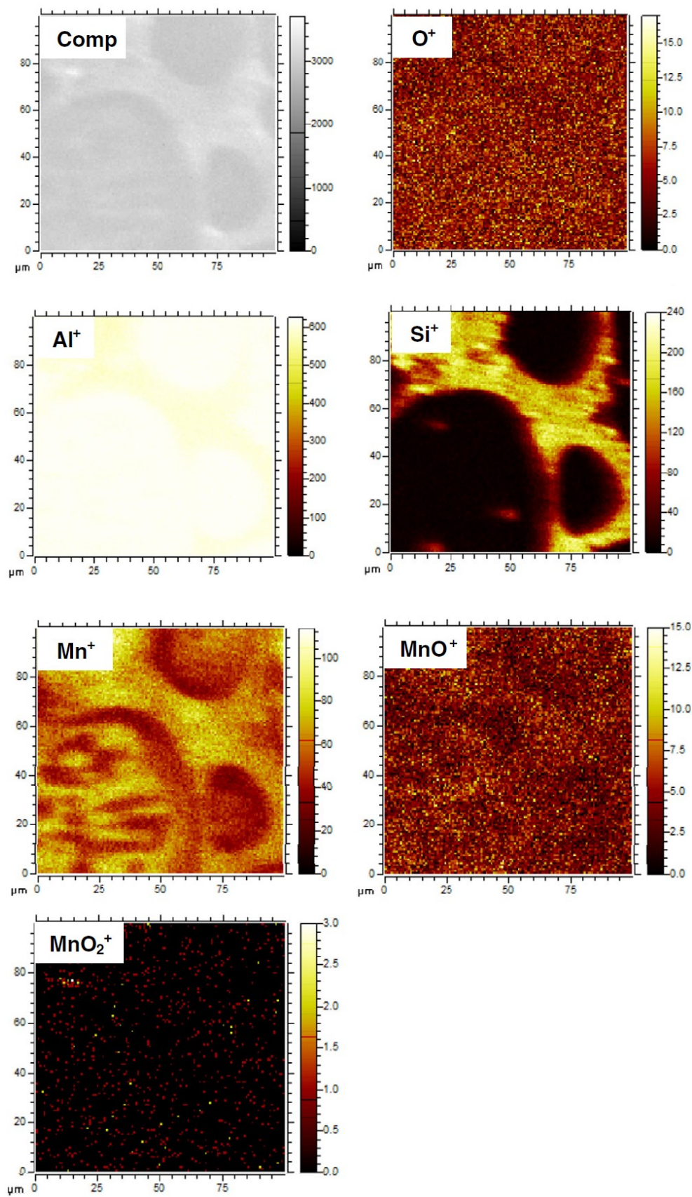
Fig. 1-16. Mapping of positive ions from the film analyzed by TOF-SIMS [17].
