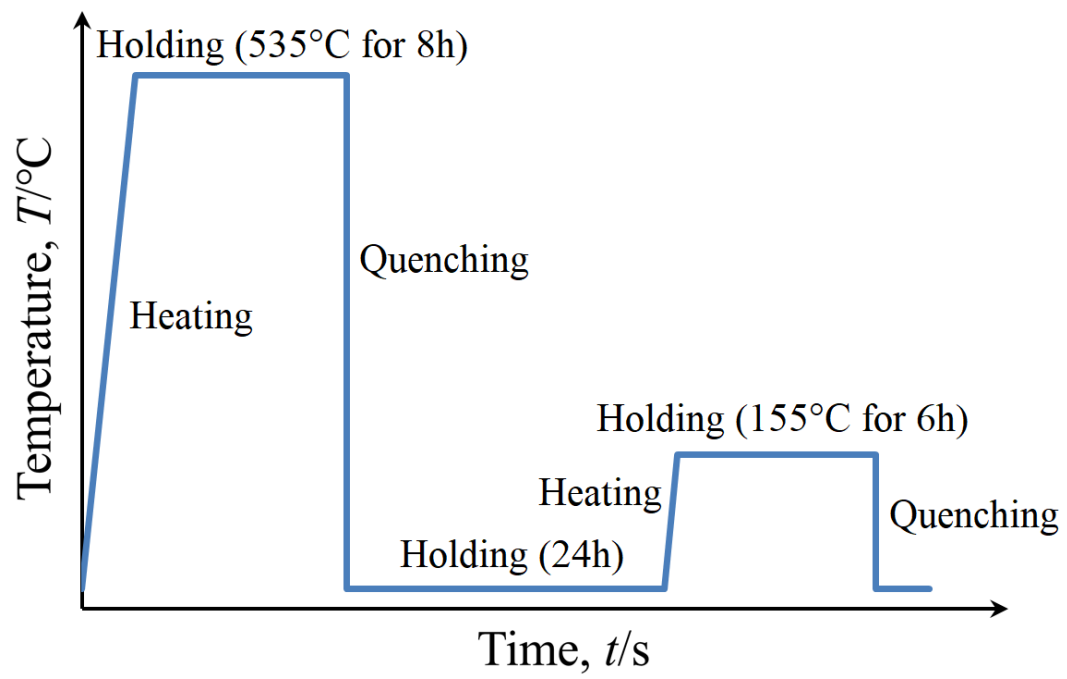
Fig. 2-4. Schematic temperature-time curve for solution treatment process in this chapter.
