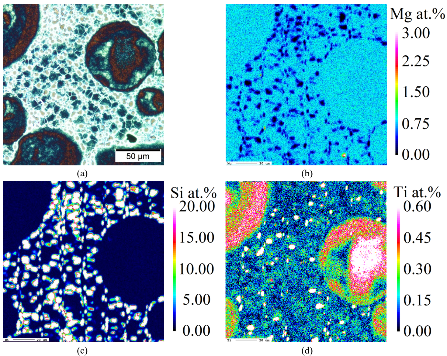
Fig. 2-18. Optical micrograph of the eutectic region etched by Weck's reagent (a) and results of EPMA analysis, (b) Mg, (c) Si, (d) Ti.
