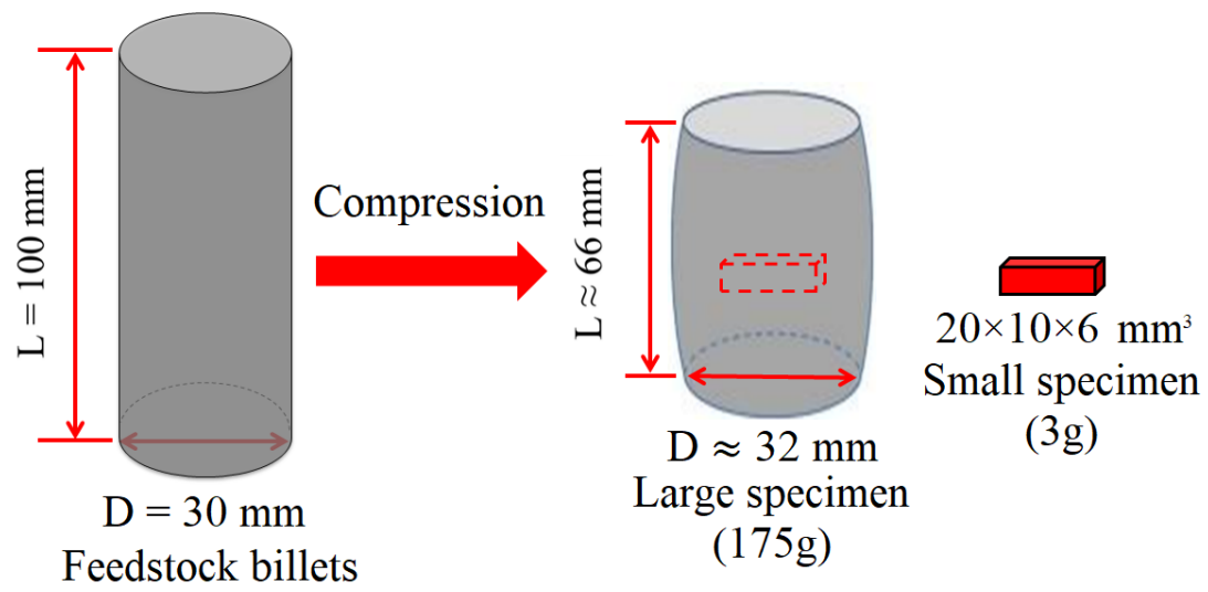
Fig. 4-1. Definition of large specimen and small specimen used in this chapter.
