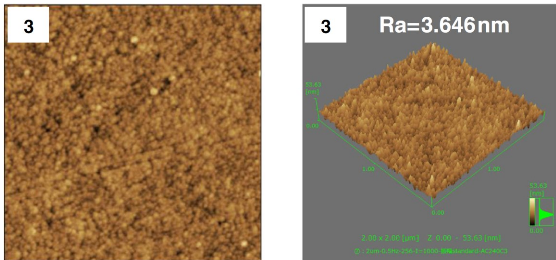
Fig. 1-12. Both 2D and 3D surface profile made by AFM, the number indicates the analyzed location in Fig. 1-11 [17].
