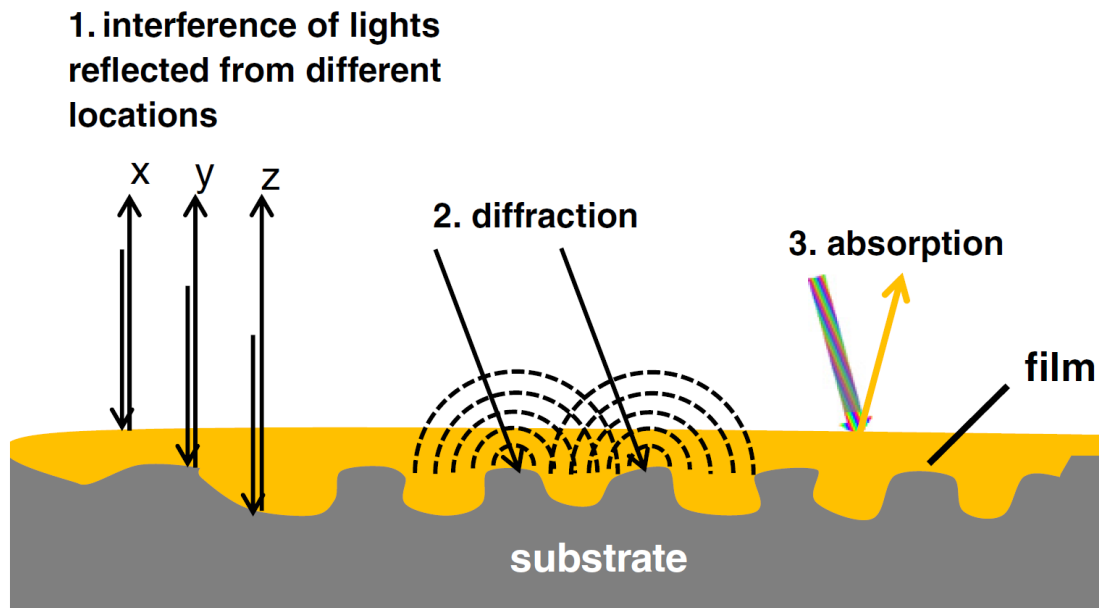
Fig. 1-17. Schematic illustration showing the cross section of the specimen after etching as well as three proposed coloring mechanisms [17].
