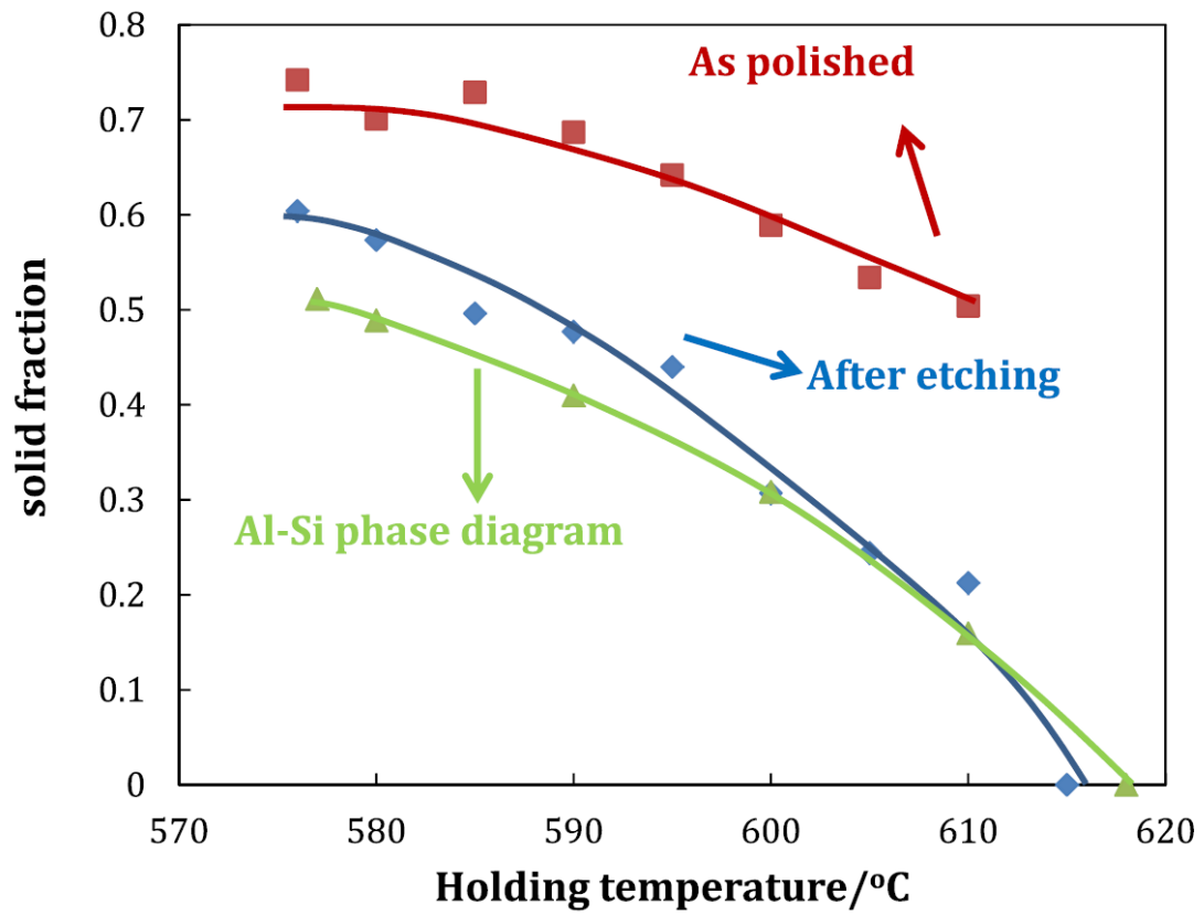
Fig. 1-8. Solid fractions of A356 aluminum alloy measured from as polished and as etched specimens, as well as the calculation using Al-Si binary phase diagram [16].
