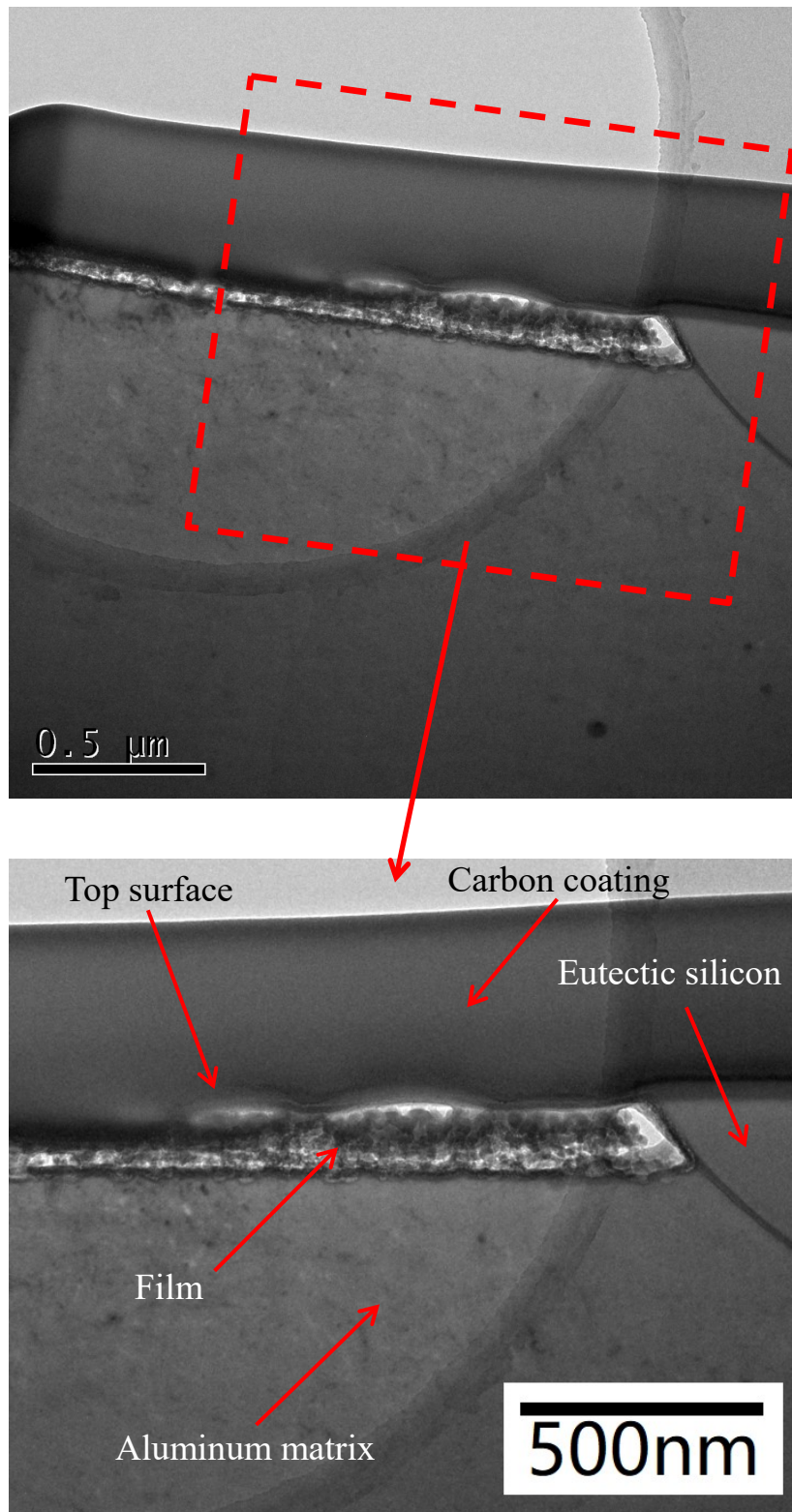
Fig. 2-15. Cross-section of the eutectic solidified region of solution-treated specimen observed by STEM.
