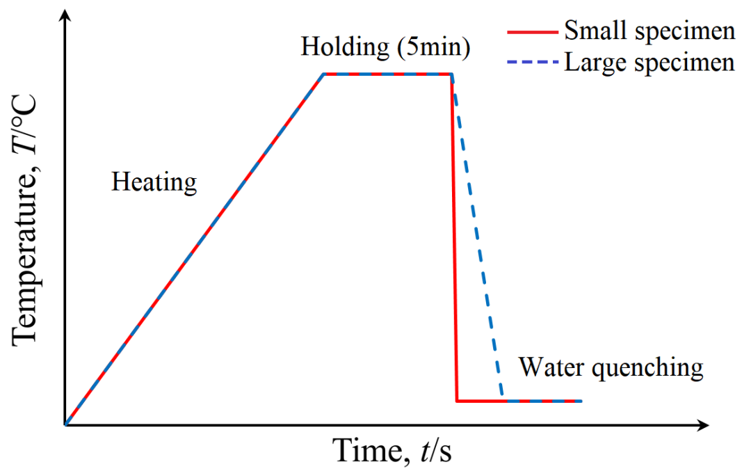
Fig. 4-3. Schematic temperature-time curve for heating, holding and cooling process in this chapter.
