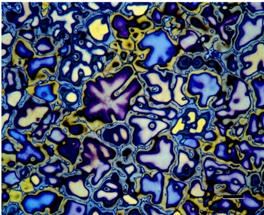
Fig. 1-5. An example of color etching provided in [1]. The micrograph is observed with crossed polarized light and sensitive tint so the color contrast is strengthened. Magnification bar is 50 \mu\text{m} long.
