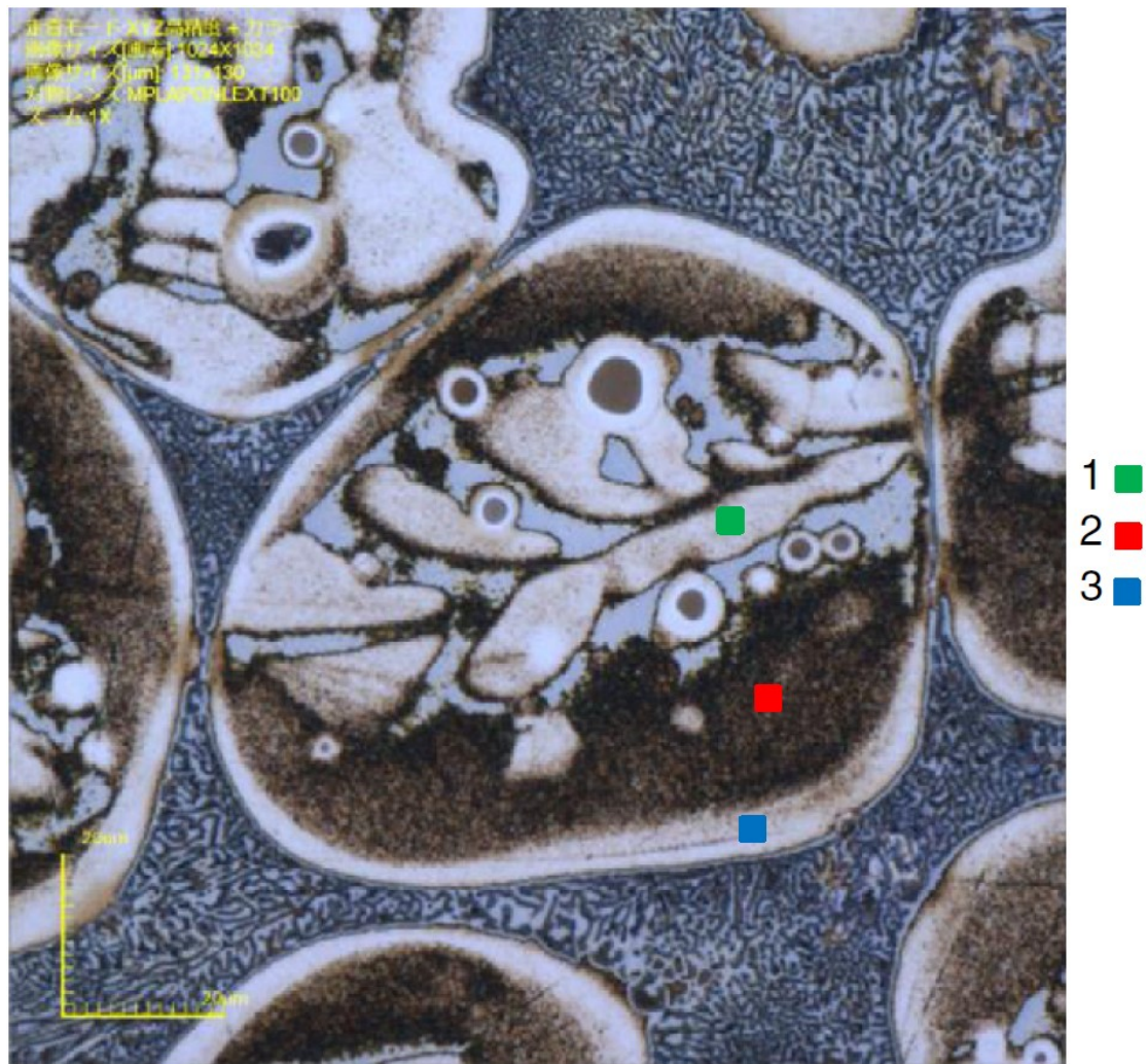
Fig. 1-11. Optical micrograph of the spheroidal grain which was characterized by AFM. The three analysis locations are indicated by three points [17].
