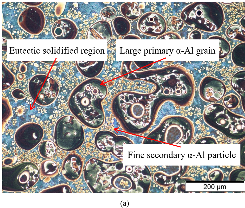
Fig. 2-6. Microstructure of the as-cast specimen etched by Weck's reagent for different magnifications and locations.
