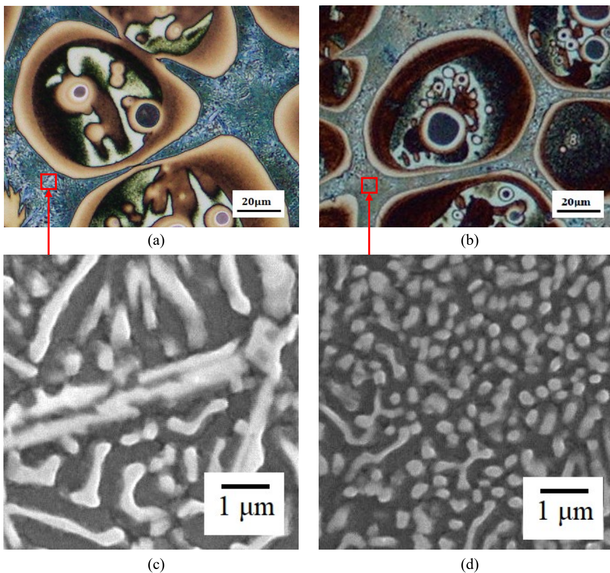
Fig. 4-5. (a) and (b): Optical micrographs of the etched microstructure by Weck's reagent of the quenched large specimen and small specimen from 588°C. (c) and (d): SEM image of the quenched liquid region showing the eutectic solidified structure.
