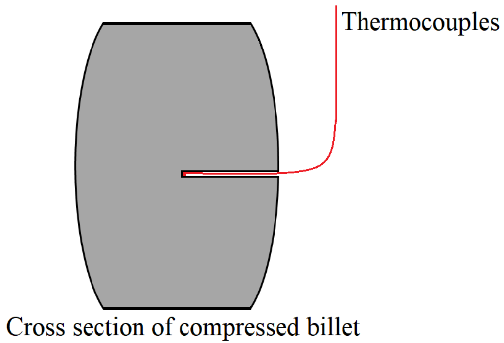
Fig. 2-2. Schematic of thermocouple insert in the compressed billet.
