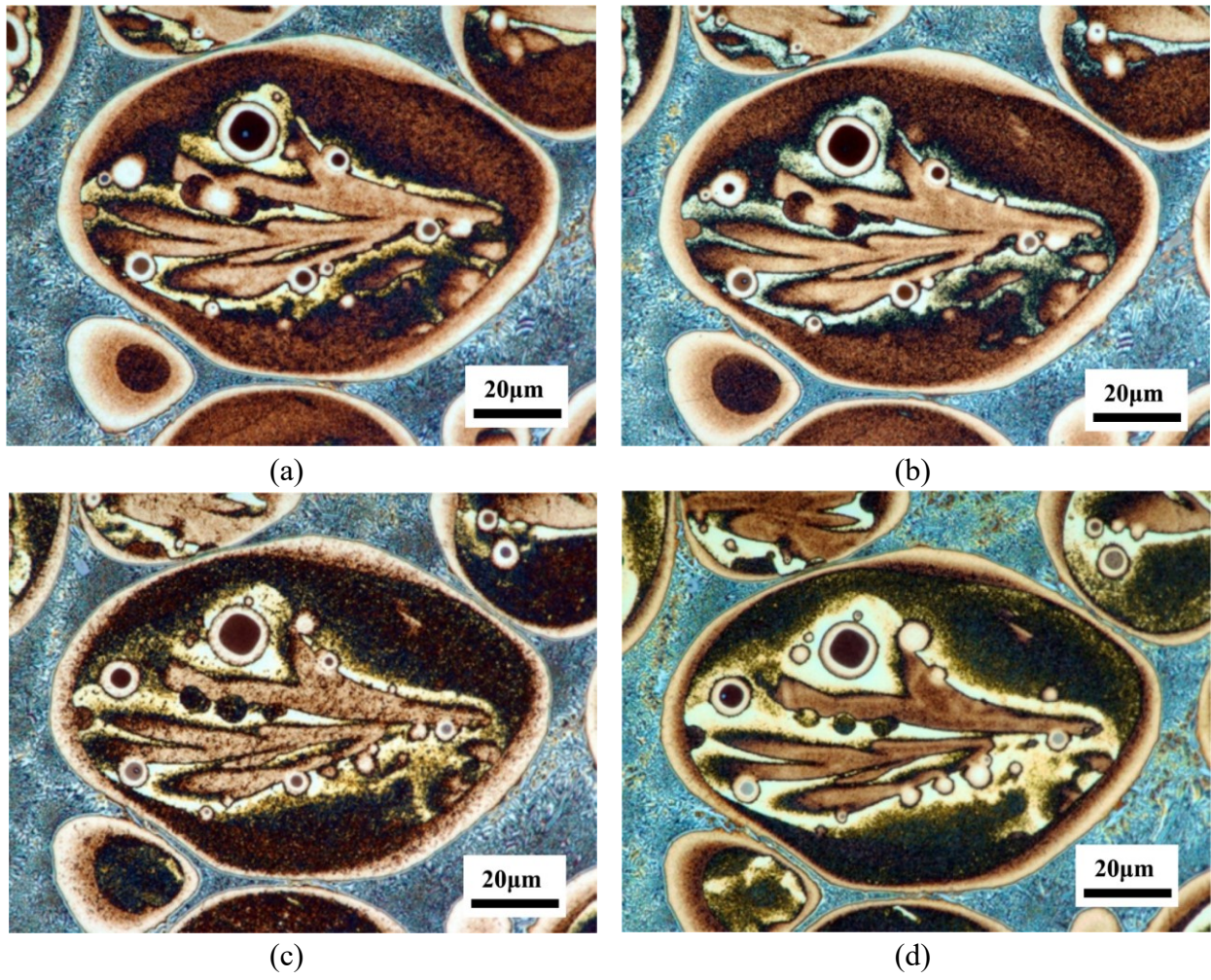
Fig. 3-1. Repeating etching using Weck's reagent for four times with the same etching time of 12 s [1].
