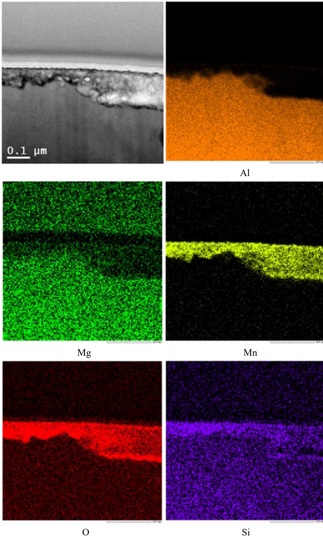
Fig. 1-14. Composition analysis of the film by STEM equipped with EDS [17].
