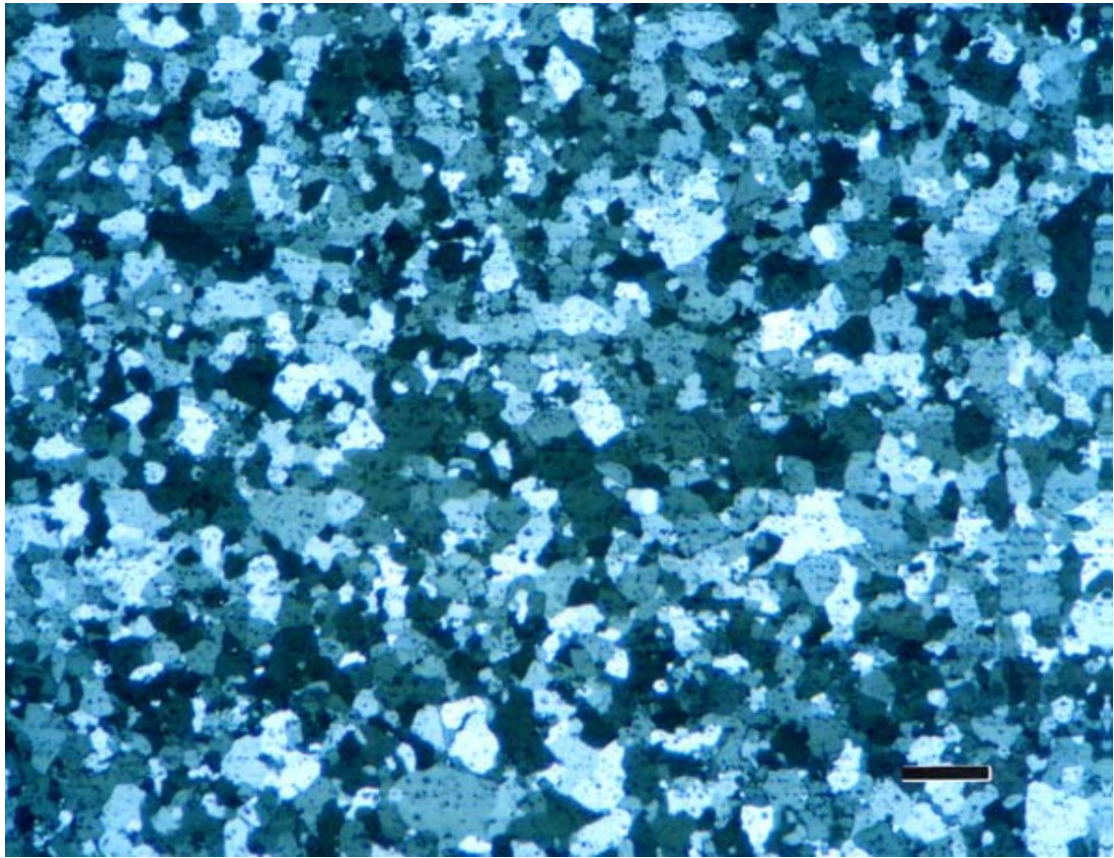
Fig. 1-4. An example showing the grain structure of wrought aluminum alloy after anodizing [1]. The microstructure was observed under polarized light and the magnification bar is 100 \mu\text{m} long
