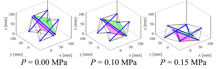
Fig. 8. Tensegrity model of Pattern 1 as the pressure is varied.
