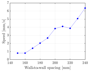
Fig. 17. Relationship between wall-to-wall spacing and speed.
