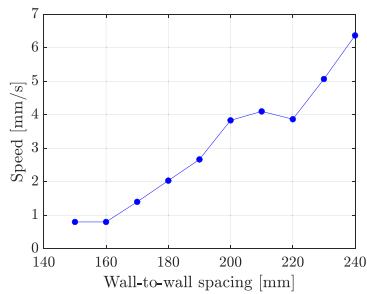
Fig. 17. Relationship between wall-to-wall spacing and speed.
