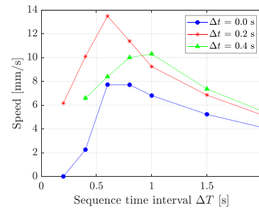
Fig. 19. Relationship between the sequence time interval \Delta T and speed when the wall spacing is 210 mm.
