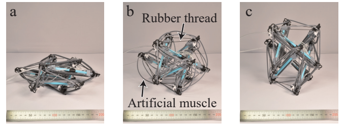
Fig. 13. (a) Tensegrity when artificial muscles are applied in Pattern 1. (b) Tensegrity in the initial state. (c) Tensegrity when artificial muscles are applied in Pattern 2.
