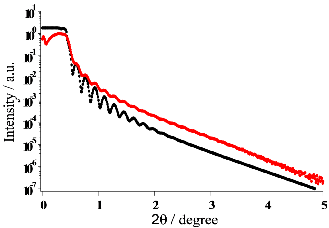
Figure 2-2. X-ray reflectivity curve of PS brushes on glass substrate. The experimental data was fitted by setting the brush to 48.2 nm. The density ( \rho ) of the PS layer was assumed to be 1.05 \text{ g cm}^{-3} (equal to \rho of the bulk PS).
