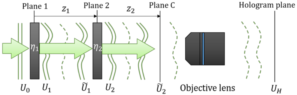
Fig 5.2: Imaging model for digital holography.
