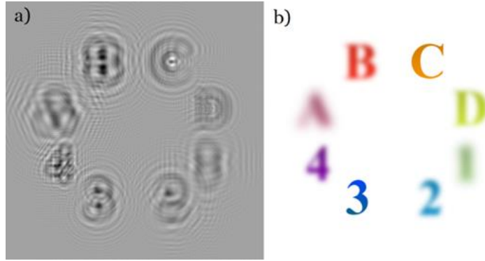
Fig. 5.6: Amplitude of object wave and (b) color BF image. Object A1 appears the most blurred in (b) as it is farthest from plane C.
