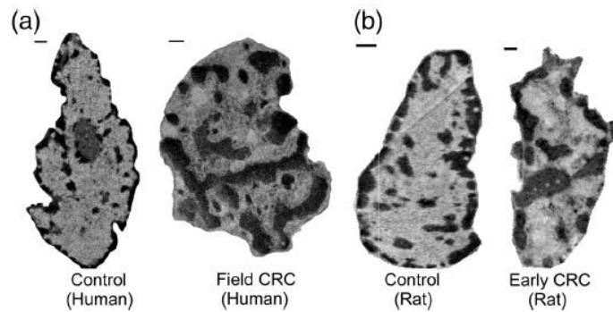
Fig 2.2: a) Normal nuclei from control patients and a pre-cancerous adenoma representing field CRC. Scale bars: 500 nm. b) Normal colonic cell nuclei from control rats and early CRC. Scale bars: 250 nm. (Copyright Cherkezzyan et al. 2014)
