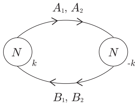
Figure 2.2: The quiver diagram of the ABJM theory is shown.
