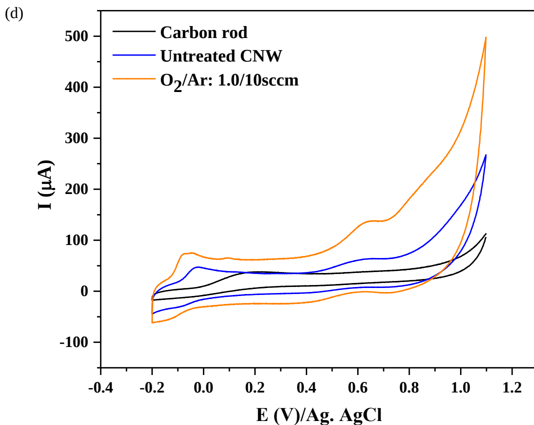
Figure. 5.8. CV profiles of (a) carbon rod, (b) untreated CNW, and (c) CNW treated with \text{O}_2/\text{Ar} : 1.0/10sccm in phosphate buffer solution, 1mM AA, 0.1mM UA, and binary mixture of 1mM AA + 0.1mM UA, and (d) their comparison for binary mixture of 1mM AA + 0.1mM UA
