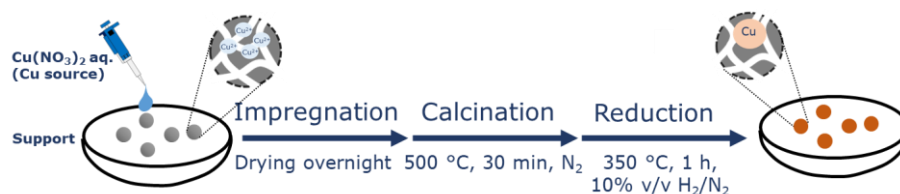
Figure 2.3: Schematic diagram of the preparation of supported monometallic Cu catalysts using the impregnation method.
