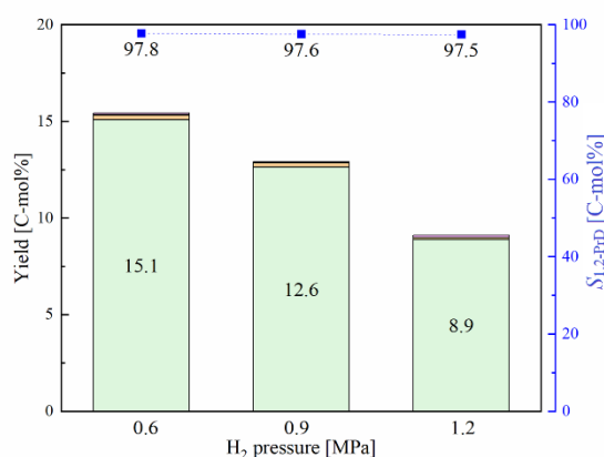
Figure 3.3: Effect of H 2 pressure on product yields. (Reactant: 20 g of 15 wt% aqueous glycerol solution, catalyst loading: 0.2 gCu/g glycerol , reaction temperature: 180 °C, reaction time: 24 h, initial H 2 pressure: 0.6–1.2 MPa)
