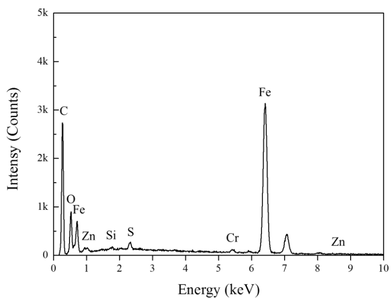
Fig. 4.42 Characteristic EDS-spectra of injector no.4 at the inlet of hole.
