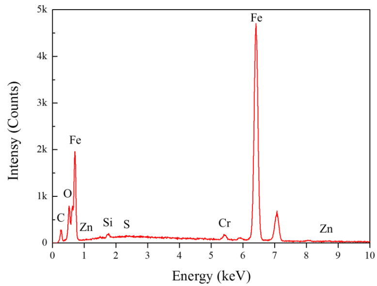
Fig. 4.34 Characteristic EDS-spectra of injector no.1 at the middle of hole.
