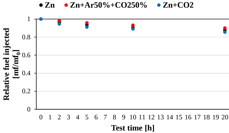
Fig. 4.31 Relative fuel injected amount at 1,000 \mu\text{s} .
