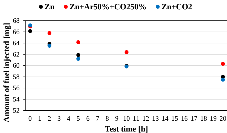
Fig. 4.30 Amount of fuel injected at 1,000 \mu s.
