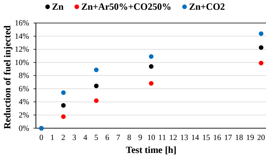
Fig. 4.32 Fuel injected difference at 1,000 \mu\text{s} .
