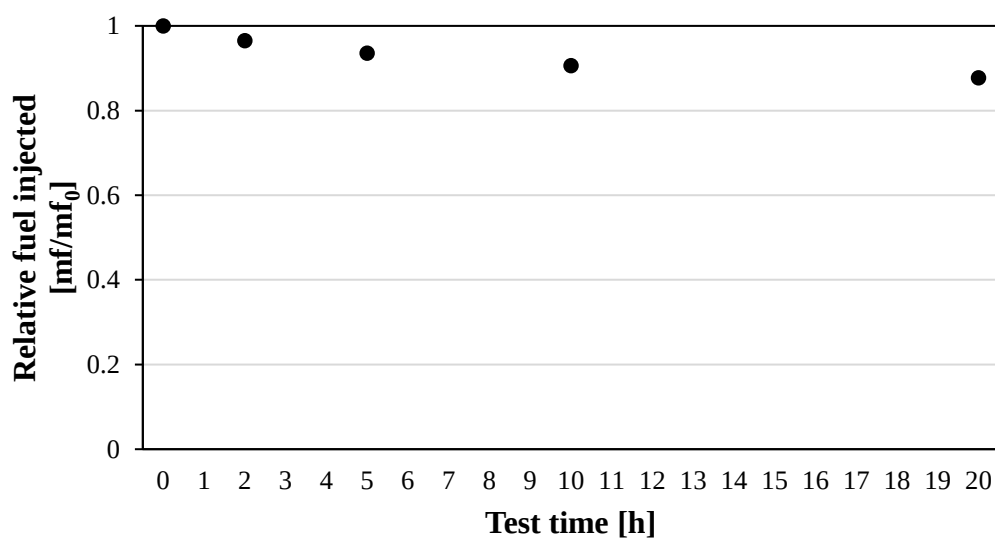
Fig. 4.7 Relative fuel injected amount at 1,000 \mu s.
