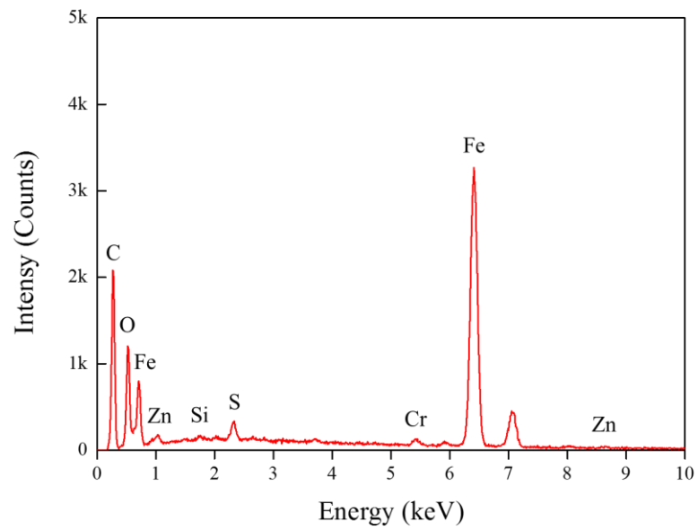
Fig. 4.40 Characteristic EDS-spectra of injector no.3 at the middle of hole.
