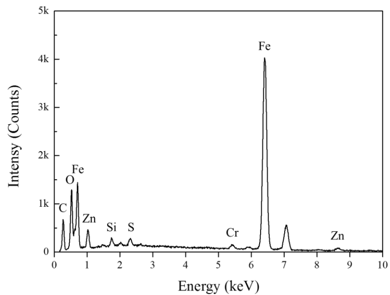
Fig. 4.18 Characteristic EDS-spectra of injector no.3 at the inlet of hole
