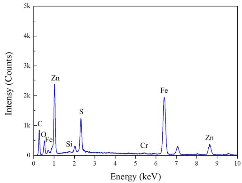
Fig. 4.23 Characteristic EDS-spectra of injector no.4 at the outlet of hole.
