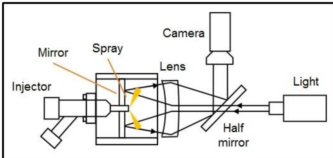
Fig. 2.22 Schematic of spray observation device.
