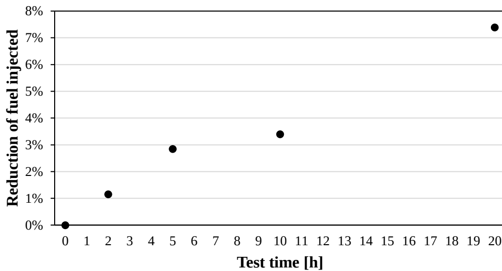
Fig. 4.5 Fuel injected difference at 480 \mu s.
