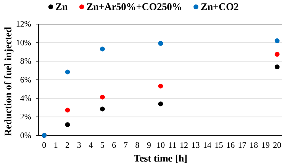
Fig. 4.29 Fuel injected difference at 480 \mu s.
