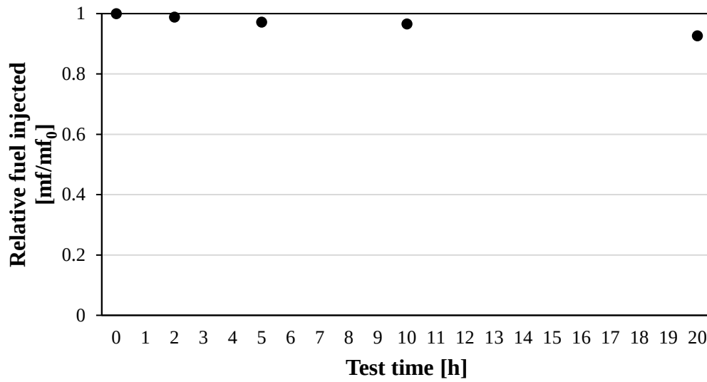
Fig. 4.4 Relative fuel injected amount at 480 \mu s.
