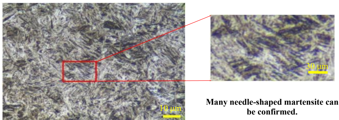
Fig. 3. 21 200 °C tempered nozzle with nital etching (1,000x).
