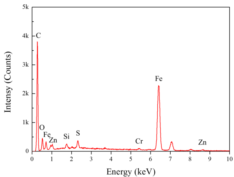
Fig. 4.37 Characteristic EDS-spectra of injector no.2 at the middle of hole.
