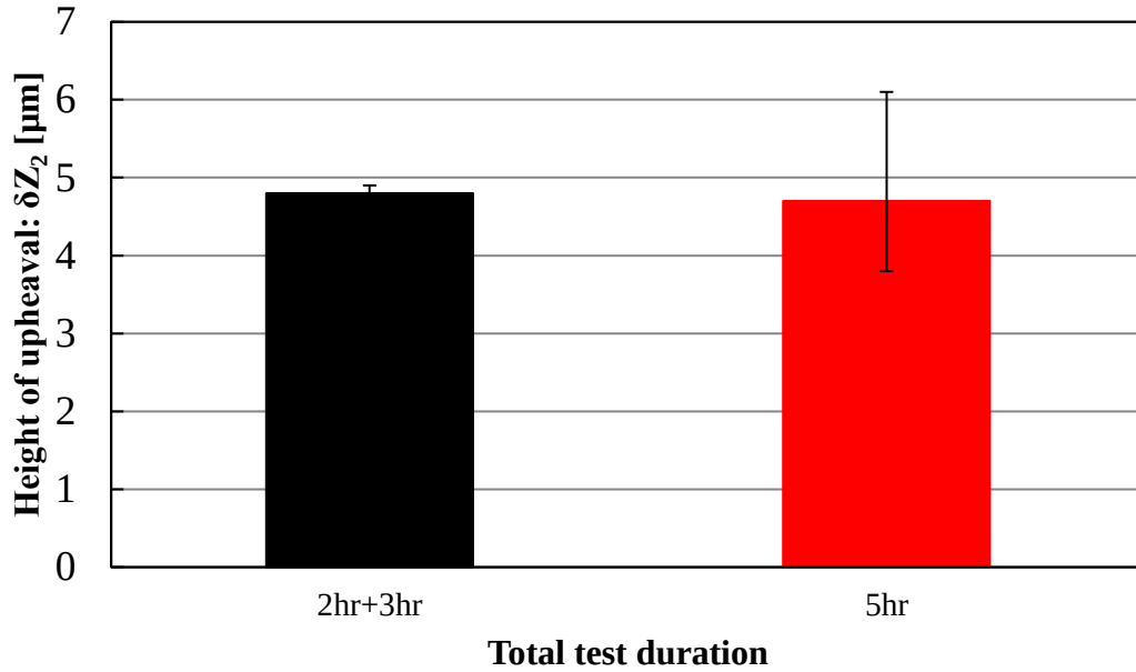
Fig. 3.9 Comparison of deformation between 2-hour heating (2h+3h) and short-term test (5h).
