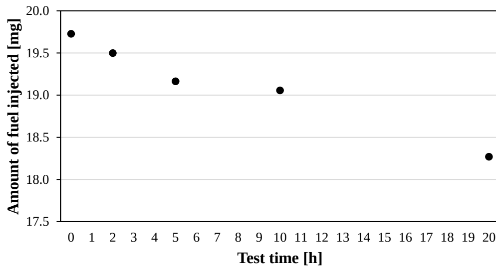
Fig. 4.3 Amount of fuel injected at 480 \mu\text{s} .
