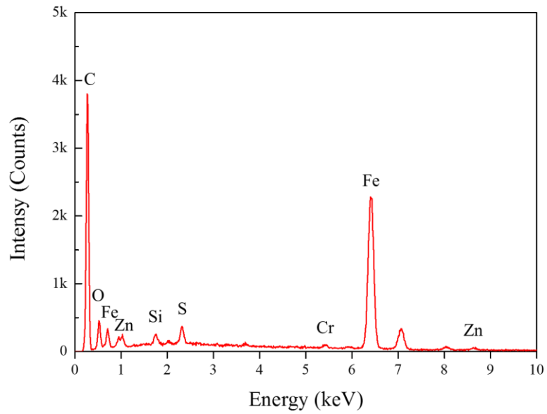
Fig. 4.25 Characteristic EDS-spectra of injector no.5 at the middle of hole.
