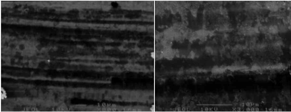
Fig. 2.29 SEM images (800x and 3,000x) of worn surface of body seat in DLC nozzle under 240 °C and Acid 400 μm (100 h).
