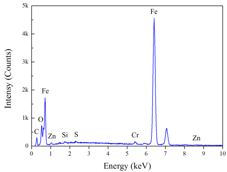
Fig. 4.17 Characteristic EDS-spectra of injector no.2 at the outlet of hole.
