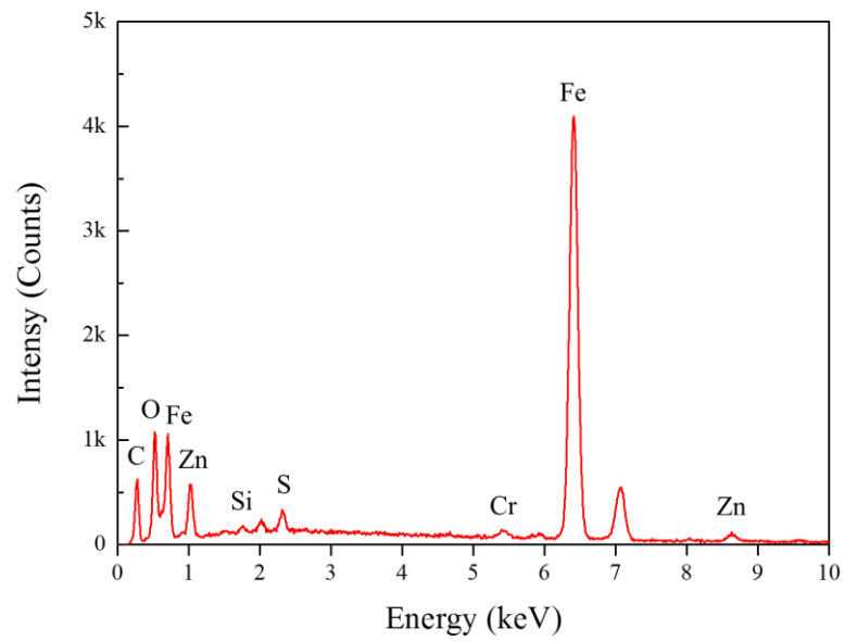
Fig. 4.19 Characteristic EDS-spectra of injector no.3 at the middle of hole.
