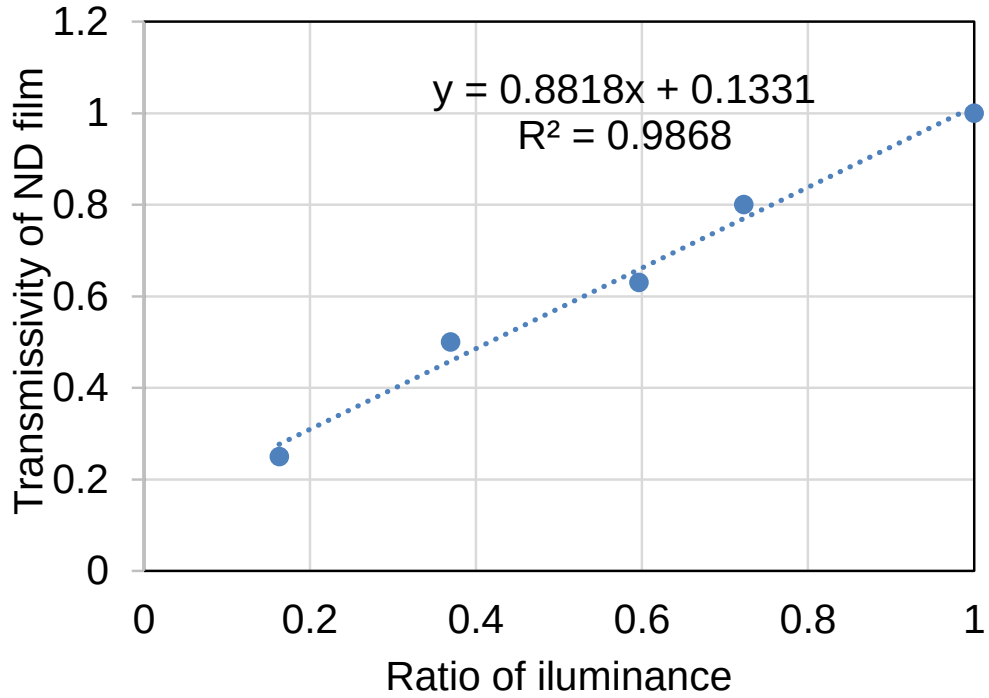
Fig. 2.24 Results of illuminance-transmissivity test.
