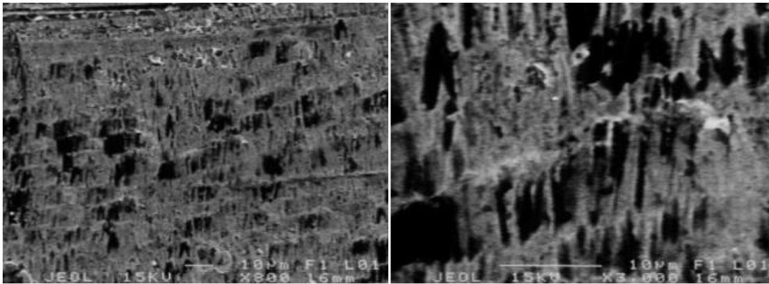
Fig. 2.30 SEM images (800x and 3,000x) of worn surface of body seat in non-DLC nozzle under 240 °C and Acid 400 μm (50 h).
