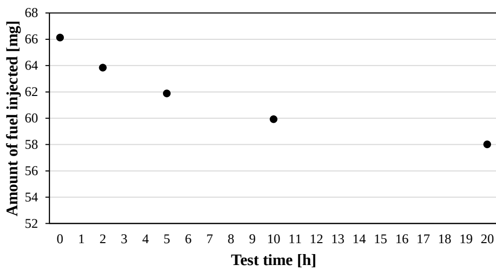
Fig. 4.6 Amount of fuel injected at 1,000 \mu s.
