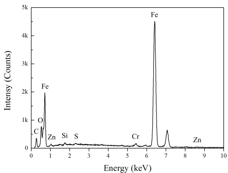
Fig. 4.15 Characteristic EDS-spectra of injector no.2 at the inlet of hole.
