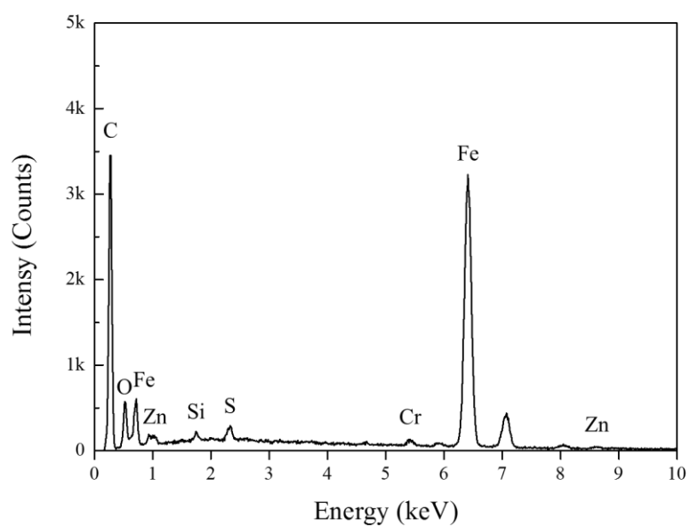
Fig. 4.36 Characteristic EDS-spectra of injector no.2 at the inlet of hole.
